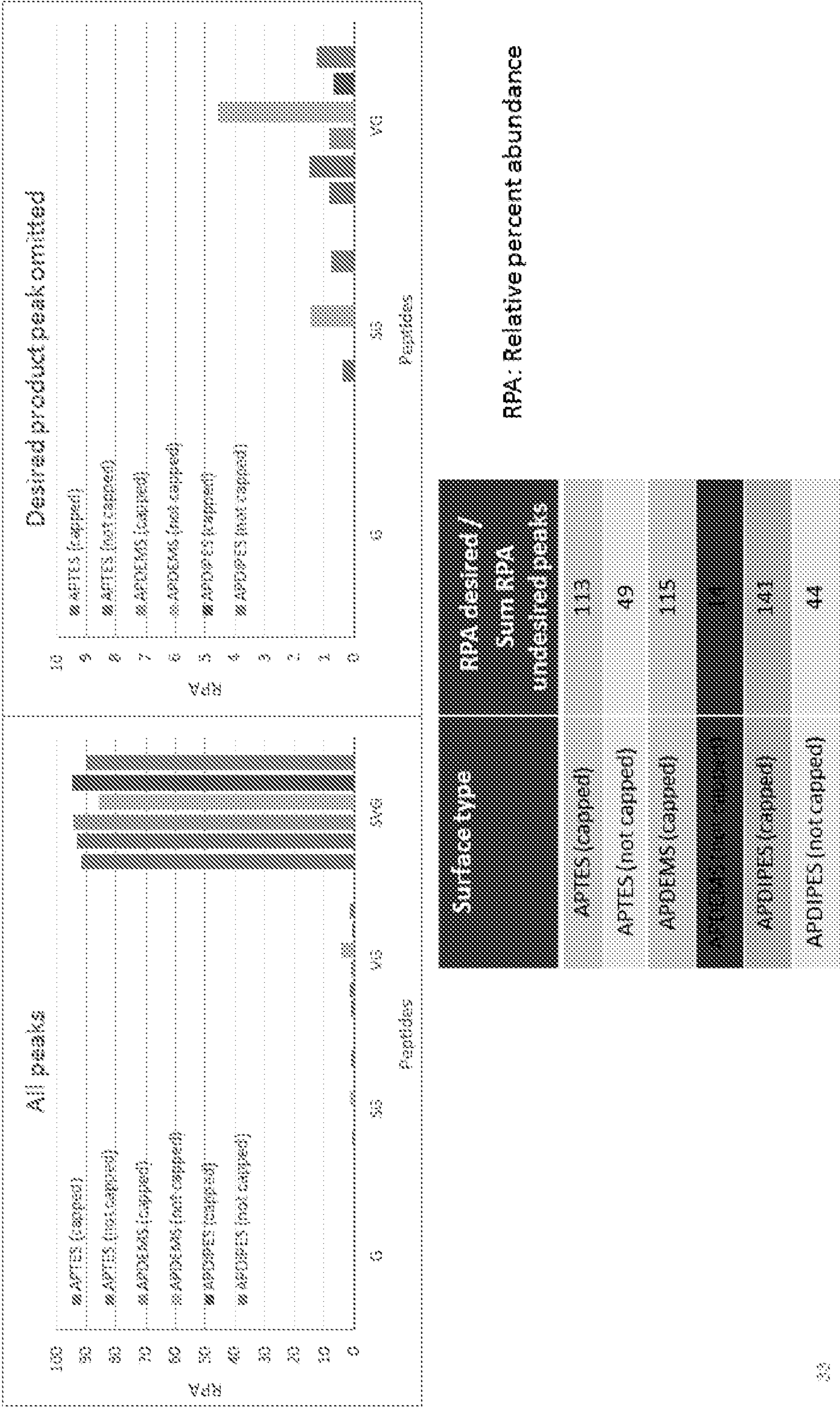
FIG. 34 SVG Synthesis – Capped APDIPES Surface Produces Highest Percentage of Pure Probes
