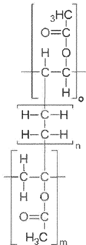
Formula (II)
