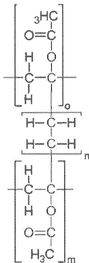
Formula (III)
