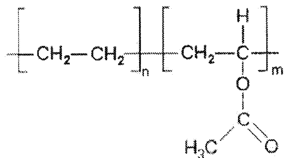
Formula (IV)
