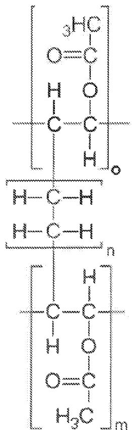
Formula (I)
