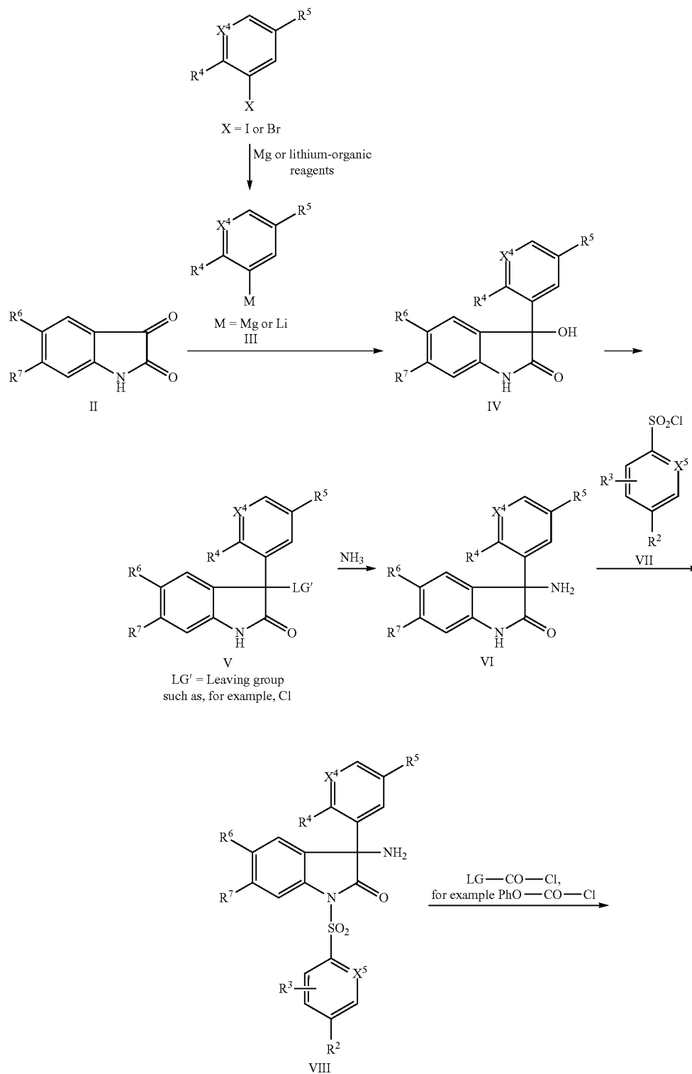
SYNTHESIS SCHEME 1
