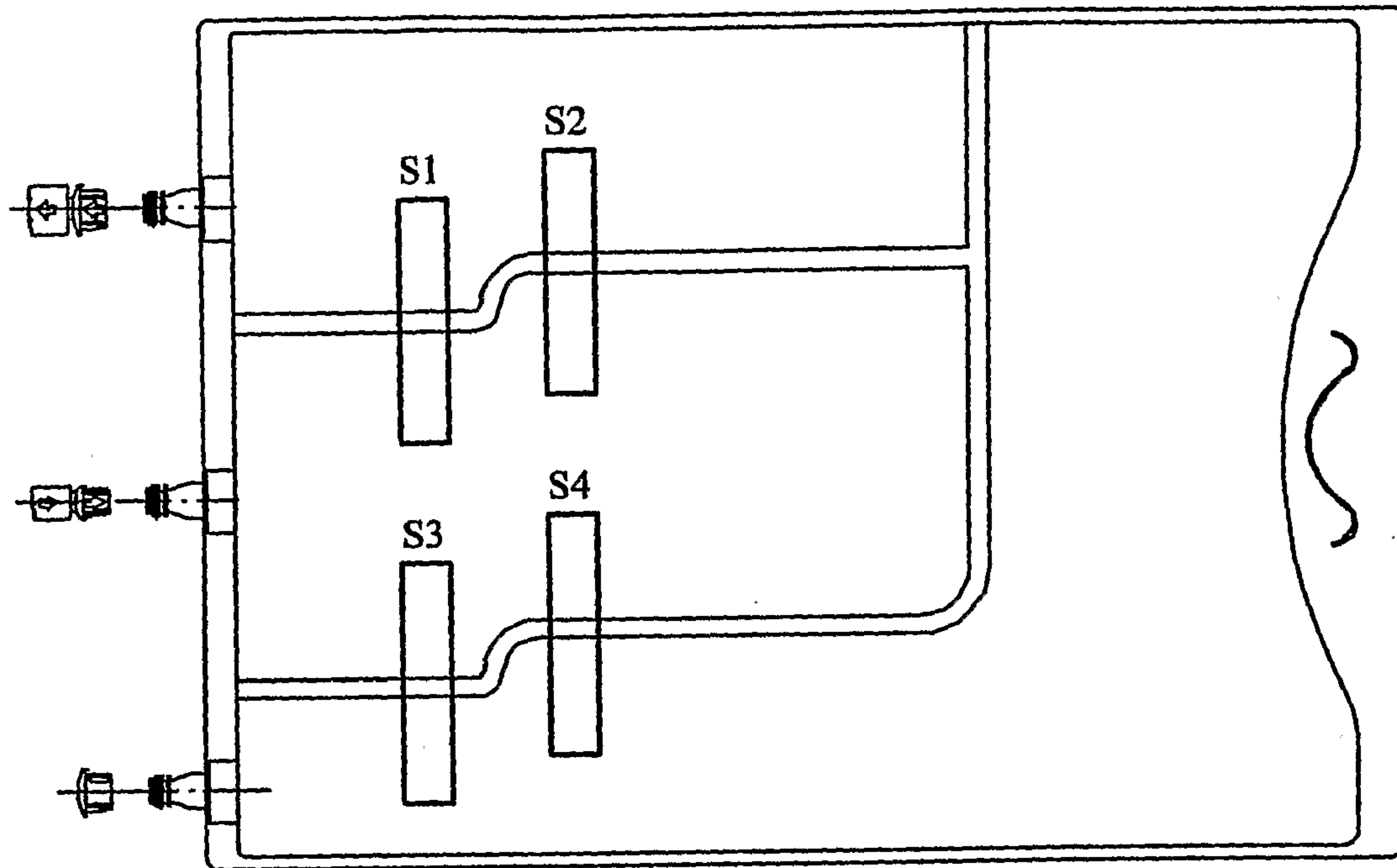
Figure 10: Illustration of sampling for tensile testing (Example)
