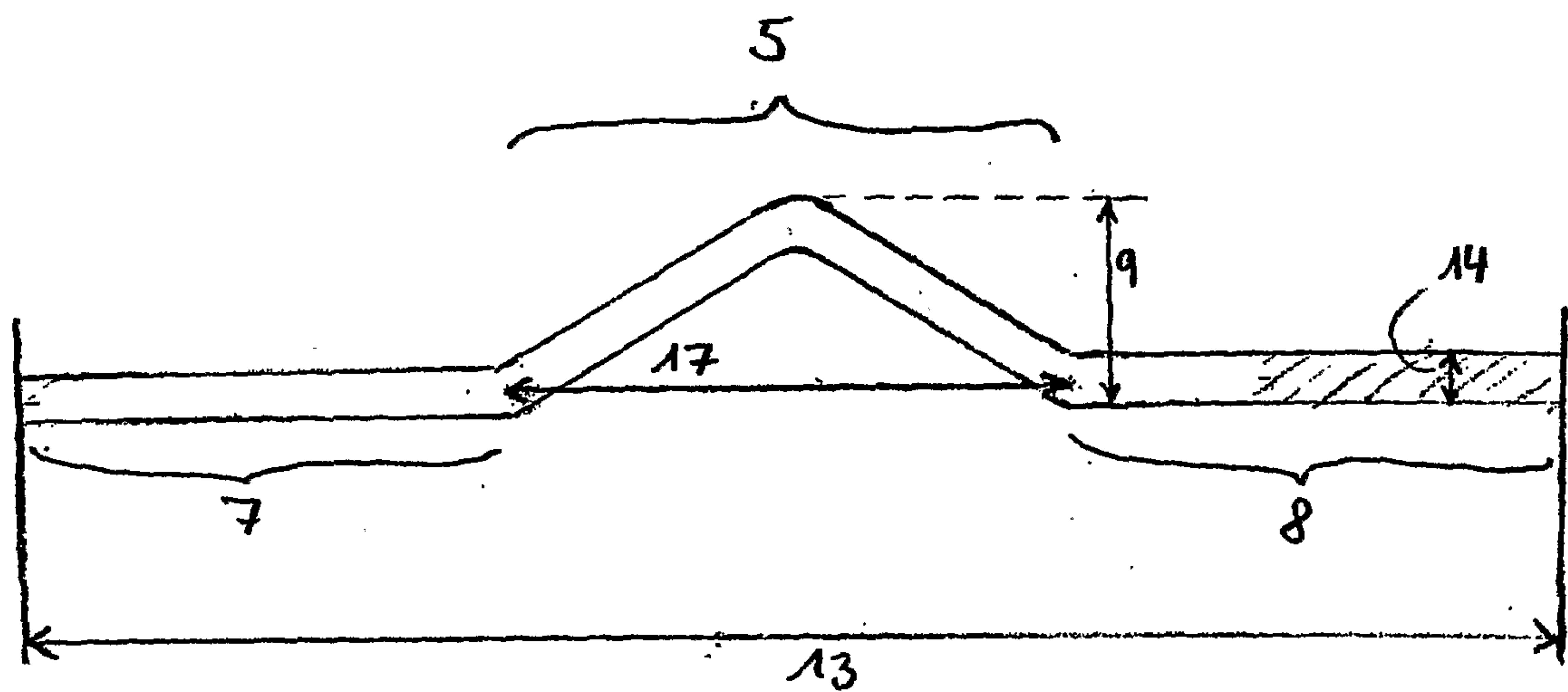
Figure 5: V-type peelable seal (seal type B)
