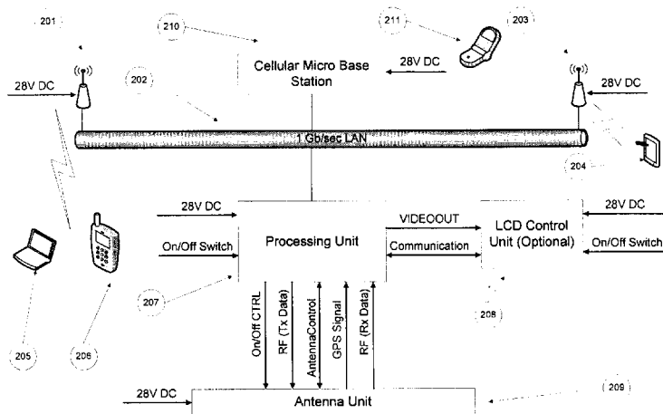
Figure 2 – Moving Segment System Description
