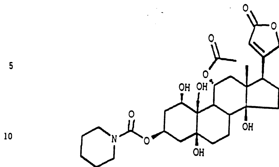
15 3β-[(1'-piperidiny)-carbonyloxy]-11-O-acetyl-ouabaigenine
