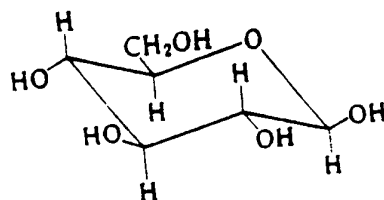
"chair"
