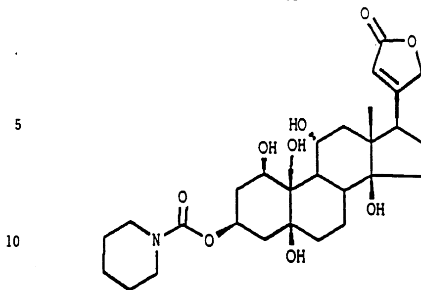
3β-O-(piperidinoformyl)-ouabaigenine
