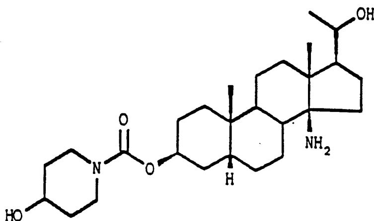
14β-amino-3β-[(4'-hydroxy-1'-piperidinyloxy)-carbonyloxy]- 20α-hydroxy-pregnane
