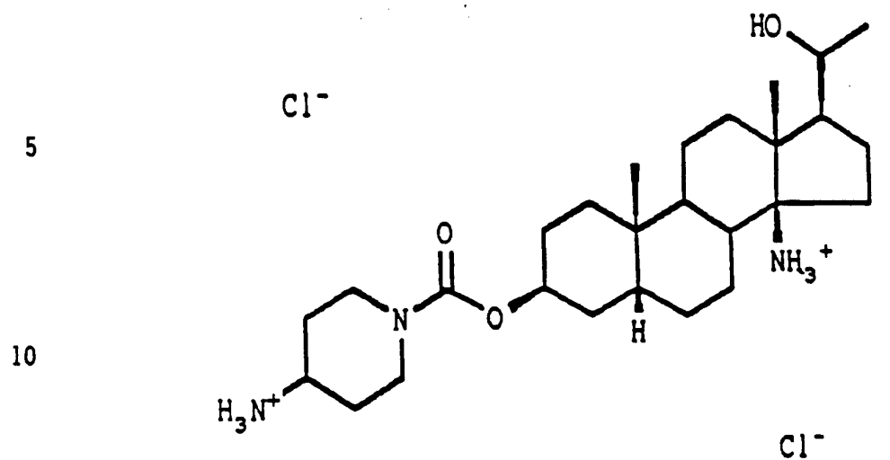
15 14β-amino-3β-[(4'-hydroxy-1'-piperidiny)-carbonyloxy]-20β-hydroxy-pregnane, dihydrochloride
