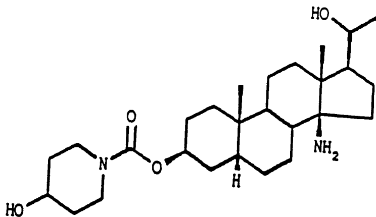
14β-amino-3β-[(4'-hydroxy-1'-piperidinyloxy)-carbonyloxy]- 20β-hydroxy-pregnane
