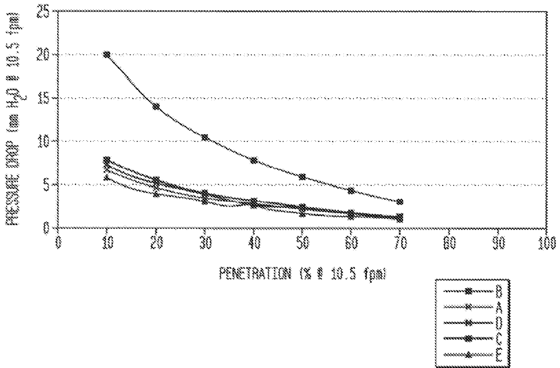
DISCHARGED DOP PENETRATION VERSUS PRESSURE DROP
