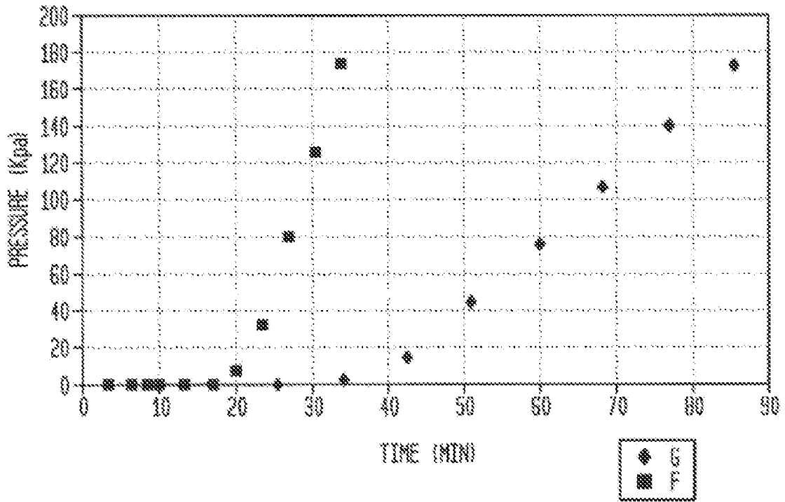
MULTI-PASS TEST PRESSURE CHART
