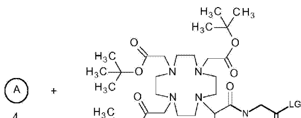
Scheme 12
