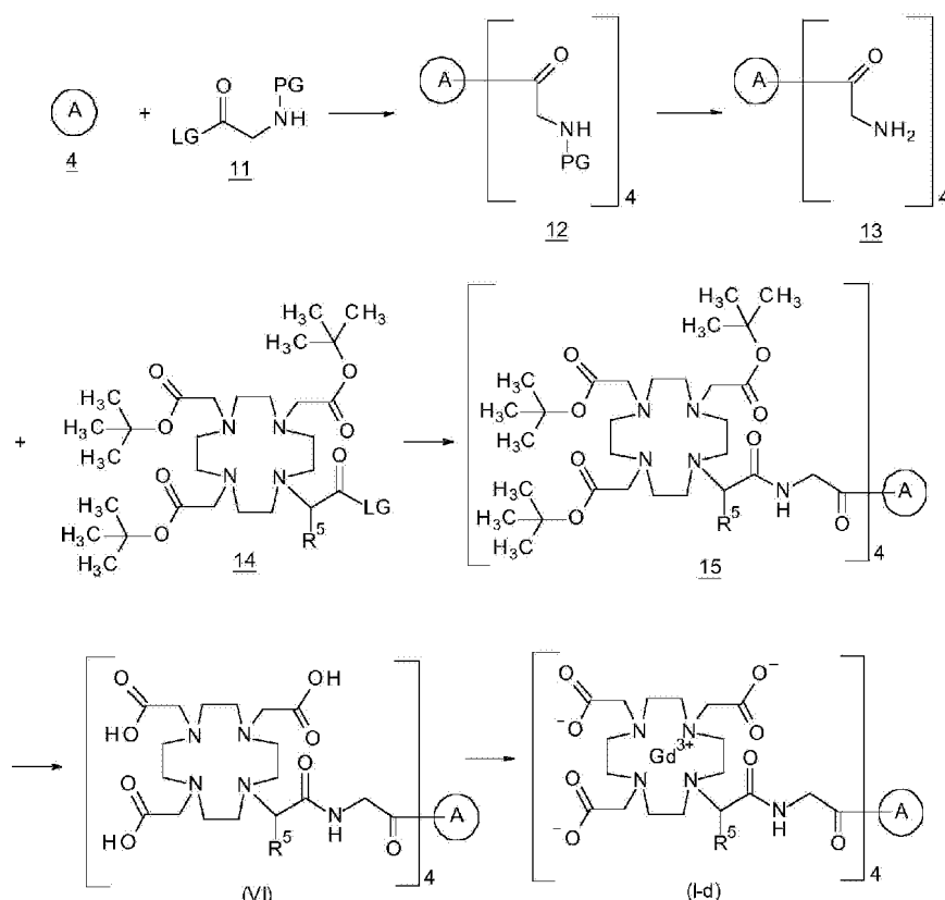
Scheme 11
