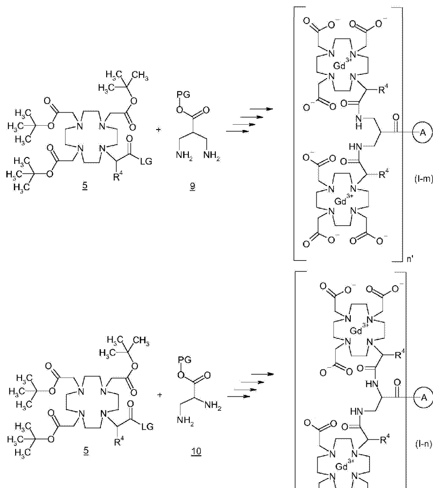
Scheme 10
