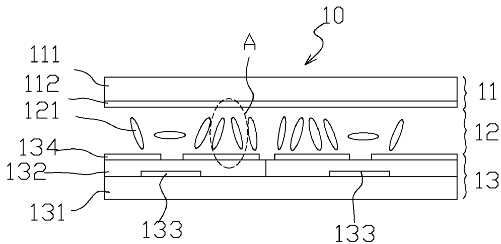
FIG. 1 (Background Art)
