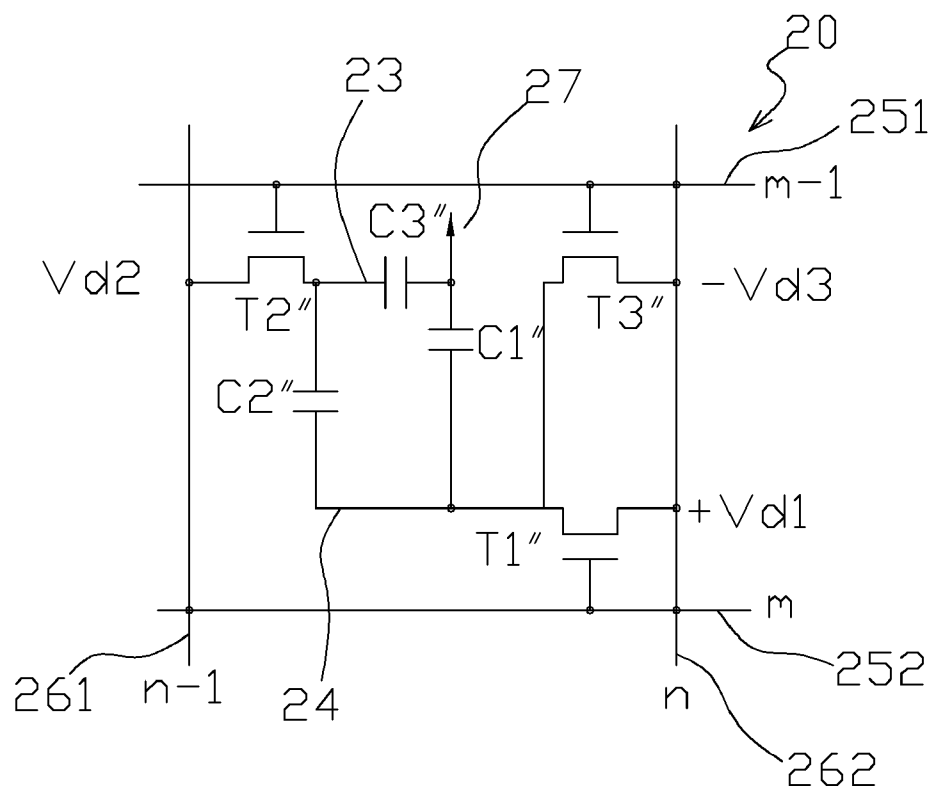
FIG. 2 (Background Art)
