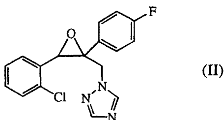
epoxiconazole
