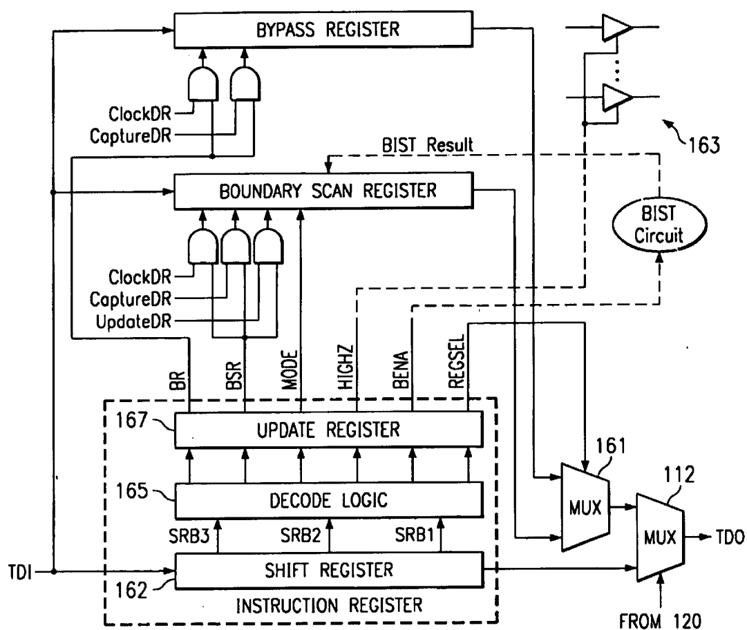
FIG. 16 (PRIOR ART)
