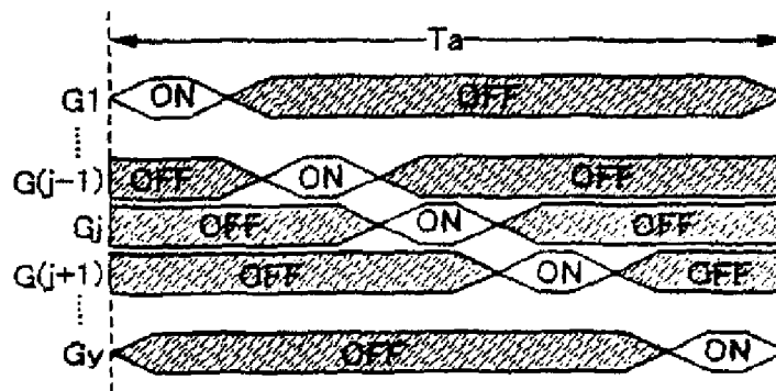
FIG. 3A WRITING PERIOD T_a
