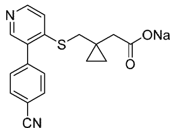
(Compound 1-Na).
