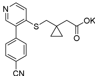
(Compound 1-K).
