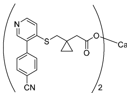
(Compound 1-Ca).
