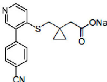
(Compound 1-Na),
