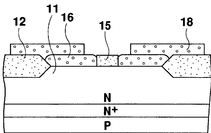
Fig. 1C PRIOR ART
