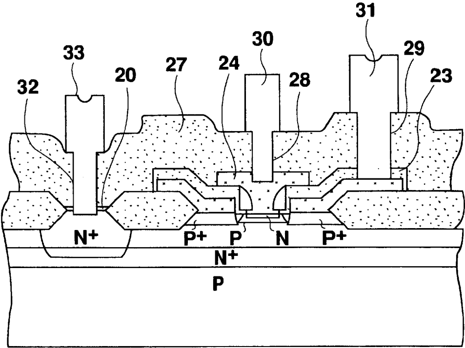
Fig. 2 PRIOR ART
