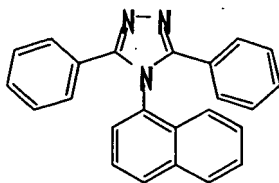
2-(4-tert-butylphenyl)-5-(4-biphenyl)-1,3,4-oxadiazole
