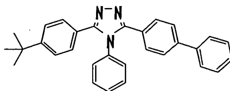
3-(4-tert-butylphenyl)-4-phenyl-5-(4'-biphenyl)-1,2,4-triazole
