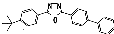
2-(4-tert-butylphenyl)-5-(4-biphenyl)-1,3,4-oxadiazole
