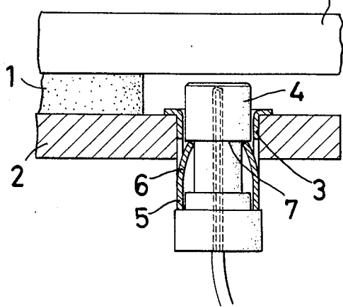
FIG. 1 PRIOR ART 8
