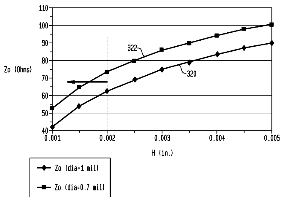
FIG. 3D IMPEDANCE VS. WIRE DISTANCE FROM GROUND
