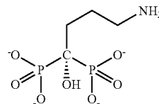
Alendronate
