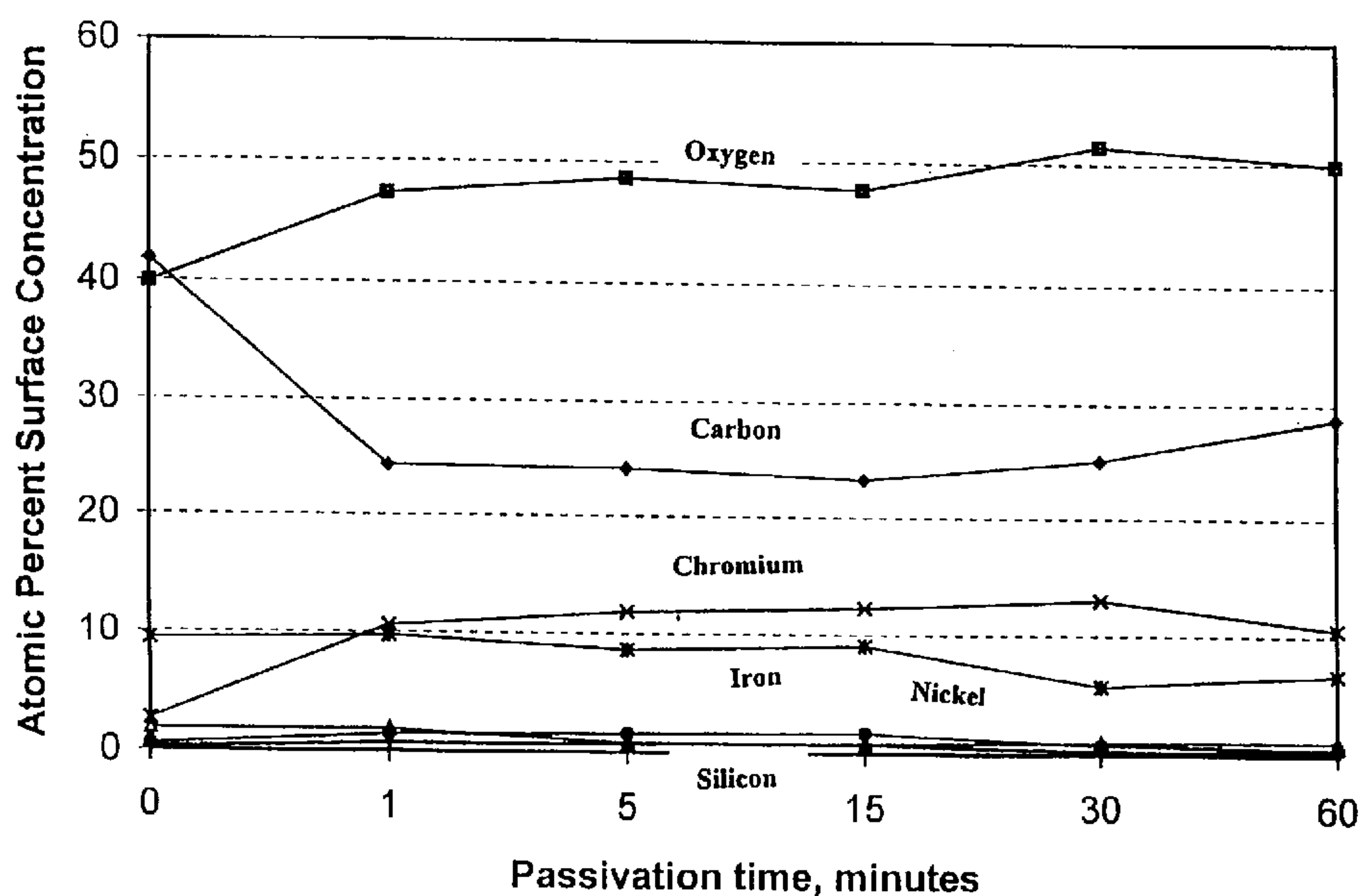
Change in Surface Composition as a Function of Passivation Time, Expanded Scale
