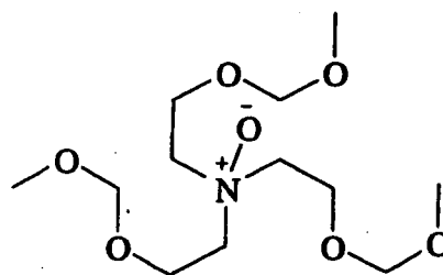
Base-1
