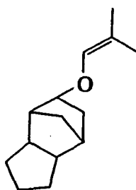
8-(2'-methyl-1'-propenyloxy)tricyclo[5.2.1.0 2,6 ]decane
