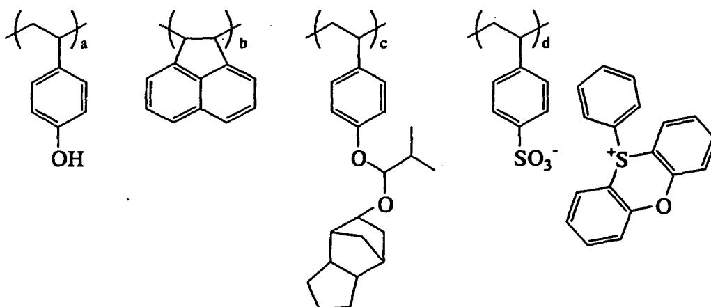
Polymer 34
