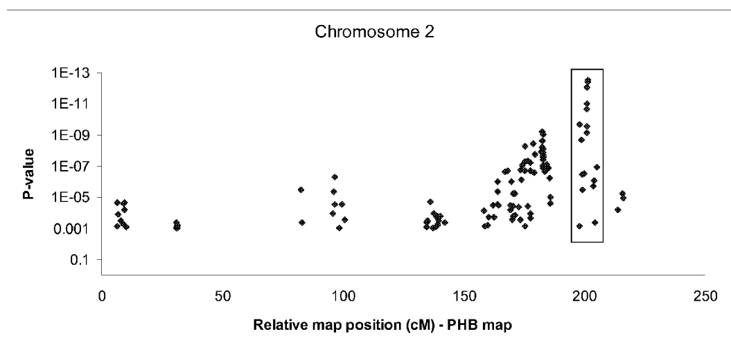
FIG. 2: Associations between marker loci on chromosome 2 and northern leaf blight resistance in a stiff stalk subpopulation at p \leq 0.001 . The lines used in the association analysis had phenotypic scores of 1 and 9.
