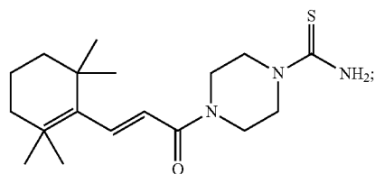
(E)-4-(3-(2,2,6,6-Tetramethylcyclohex-1-en-1-yl)acryloyl)piperazine-1-carbothioamide
