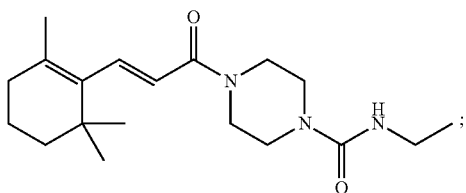
(E)-N-Methyl-4-(3-(2,6,6-trimethylcyclohex-1-enyl)acryloyl)piperazine-1-carboxamide
