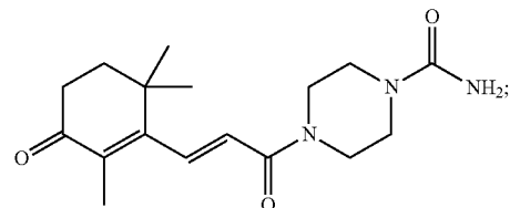
(E)-4-(3-(2,6,6-Trimethyl-3-oxocyclohex-1-en-1-yl)acryloyl)piperazine-1-carboxamide
