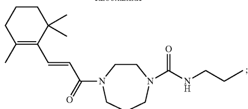
(E)-N-Propyl-4-(3-(2,6,6-trimethylcyclohex-1-en-1-yl)acryloyl)-1,4-diazepane-1-carboxamide
