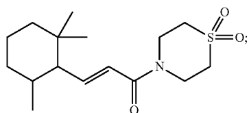
(E)-1-(1,1-Dioxidothiomorpholino)-3-(2,6,6-trimethylcyclohex-1-yl)prop-2-en-1-one
