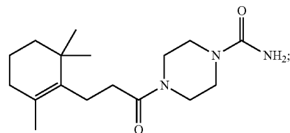
4-(3-(2,6,6-Trimethylcyclohex-1-enyl)propanoyl)piperazine-1-carboxamide
