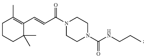
(E)-N-Propyl-4-(3-(2,6,6-trimethylcyclohex-1-enyl)acryloyl)piperazine-1-carboxamide
