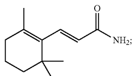
(E)-3-(2,6,6-trimethylcyclohex-1-en-1-yl)acrylamide
