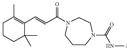
(E)-N-Methyl-4-(3-(2,6,6-trimethylcyclohex-1-en-1-yl)acryloyl)-1,4-diazepane-1-carboxamide
