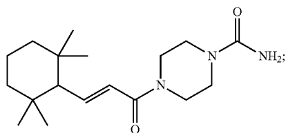
(E)-4-(3-(2,2,6,6-Tetramethylcyclohexyl)acryloyl)piperazine-1-carboxamide
