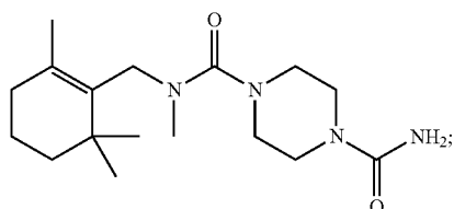
N1-Methyl-N1-((2,6,6-trimethylcyclohex-1-en-1-yl)methyl)piperazine-1,4-dicarboxamide
