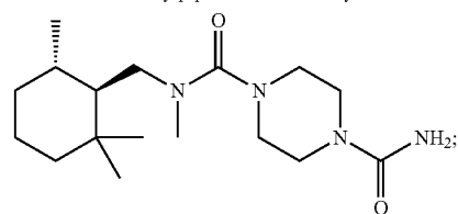
(-)-N1-Methyl-N1-(((1R,6S)-2,2,6-trimethylcyclohexyl)methyl)piperazine-1,4-dicarboxamide
