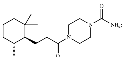
4-(3-((1S,6R)-2,2,6-trimethylcyclohexyl)propanoyl)piperazine-1-carboxamide
