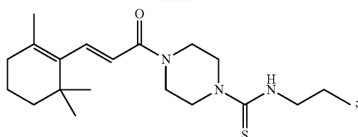
(E)-N-Propyl-4-(3-(2,6,6-trimethylcyclohex-1-enyl)acryloyl)piperazine-1-carbothioamide
