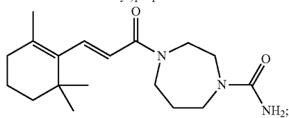
(E)-4-(3-(2,6,6-Trimethylcyclohex-1-en-1-yl)acryloyl)-1,4-diazepane-1-carboxamide
