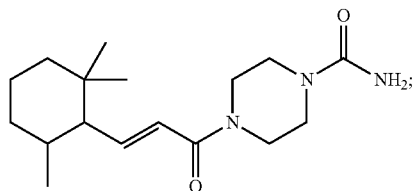
4-((E)-3-((1,6-anti)-2,2,6-trimethylcyclohexyl)acryloyl)piperazine-1-carboxamide
