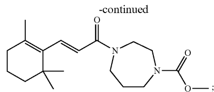
(E)-Methyl-4-(3-(2,6,6-trimethylcyclohex-1-en-1-yl)acryloyl)-1,4-diazepane-1-carboxylate
