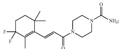
(E)-4-(3-(3,3-Difluoro-2,6,6-trimethylcyclohex-1-en-1-yl)acryloyl)piperazine-1-carboxamide
