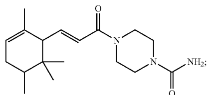
(E)-4-(3-(2,5,6,6-tetramethylcyclohex-2-en-1-yl)acryloyl)piperazine-1-carboxamide
