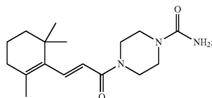
(E)-4-(3-(2,6,6-Trimethylcyclohex-1-enyl)acryloyl)piperazine-1-carboxamide
