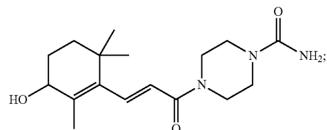
(E)-4-(3-(3-hydroxy-2,6,6-trimethylcyclohex-1-en-1-yl)acryloyl)piperazine-1-carboxamide
