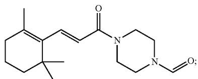
(E)-4-(3-(2,6,6-Trimethylcyclohex-1-en-1-yl)acryloyl)piperazine-1-carbaldehyde
