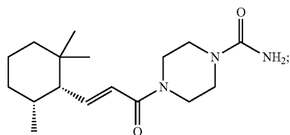
4-((E)-3-((1S,6R)-2,2,6-trimethylcyclohexyl)acryloyl)piperazine-1-carboxamide
