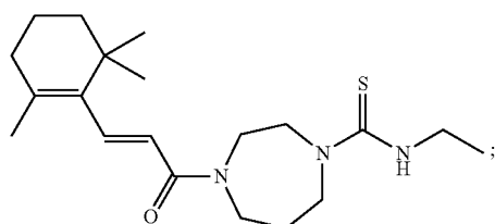
(E)-N-Ethyl-4-(3-(2,6,6-trimethylcyclohex-1-enyl)acryloyl)-1,4-diazepane-1-carbothioamide
