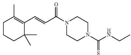
(E)-N-Ethyl-4-(3-(2,6,6-trimethylcyclohex-1-enyl)acryloyl)piperazine-1-carbothioamide
