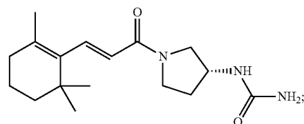
(R,E)-1-(1-(3-(2,6,6-Trimethylcyclohex-1-en-1-yl)acryloyl)pyrrolidin-3-yl)urea
