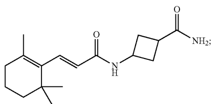
(E)-3-(3-(2,6,6-Trimethylcyclohex-1-en-1-yl)acrylamido)azetidine-1-carboxamide
