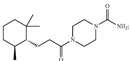
4-(3-((1R,6S)-2,2,6-trimethylcyclohexyl)propanoyl)piperazine-1-carboxamide
