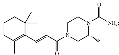
(R,E)-2-Methyl-4-(3-(2,6,6-trimethylcyclohex-1-enyl)acryloyl)piperazine-1-carboxamide
