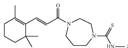
(E)-N-Methyl-4-(3-(2,6,6-trimethylcyclohex-1-en-1-yl)acryloyl)-1,4-diazepane-1-carbothioamide
