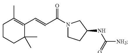
(S,E)-1-(1-(3-(2,6,6-Trimethylcyclohex-1-en-1-yl)acryloyl)pyrrolidin-3-yl)urea
