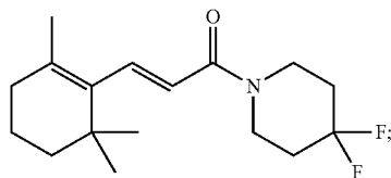
(E)-1-(4,4-Difluoropiperidin-1-yl)-3-(2,6,6-trimethylcyclohex-1-en-1-yl)prop-2-en-1-one
