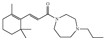
(E)-1-(4-propyl-1,4-diazepan-1-yl)-3-(2,6,6-trimethylcyclohex-1-en-1-yl)prop-2-en-1-one
