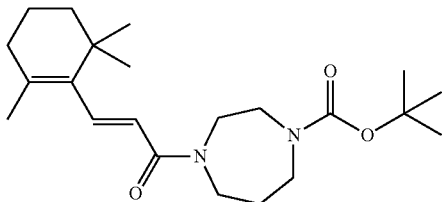
(E)-tert-Butyl 4-(3-(2,6,6-trimethylcyclohex-1-en-1-yl)acryloyl)-1,4-diazepane-1-carboxylate
