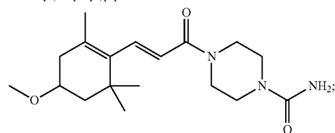
(E)-4-(3-(4-Methoxy-2,6,6-trimethylcyclohex-1-en-1-yl)acryloyl)piperazine-1-carboxamide
