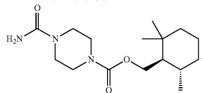
(-)-((1R,6S)-2,2,6-trimethylcyclohexyl)methyl-4-carbamoylpiperazine-1-carboxylate
