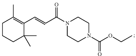
(E)-Ethyl 4-(3-(2,6,6-trimethylcyclohex-1-enyl)acryloyl)piperazine-1-carboxylate
