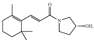
(R,E)-1-(3-Hydroxypyrrolidin-1-yl)-3-(2,6,6-trimethylcyclohex-1-en-1-yl)prop-2-en-1-one
