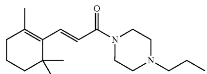
(E)-1-(4-Propylpiperazin-1-yl)-3-(2,6,6-trimethylcyclohex-1-enyl)prop-2-en-1-one
