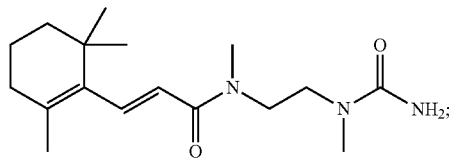
(E)-N-Methyl-N-(2-(1-methylureido)ethyl)-3-(2,6,6-trimethylcyclohex-1-en-1-yl)acrylamide
