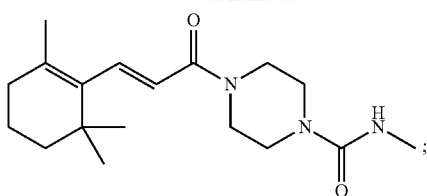
(E)-N-Methyl-4-(3-(2,6,6-trimethylcyclohex-1-enyl)acryloyl)piperazine-1-carboxamide
