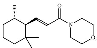
(E)-1-Morpholino-3-((1S,6S)-2,2,6-trimethylcyclohexyl)prop-2-en-1-one
