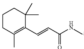
(E)-N-Methyl-3-(2,6,6-trimethylcyclohex-1-en-1-yl)acrylamide
