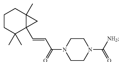
(E)-4-(3-(2,2,6-trimethylbicyclo[4.1.0]heptan-1-yl)acryloyl)piperazine-1-carboxamide
