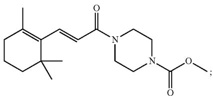
(E)-Methyl 4-(3-(2,6,6-trimethylcyclohex-1-enyl)acryloyl)piperazine-1-carboxylate
