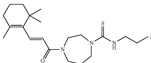
(E)-N-Propyl-4-(3-(2,6,6-trimethylcyclohex-1-enyl)acryloyl)-1,4-diazepane-1-carbothioamide
