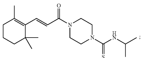
(E)-N-Isopropyl-4-(3-(2,6,6-trimethylcyclohex-1-enyl)acryloyl)piperazine-1-carbothioamide
