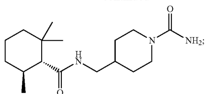
4-(((1R,6S)-2,2,6-trimethylcyclohexanecarboxamido)methyl)piperidine-1-carboxamide
