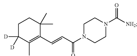
(E)-4-(3-(3,3-Dideutero-2,6,6-trimethylcyclohex-1-en-1-yl)acryloyl)piperazine-1-carboxamide
