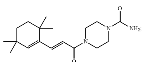
(E)-4-(3-(3,3,6,6-Tetramethylcyclohex-1-enyl)acryloyl)piperazine-1-carboxamide
