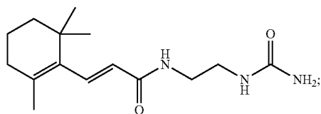
(E)-3-(2,6,6-Trimethylcyclohex-1-en-1-yl)-N-(2-ureidoethyl)acrylamide
