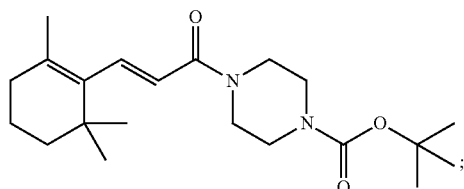
(E)-tert-Butyl 4-(3-(2,6,6-trimethylcyclohex-1-enyl)acryloyl)piperazine-1-carboxylate
