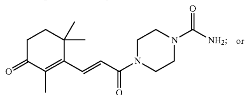
(E)-4-(3-(2,6,6-Trimethyl-3-oxocyclohex-1-en-1-yl)acryloyl)piperazine-1-carboxamide
