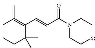
(E)-1-Thiomorpholino-3-(2,6,6-trimethylcyclohex-1-en-1-yl)prop-2-en-1-one
