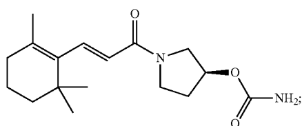
(S,E)-1-(3-(2,6,6-Trimethylcyclohex-1-enyl)acryloyl)pyrrolidin-3-yl carbamate
