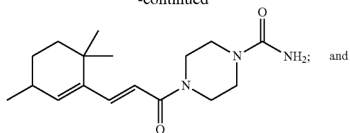
(E)-4-(3-(3,3,6,6-Trimethylcyclohex-1-en-1-yl)acryloyl)piperazine-1-carboxamide
