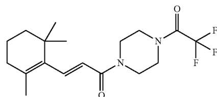
(E)-1-(4-(2,2,2-Trifluoroacetyl)piperazin-1-yl)-3-(2,6,6-trimethylcyclohex-1-enyl)prop-2-en-1-one
