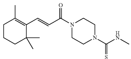
(E)-N-Methyl-4-(3-(2,6,6-trimethylcyclohex-1-enyl)acryloyl)piperazine-1-carbothioamide
