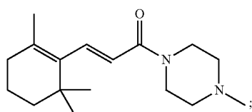
(E)-1-(4-Methylpiperazin-1-yl)-3-(2,6,6-trimethylcyclohex-1-enyl)prop-2-en-1-one
