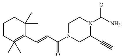
(E)-2-Ethynyl-4-(3-(2,6,6-trimethylcyclohex-1-en-1-yl)acryloyl)piperazine-1-carboxamide
