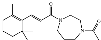
(E)-1-(4-Acetyl-1,4-diazepan-1-yl)-3-(2,6,6-trimethylcyclohex-1-en-1-yl)prop-2-en-1-one
