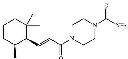
4-((E)-3-((1R,6S)-2,2,6-trimethylcyclohexyl)acryloyl)piperazine-1-carboxamide
