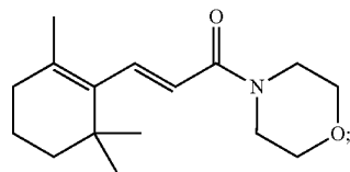
(E)-1-(Morpholino-3-(2,6,6-trimethylcyclohex-1-en-1-yl)prop-2-en-1-one
