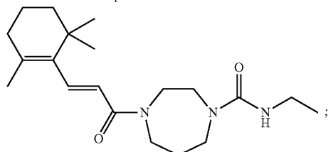
(E)-N-Ethyl-4-(3-(2,6,6-trimethylcyclohex-1-en-1-yl)acryloyl)-1,4-diazepane-1-carboxamide
