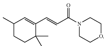
(E)-1-Morpholino-3-(3,6,6-trimethylcyclohex-1-en-1-yl)prop-2-en-1-one
