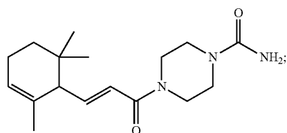
(E)-4-(3-(2,6,6-trimethylcyclohex-2-en-1-yl)acryloyl)piperazine-1-carboxamide
