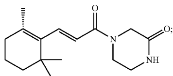
(E)-4-(3-(2,6,6-Trimethylcyclohex-1-en-1-yl)acryloyl)piperazin-2-one
