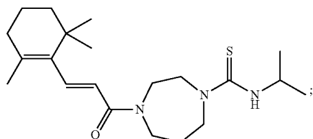
(E)-N-Isopropyl-4-(3-(2,6,6-trimethylcyclohex-1-enyl)acryloyl)-1,4-diazepane-1-carbothioamide
