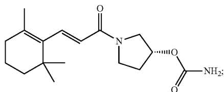
(R,E)-1-(3-(2,6,6-Trimethylcyclohex-1-en-1-yl)acryloyl)pyrrolidin-3-yl carbamate
