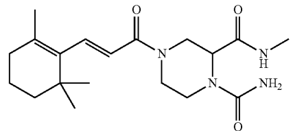
(E)-N2-Methyl-4-(3-(2,6,6-trimethylcyclohex-1-enyl)acryloyl)piperazine-1,2-dicarboxamide
