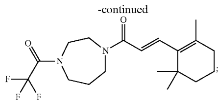
(E)-1-(4-(2,2,2-Trifluoroacetyl)-1,4-diazepan-1-yl)-3-(2,6,6-trimethylcyclohex-1-en-1-yl)prop-2-en-1-one
