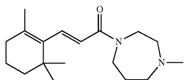
(E)-1-(4-Methyl-1,4-diazepan-1-yl)-3-(2,6,6-trimethylcyclohex-1-en-1-yl)prop-2-en-1-one
