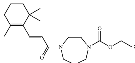
(E)-Ethyl-4-(3-(2,6,6-trimethylcyclohex-1-en-1-yl)acryloyl)-1,4-diazepane-1-carboxylate
