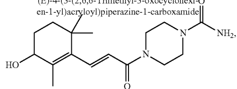
(E)-4-(3-(3-hydroxy-2,6,6-trimethylcyclohex-1-en-1-yl)acryloyl)piperazine-1-carboxamide
