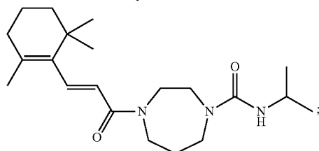
(E)-N-Isopropyl-4-(3-(2,6,6-trimethylcyclohex-1-en-1-yl)acryloyl)-1,4-diazepane-1-carboxamide
