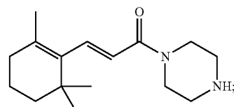
1-(Piperazin-1-yl)-3-(2,6,6-trimethylcyclohex-1-enyl)propan-1-one
