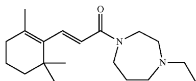
(E)-1-(4-Ethyl-1,4-diazepan-1-yl)-3-(2,6,6-trimethylcyclohex-1-en-1-yl)prop-2-en-1-one
