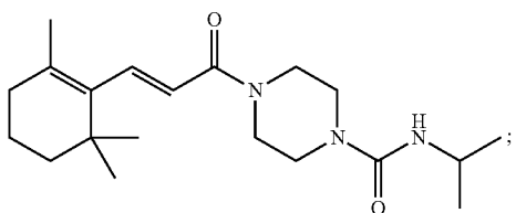
(E)-N-Isopropyl-4-(3-(2,6,6-trimethylcyclohex-1-enyl)acryloyl)piperazine-1-carboxamide
