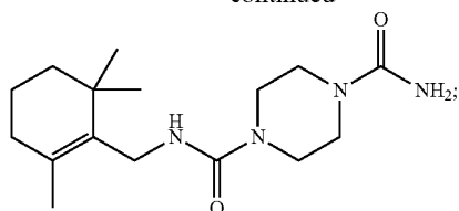
N1-((2,6,6-Trimethylcyclohex-1-en-1-yl)methyl)piperazine-1,4-dicarboxamide
