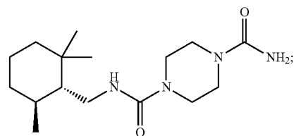
N1-(((1R,6S)-2,2,6-trimethylcyclohexyl)methyl)piperazine-1,4-dicarboxamide
