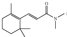
(E)-N,N-Dimethyl-3-(2,6,6-trimethylcyclohex-1-en-1-yl)acrylamide
