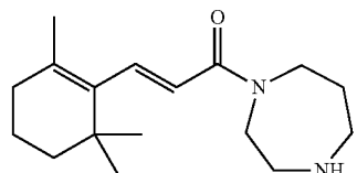
(E)-1-(1,4-Diazepan-1-yl)-3-(2,6,6-trimethylcyclohex-1-en-1-yl)prop-2-en-1-one
