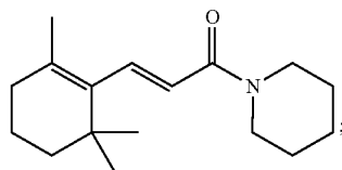
(E)-1-(Piperidin-1-yl)-3-(2,6,6-trimethylcyclohex-1-en-1-yl)prop-2-en-1-one
