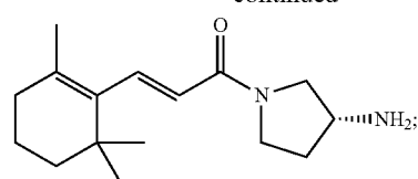
(R,E)-1-(3-Aminopyrrolidin-1-yl)-3-(2,6,6-trimethylcyclohex-1-en-1-yl)prop-2-en-1-one
