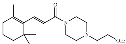
(E)-1-(4-(2-hydroxyethyl)piperazin-1-yl)-3-(2,6,6-trimethylcyclohex-1-en-1-yl)prop-2-en-1-one
