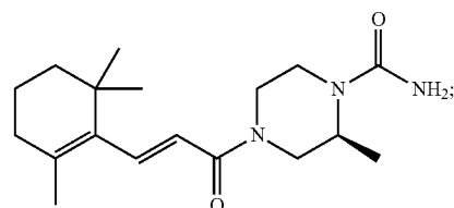
(S,E)-2-Methyl-4-(3-(2,6,6-trimethylcyclohex-1-enyl)acryloyl)piperazine-1-carboxamide
