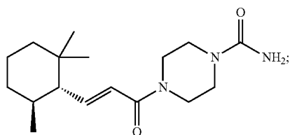
(+)-4-((E)-3-((1S,6S)-2,2,6-trimethylcyclohexyl)acryloyl)piperazine-1-carboxamide
