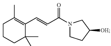
(S,E)-1-(3-Hydroxypyrrolidin-1-yl)-3-(2,6,6-trimethylcyclohex-1-enyl)prop-2-en-1-one
