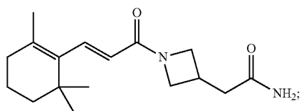
(E)-2-(1-(3-(2,6,6-trimethylcyclohex-1-en-1-yl)acryloyl)azetidin-3-yl)acetamide
