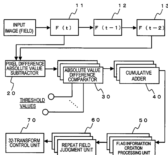
BLOCK DIAGRAM OF DETECTION DEVICE 1
