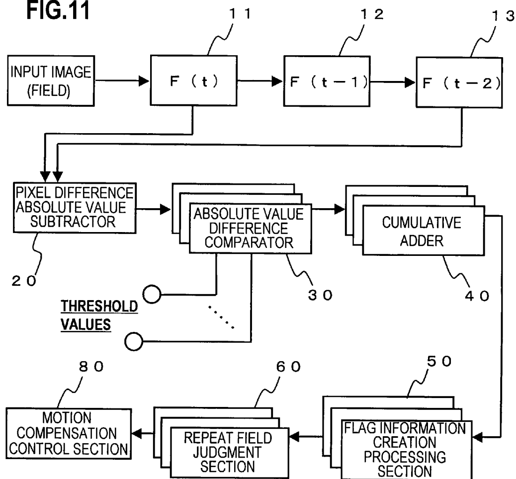
GENERAL BLOCK DIAGRAM OF ANOTHER DETECTION DEVICE 1
