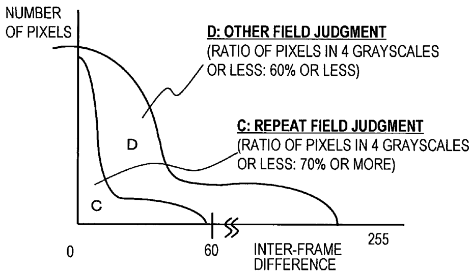
FIG. 4B INTER-FRAME DIFFERENCE DISTRIBUTION WITH NOISE
