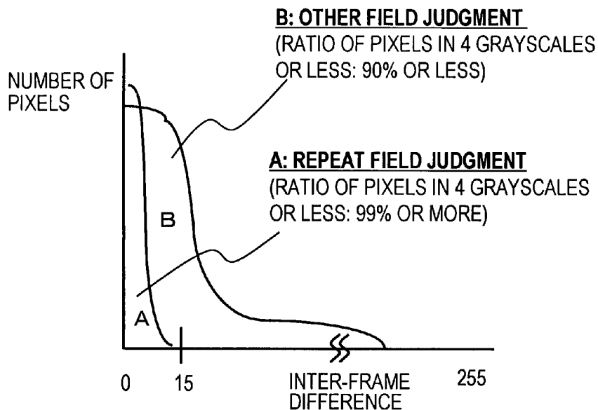
FIG. 4A INTER-FRAME DIFFERENCE DISTRIBUTION WITHOUT NOISE
