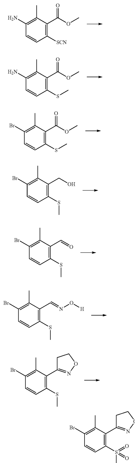
Scheme 3 shows a further possible synthesis route to bromobenzene derivatives of the type of formula X.
