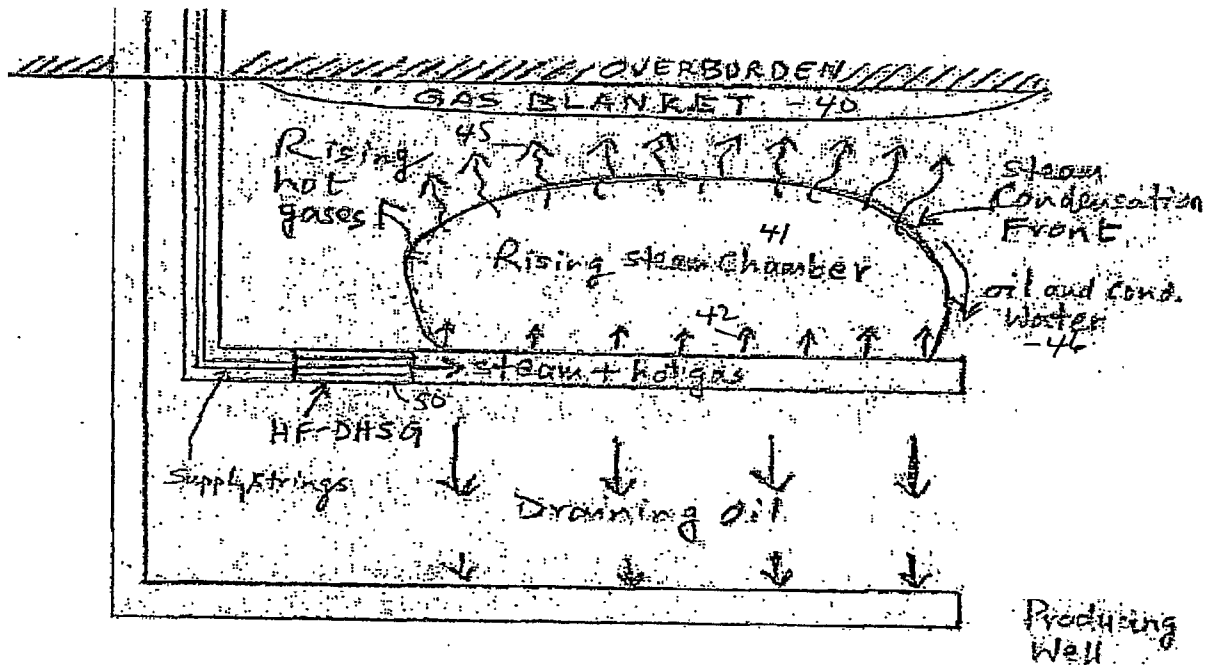
HF-DHSG in conventional SAGD - FIG. 5(a)
