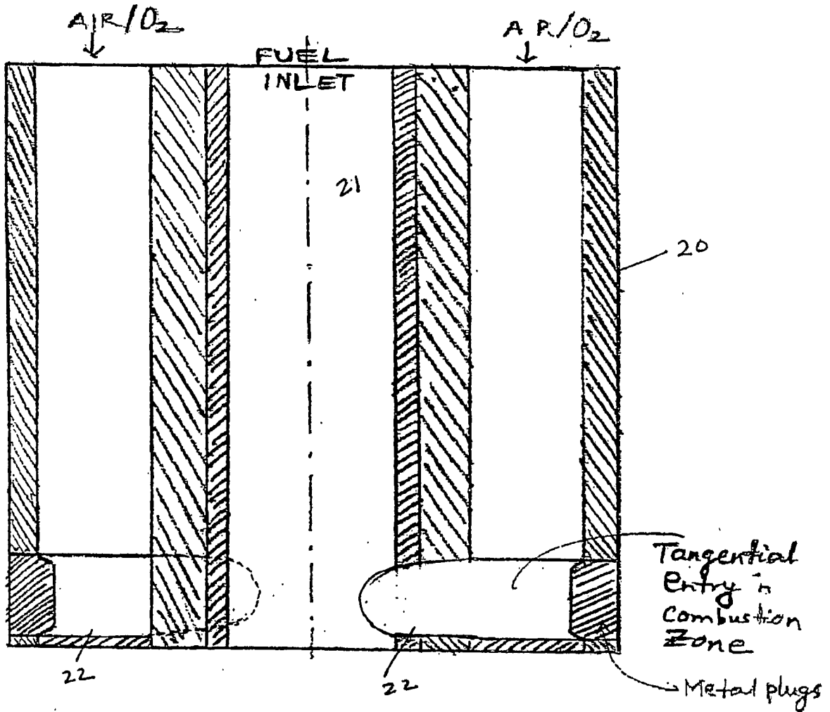
Fig. 3 (a) Design of the Swirl Burner used Steam Generator
