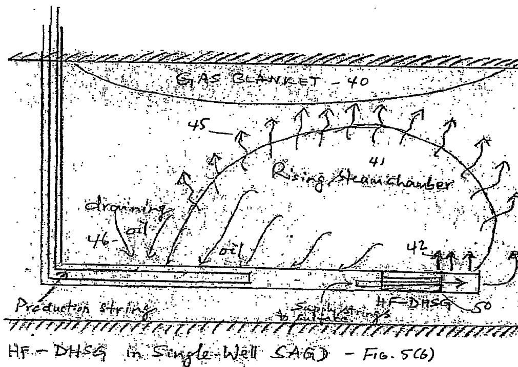
FIG. 5: Application of the Direct Combustion Process in SAGD
