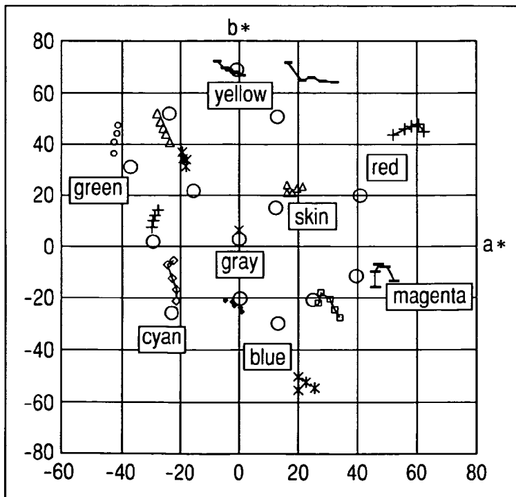
STATES OF COLORS ACHIEVED UNDER MIXED ILLUMINATION OF F6/D65 AFTER CORRECTION
