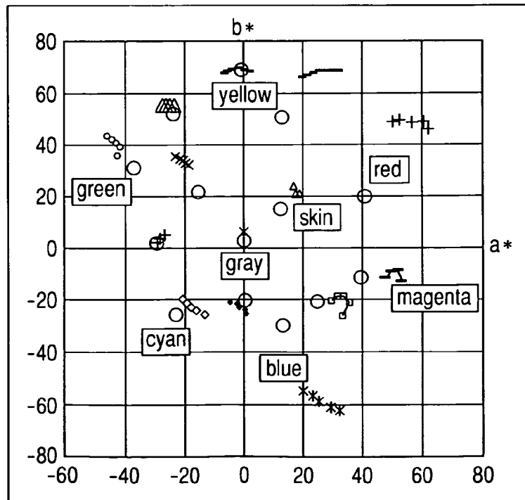
STATES OF COLORS ACHIEVED UNDER MIXED ILLUMINATION OF F12/D65 AFTER CORRECTION
