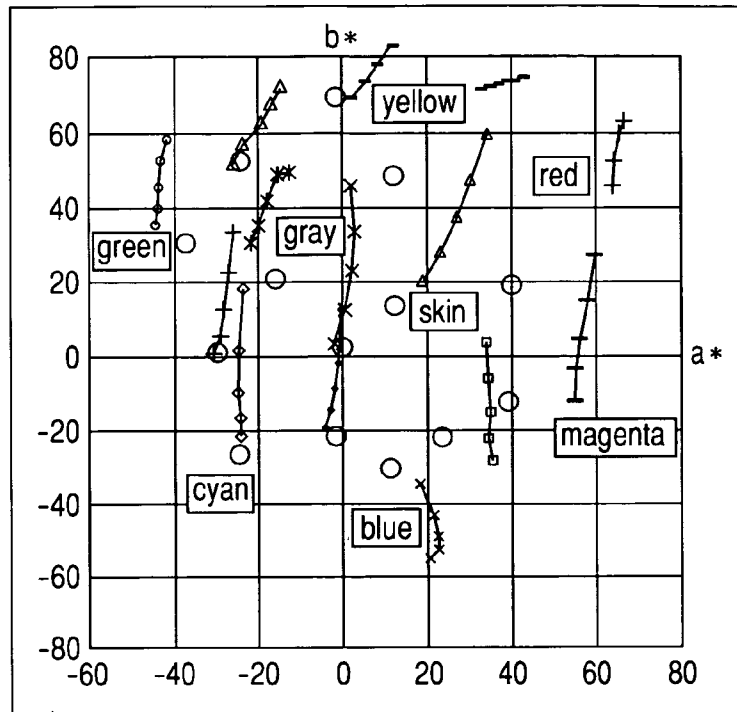
STATES OF COLORS ACHIEVED UNDER MIXED ILLUMINATION OF F12/D50 BEFORE CORRECTION (WB IS BASED ON D50)
