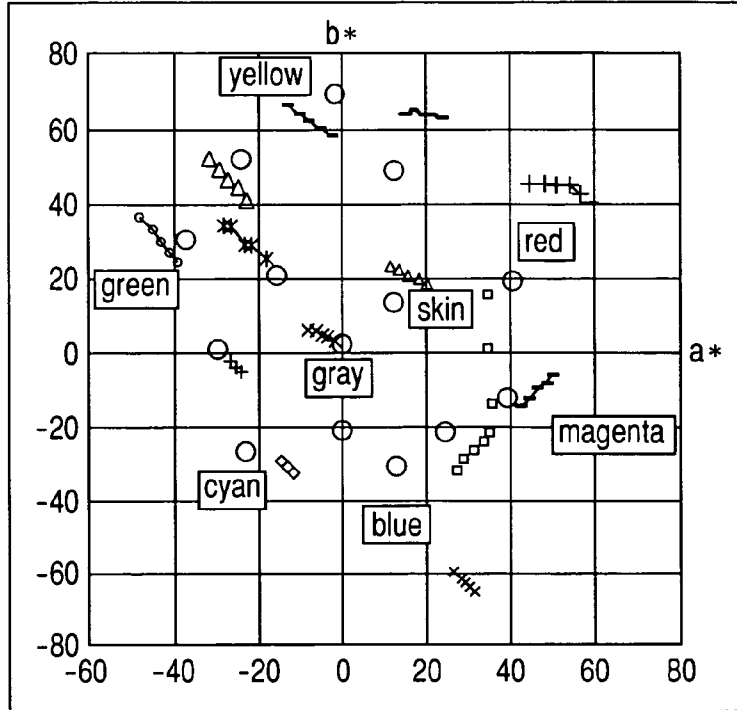
STATES OF COLORS ACHIEVED UNDER MIXED ILLUMINATION OF F12/A LIGHT SOURCE BEFORE CORRECTION (WB IS BASED ON A LIGHT SOURCE)
