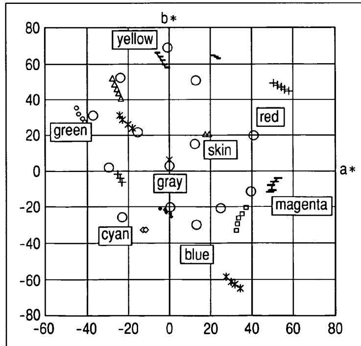
STATES OF COLORS ACHIEVED UNDER MIXED ILLUMINATION OF F12/A LIGHT SOURCE AFTER CORRECTION
