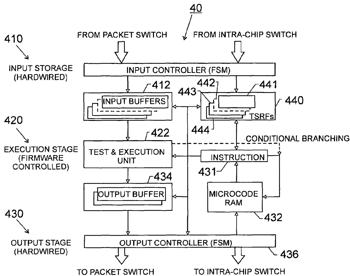
BLOCK DIAGRAM OF A PROTOCOL ENGINE
