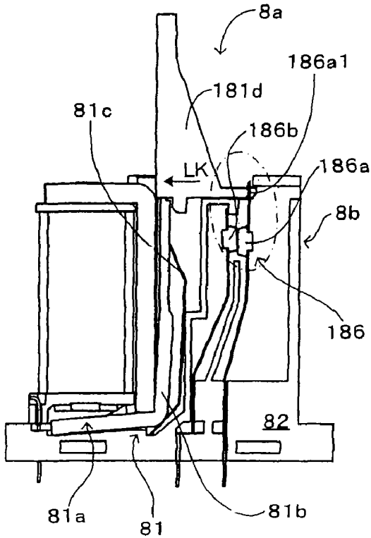
FIG. 8A: NORMALLY-CLOSED SWITCHING CONTACT: LOCK POSITION
