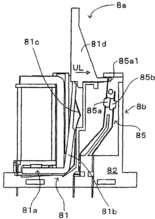
FIG. 5B1: NORMALLY-CLOSED SWITCHING CONTACT: UNLOCK POSITION
