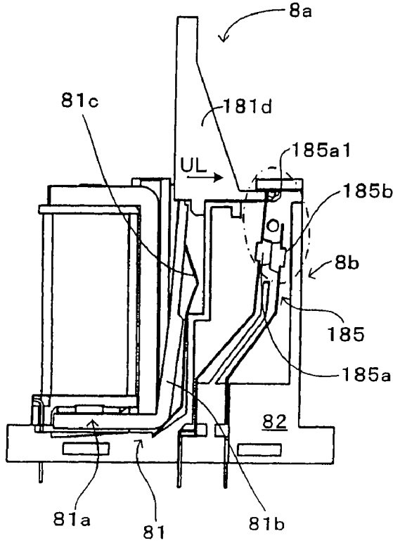
FIG. 10C: NORMALLY-OPEN SWITCHING CONTACT: UNLOCK POSITION (POWER SUPPLY TO ELECTROMAGNET SHUT OFF) (FUSED CONTACT)
