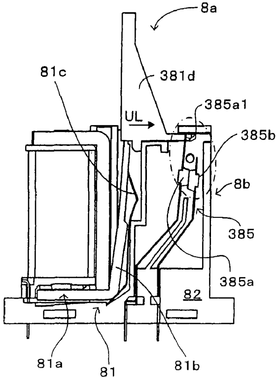
FIG. 11A: NORMALLY-OPEN SWITCHING CONTACT: UNLOCK POSITION
