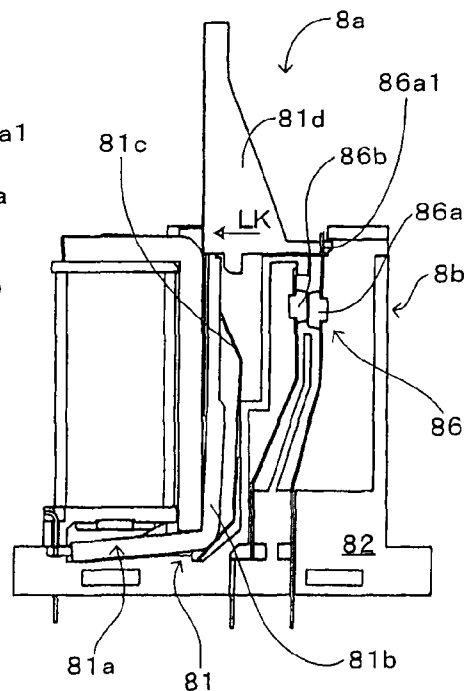
FIG. 5B2: NORMALLY-CLOSED SWITCHING CONTACT: LOCK POSITION
