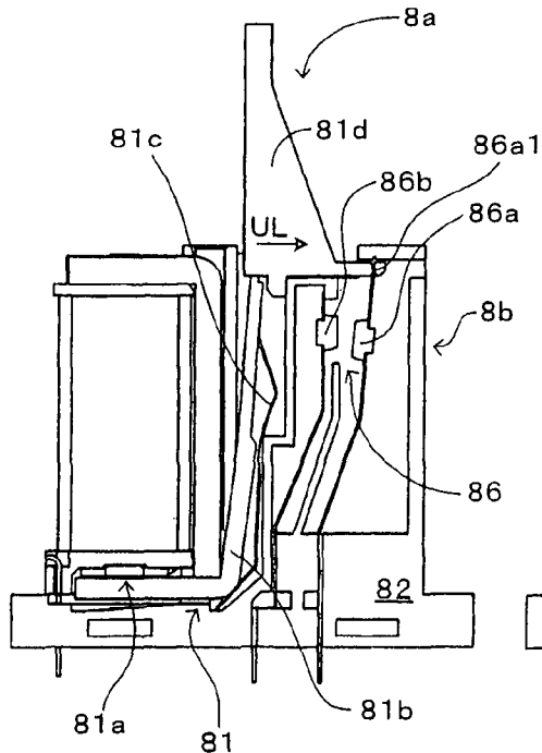
FIG. 5B1: NORMALLY-CLOSED SWITCHING CONTACT: UNLOCK POSITION
