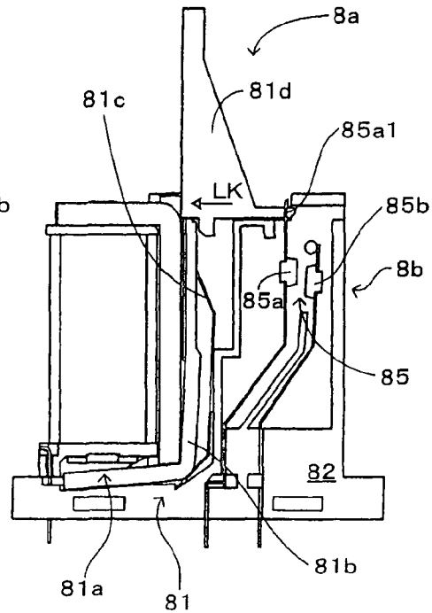
FIG. 5B2: NORMALLY-CLOSED SWITCHING CONTACT: LOCK POSITION
