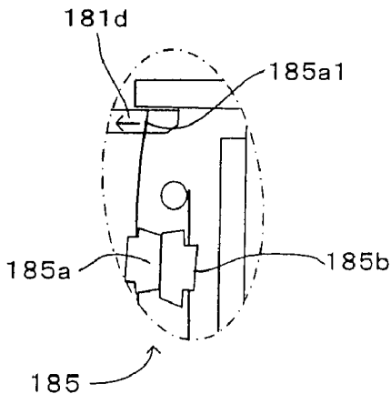
FIG. 10C: NORMALLY-OPEN SWITCHING CONTACT: UNLOCK POSITION (POWER SUPPLY TO ELECTROMAGNET SHUT OFF) (FUSED CONTACT)
