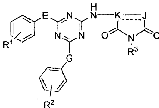
Formel I
