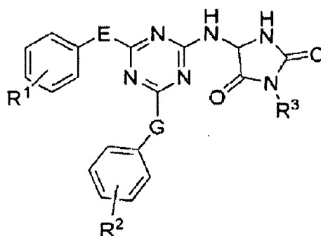
Formel II
