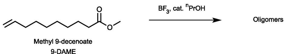
Scheme 1. BF 3 -mediated homo-oligomerization of methyl 9-decenoate.
