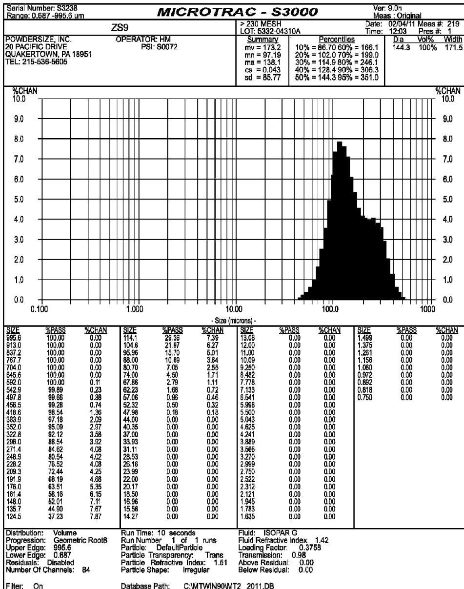
Fig. 9 (lot 5332-04310A 230 mesh)
