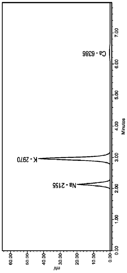
Fig. 16: Exemplary Sample Chromatogram.
