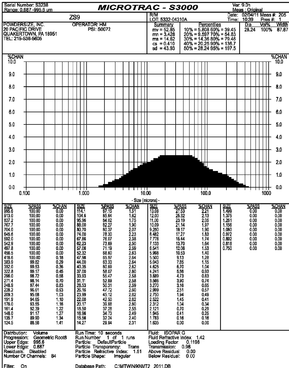
Fig. 5 (lot 5332-04310A w/o screening)
