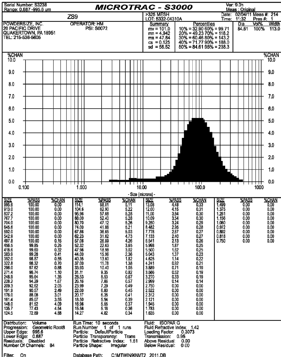
Fig. 8 (lot 5332-04310A 325 mesh)
