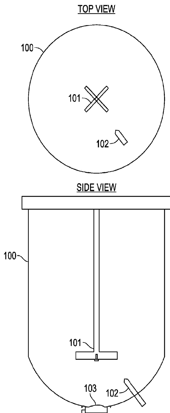
Fig. 17: 200-L reaction vessel with standard agitator arrangement.
