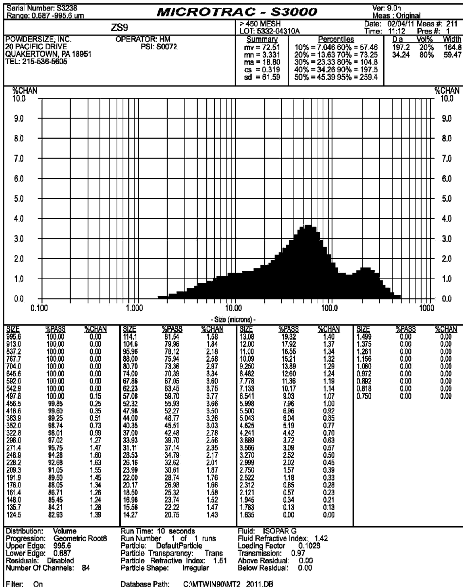
Fig. 7 (lot 5332-04310A 450 mesh)
