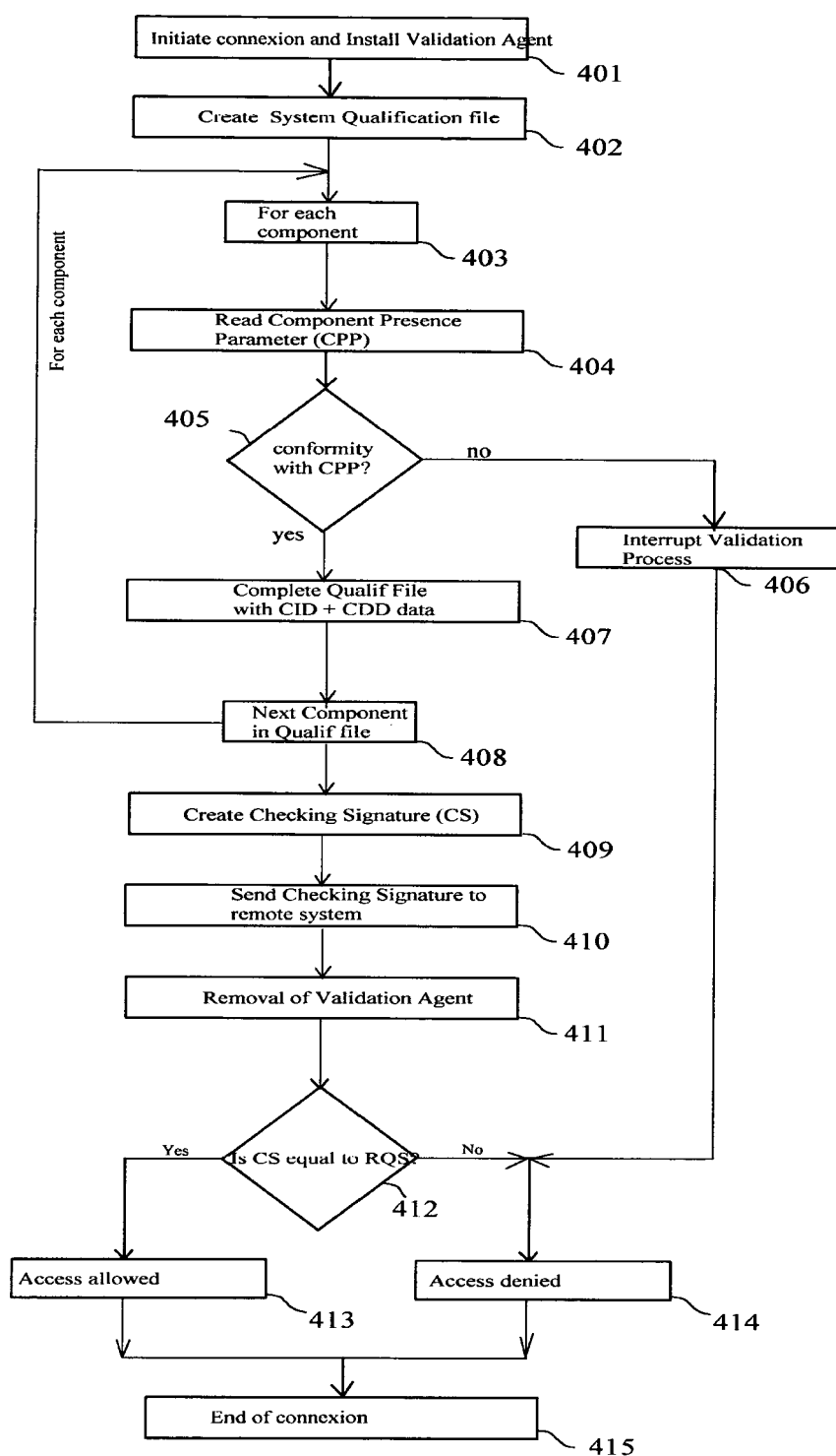
Fig. 4: Validation process ( remote)
