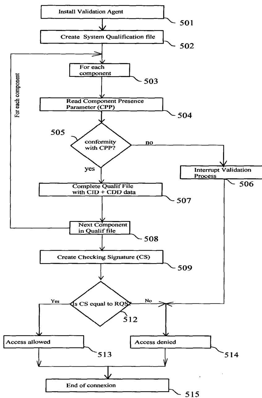
Fig. 5: Validation process ( local )
