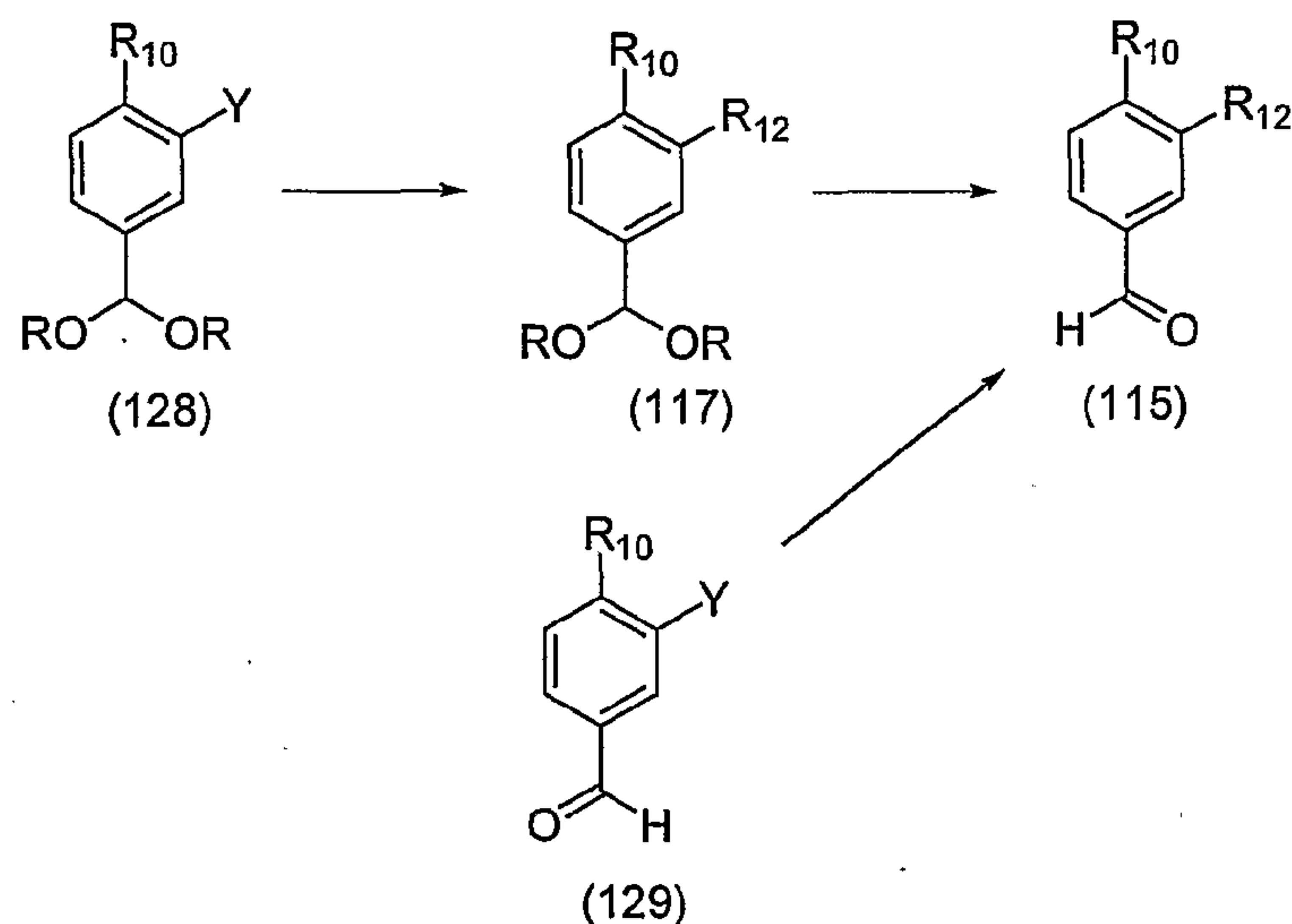
Scheme 44
