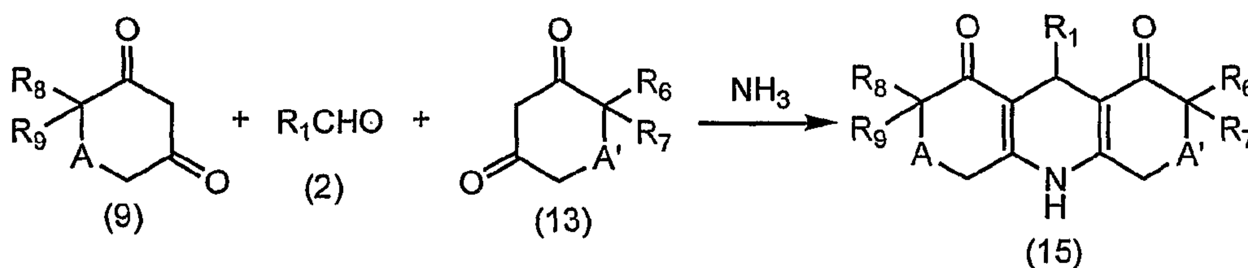
Scheme 5
