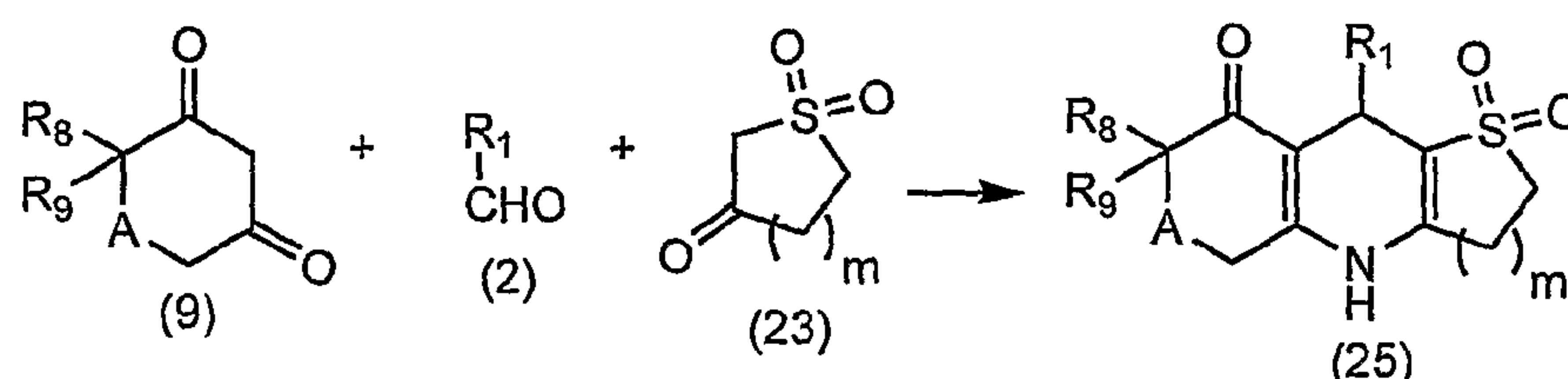
Scheme 8
