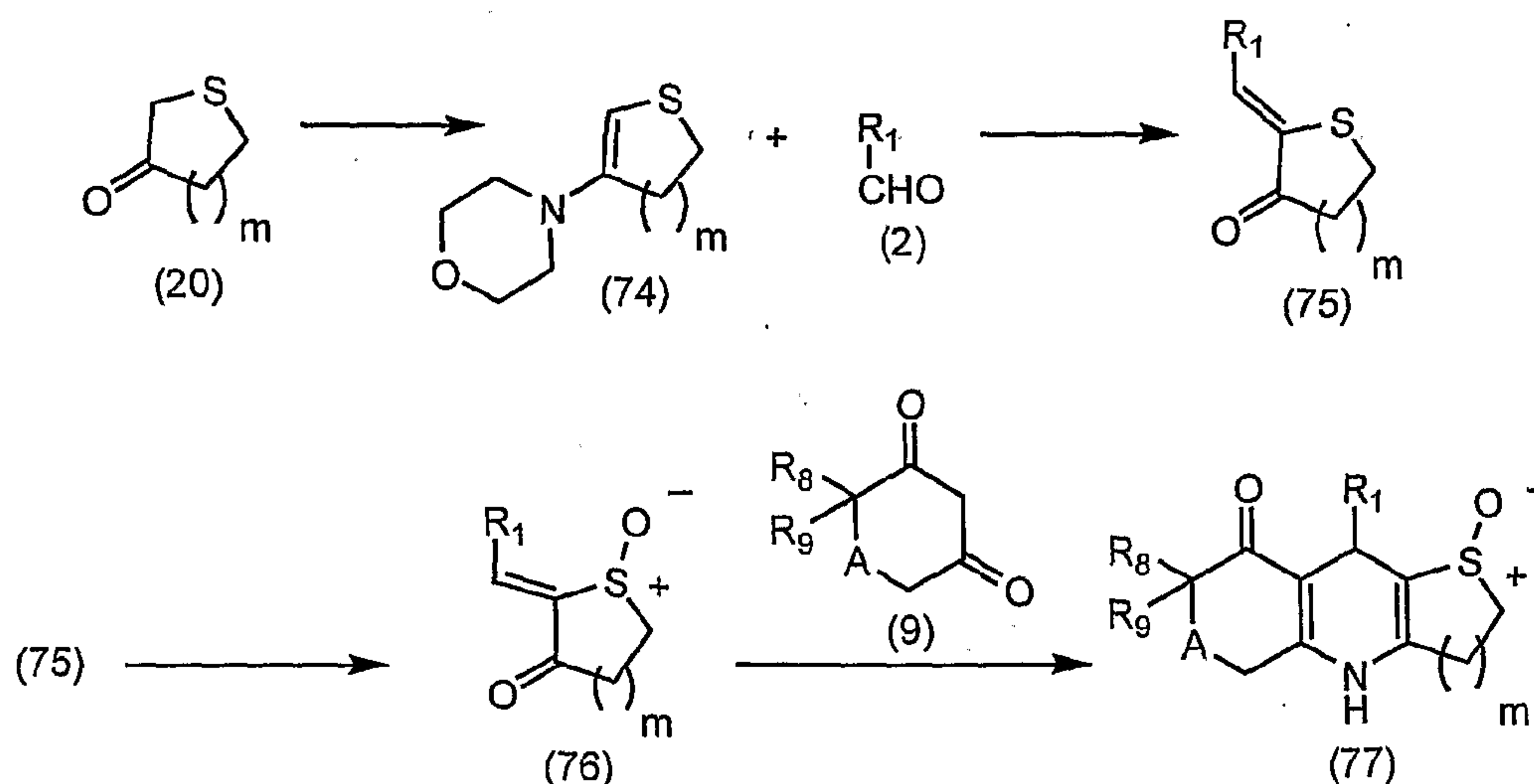
Scheme 27
