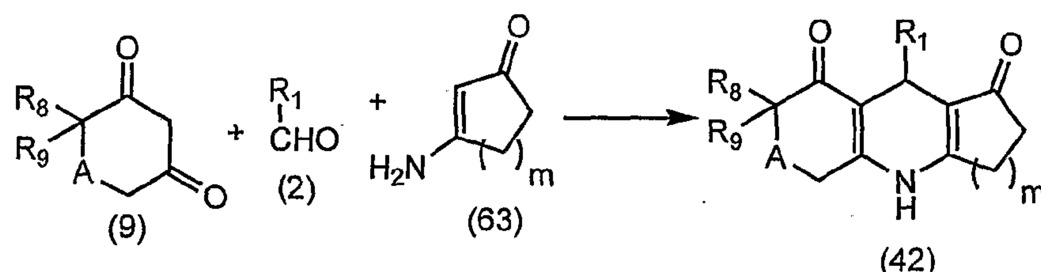
Scheme 22
