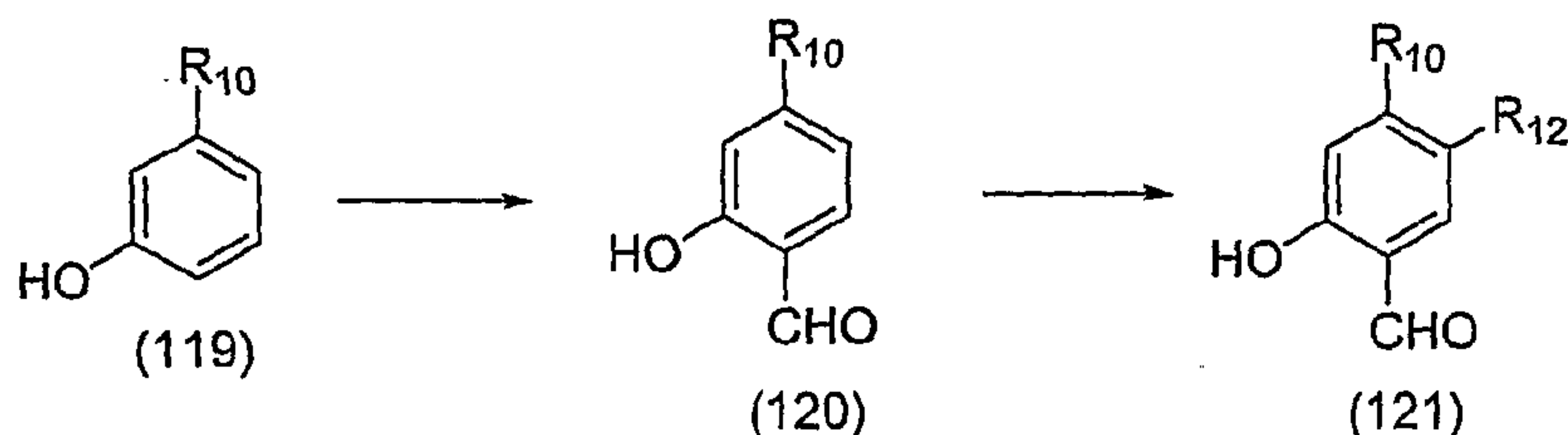
Scheme 41
