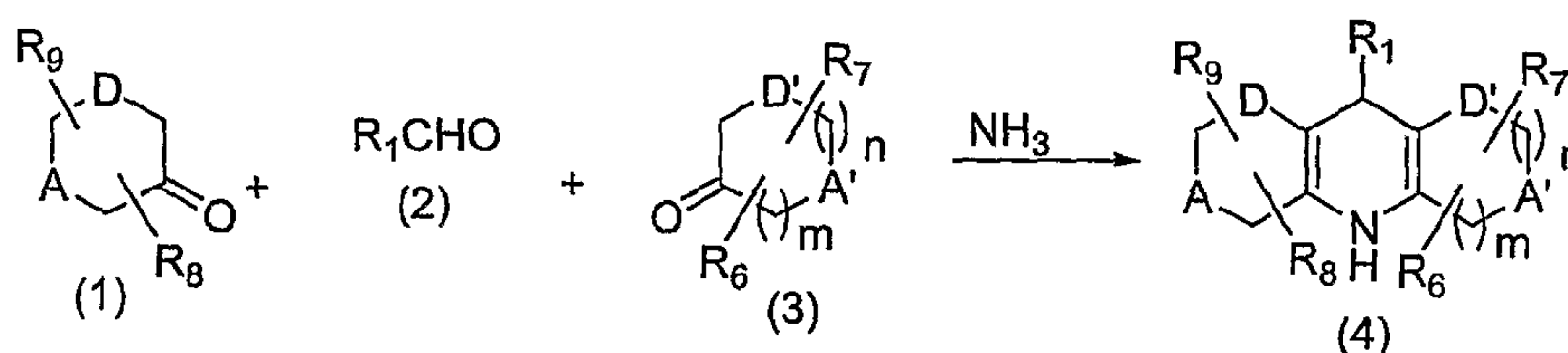
Scheme 1
