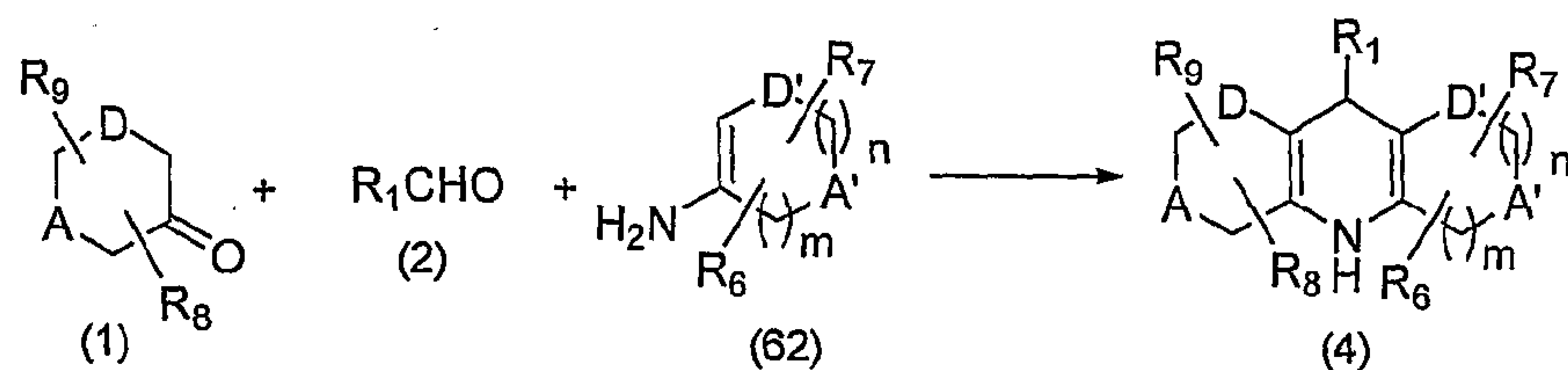
Scheme 21
