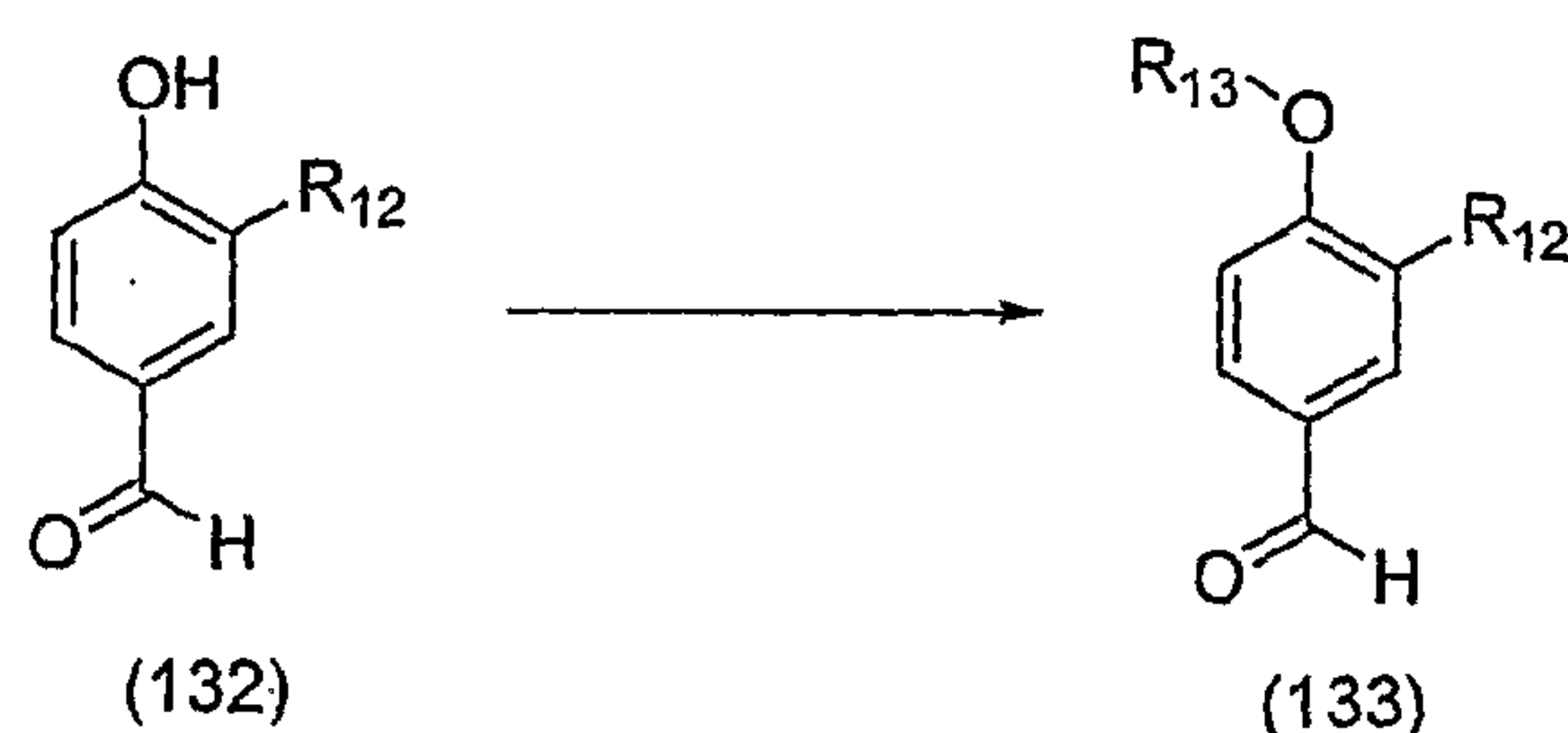
Scheme 46
