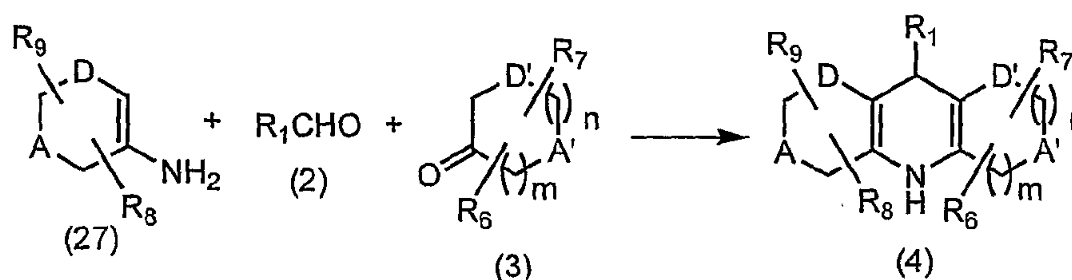
Scheme 9
