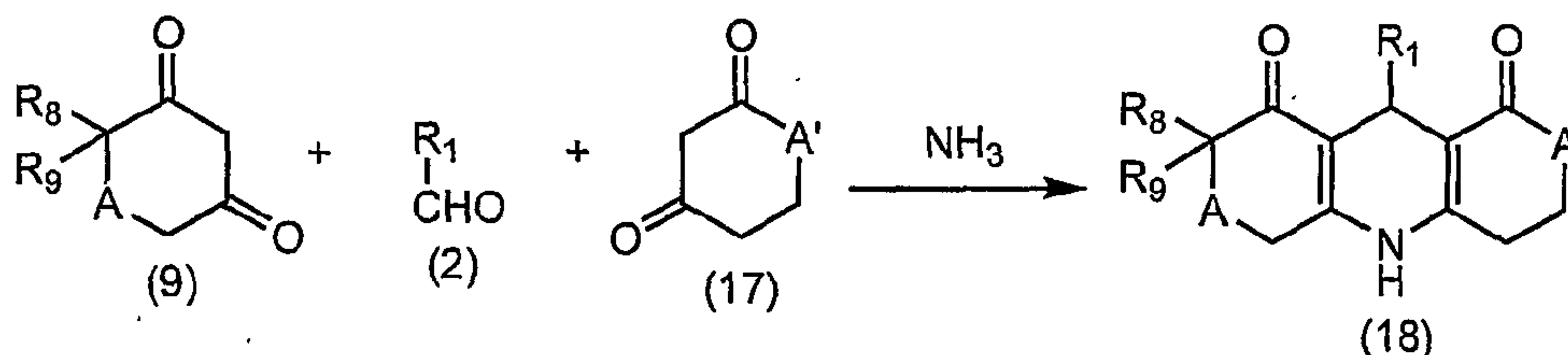
Scheme 6
