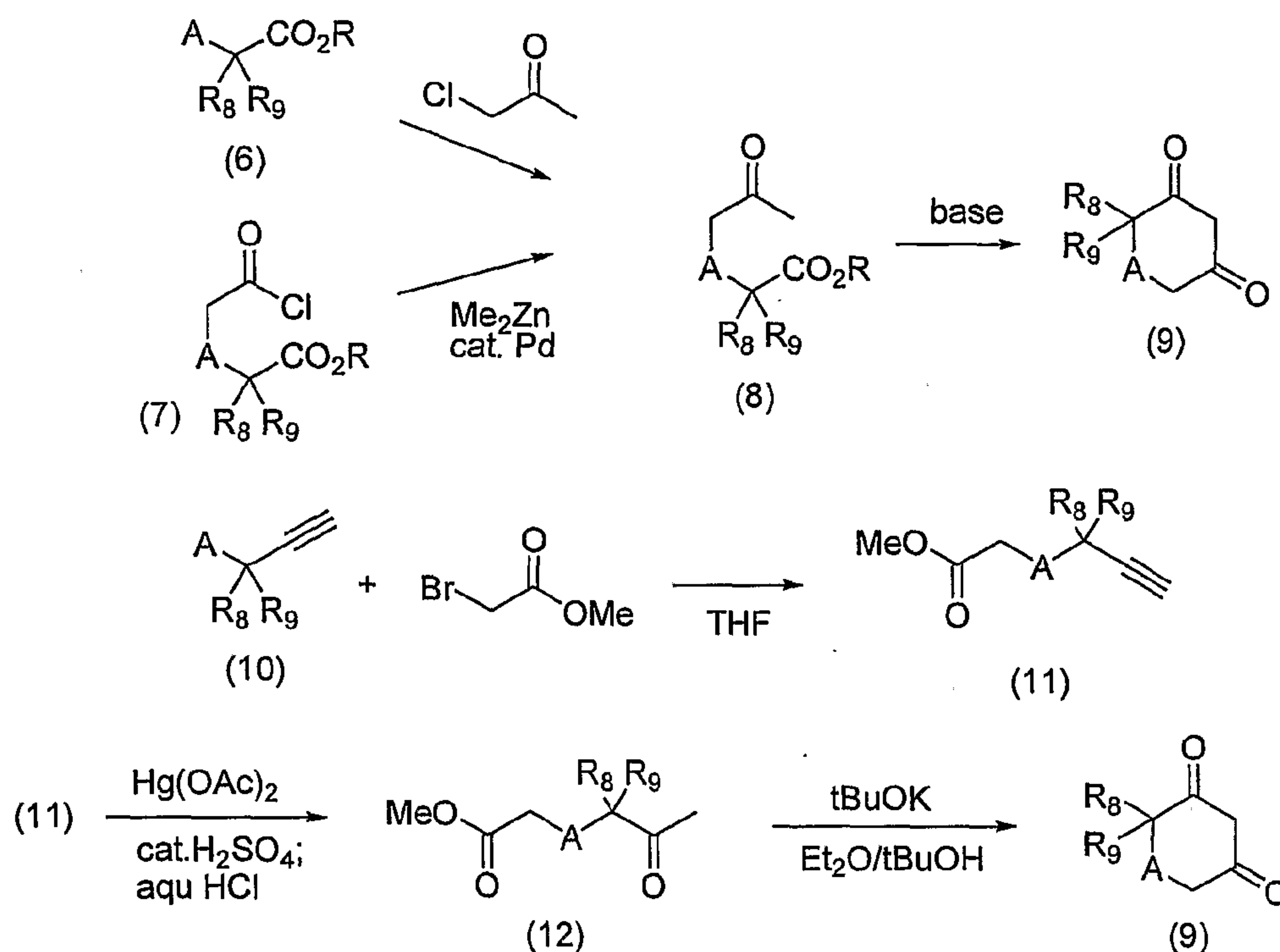
Scheme 2
