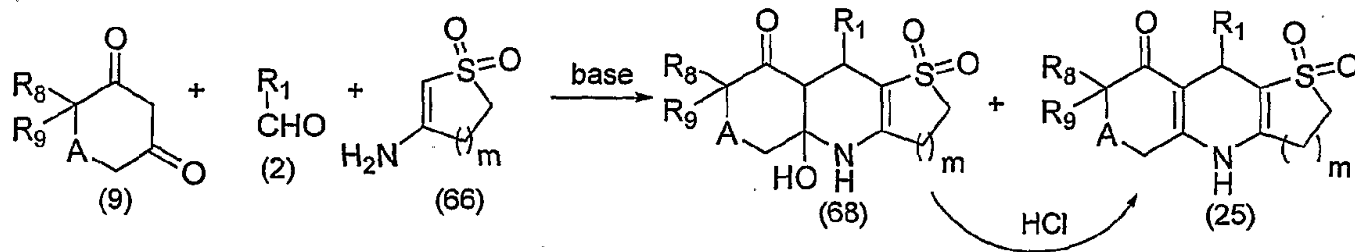
Scheme 24
