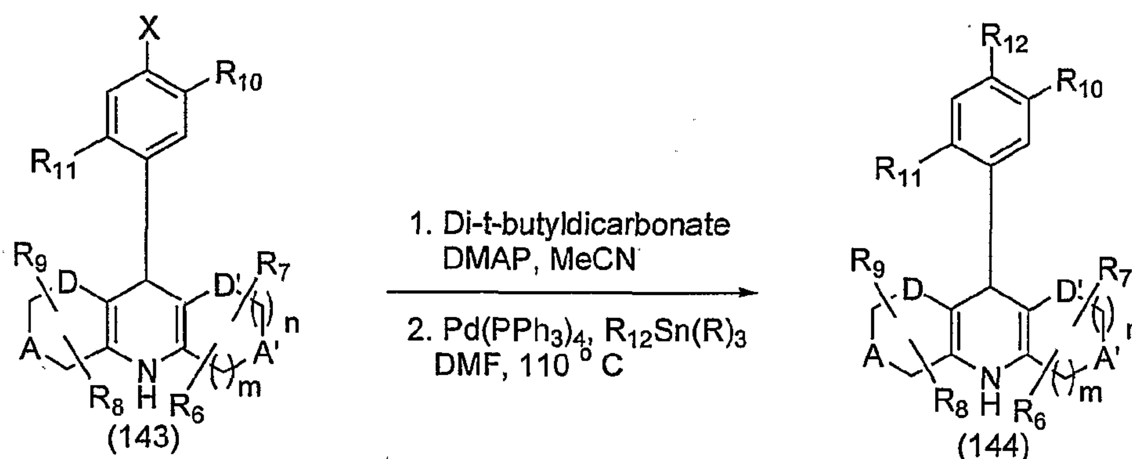
Scheme 52
