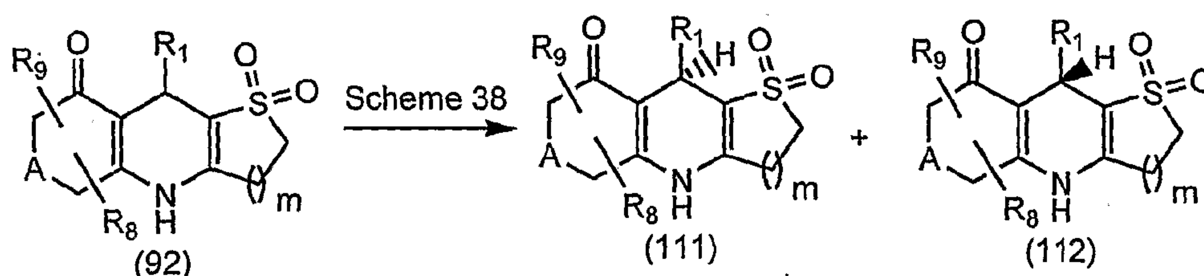
Scheme 39
