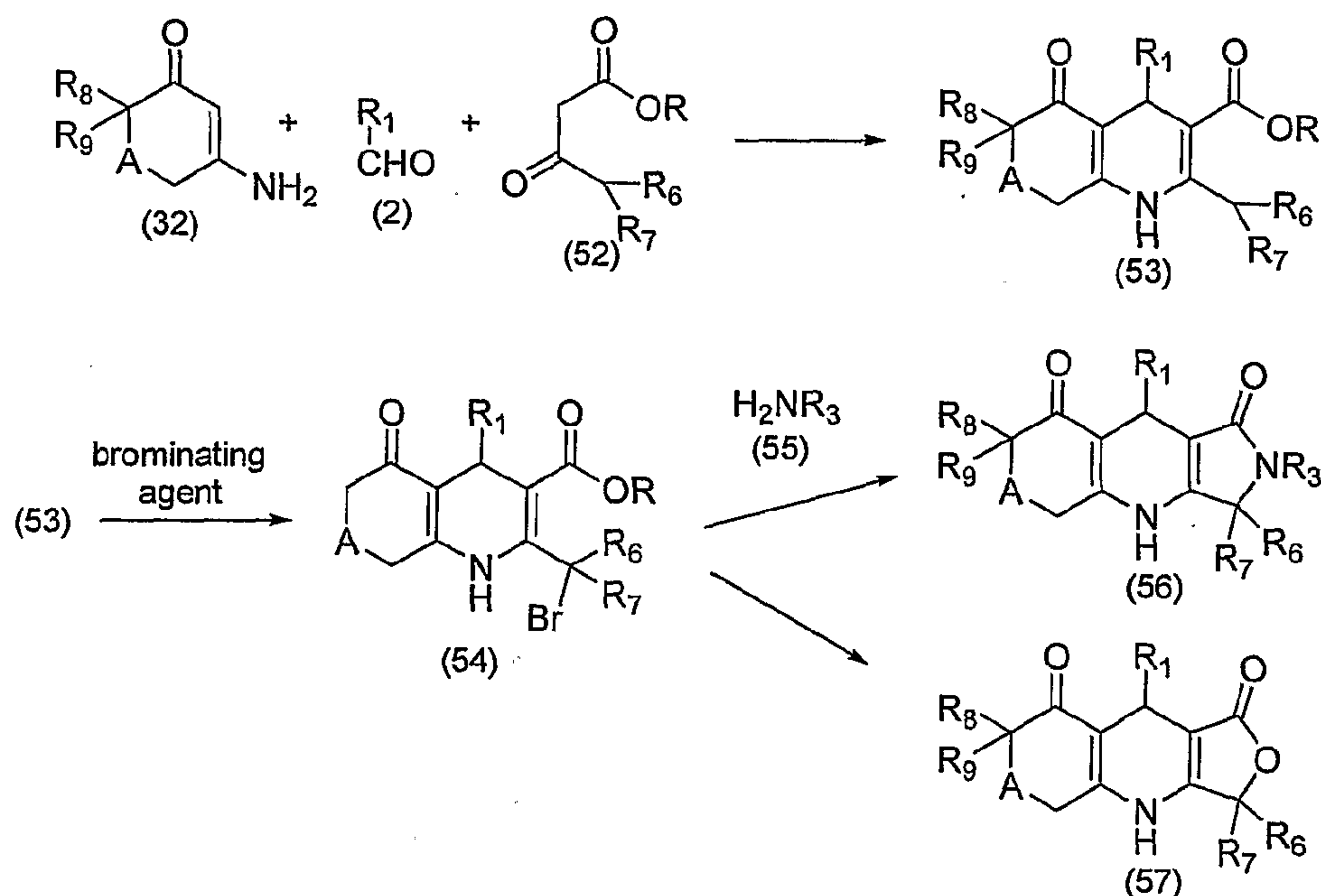
Scheme 19
