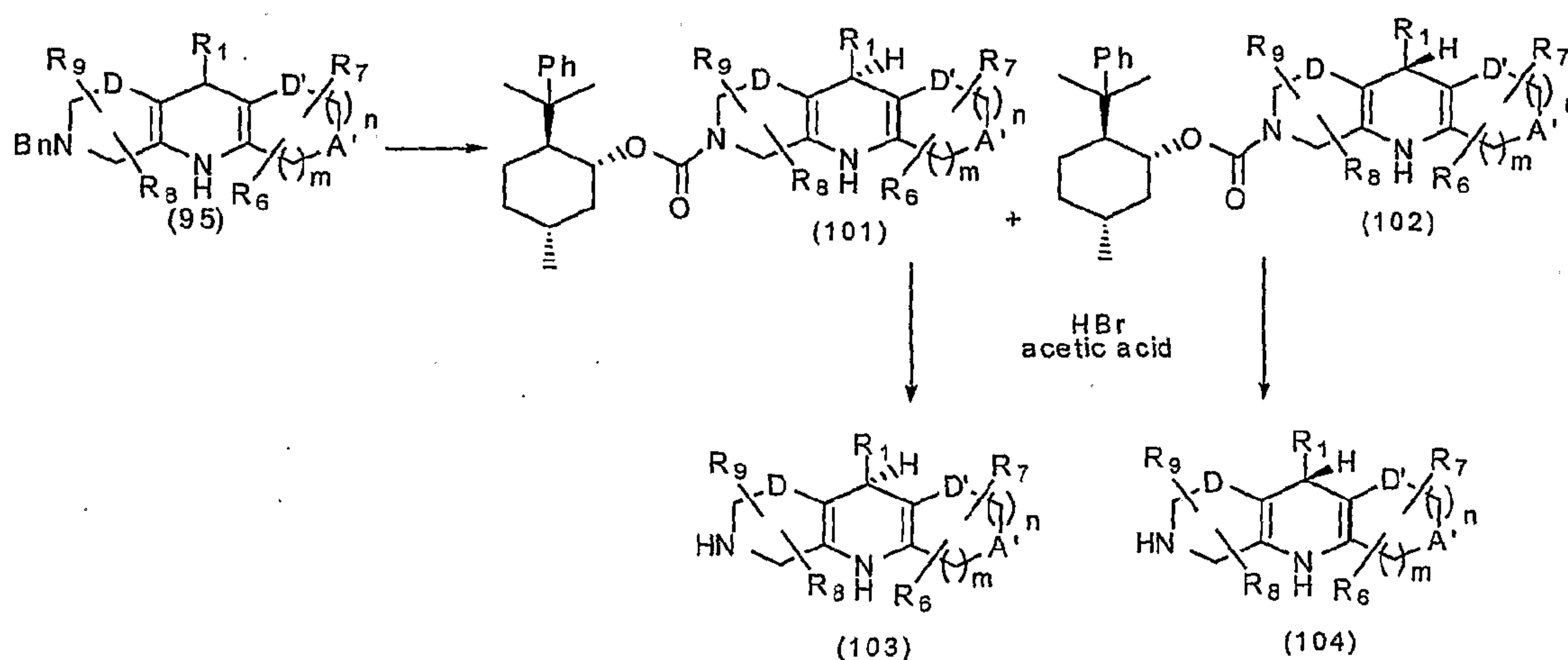
Scheme 37
