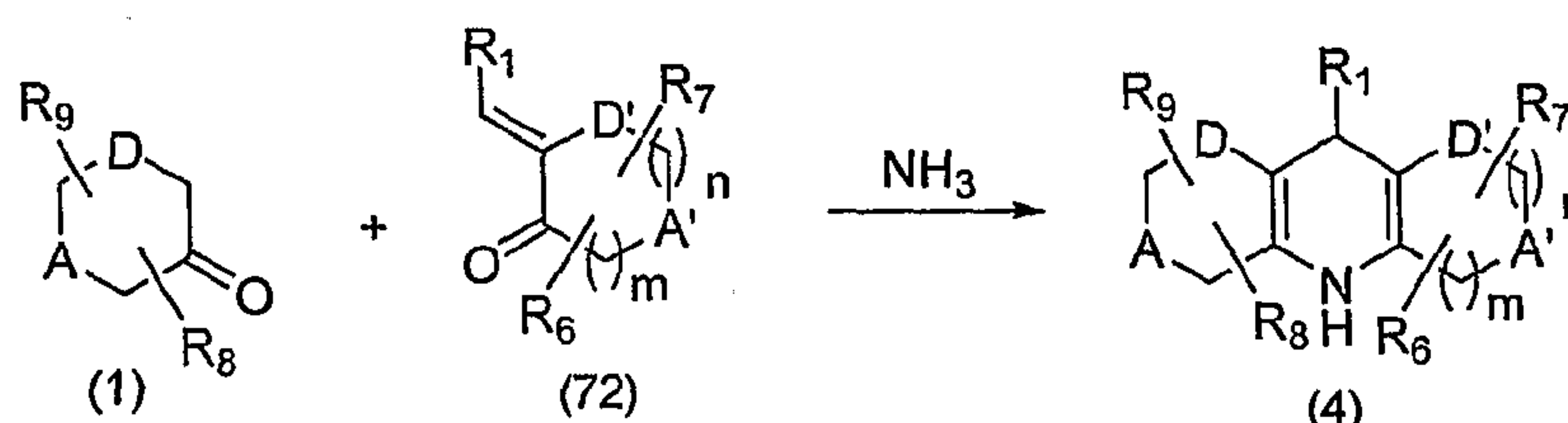
Scheme 26
