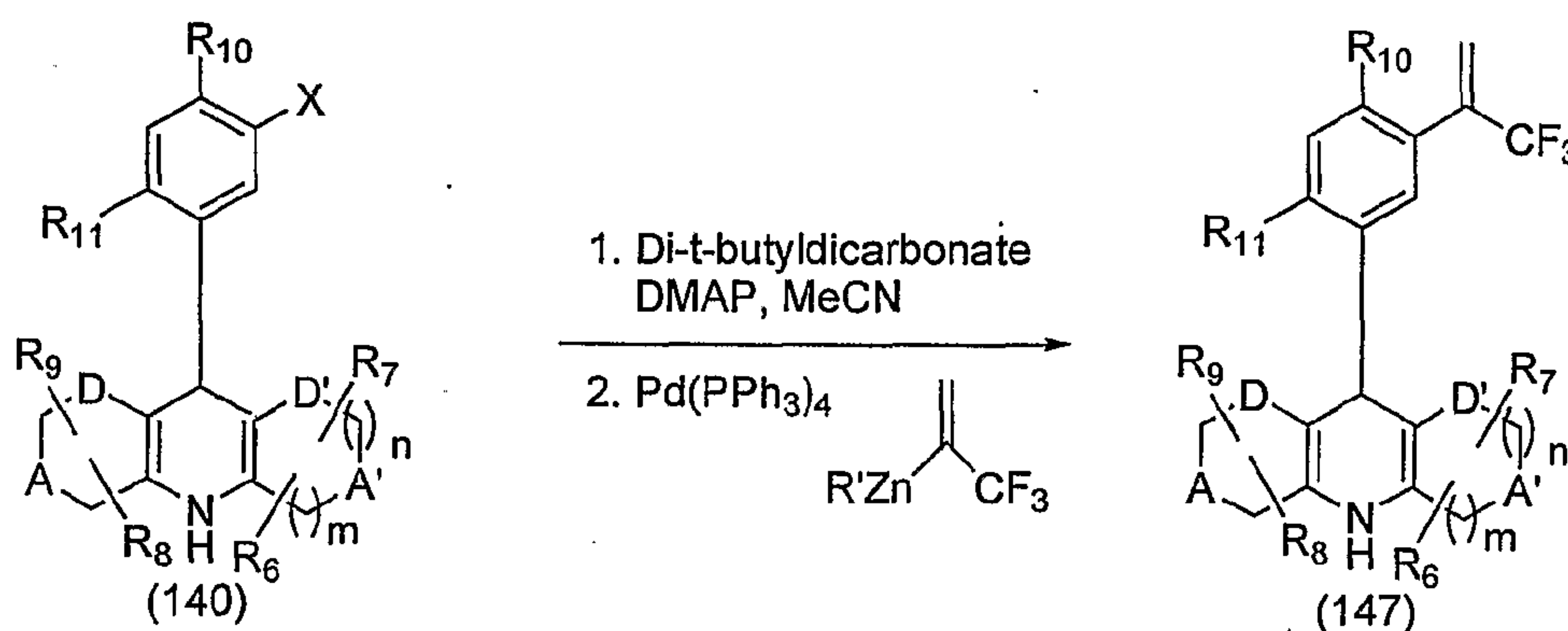
Scheme 53
