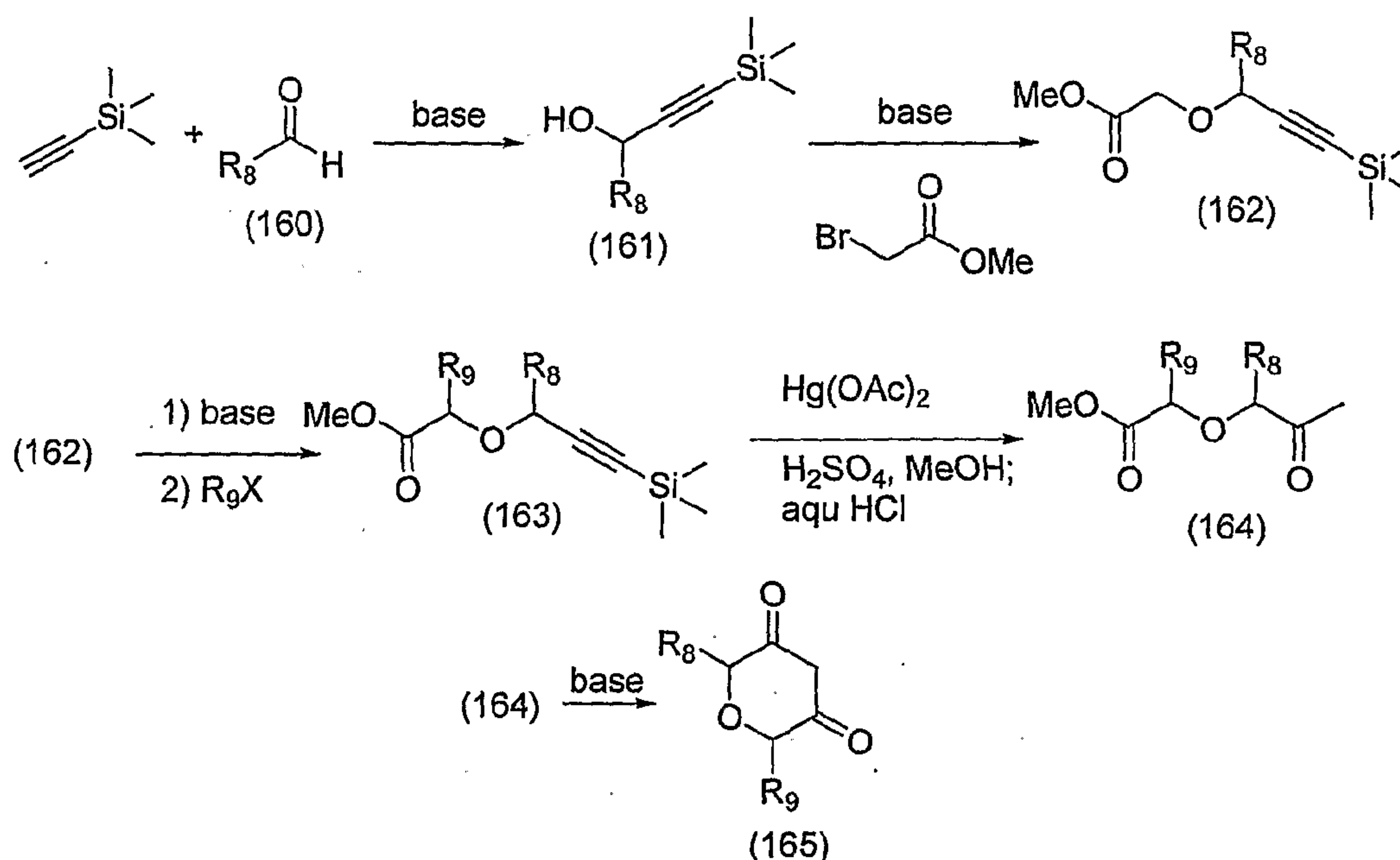
Scheme 55
