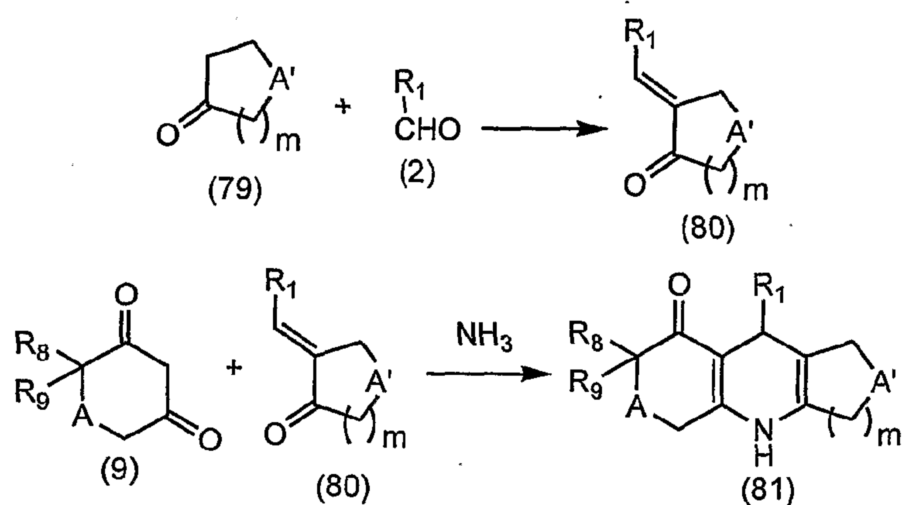
Scheme 28
