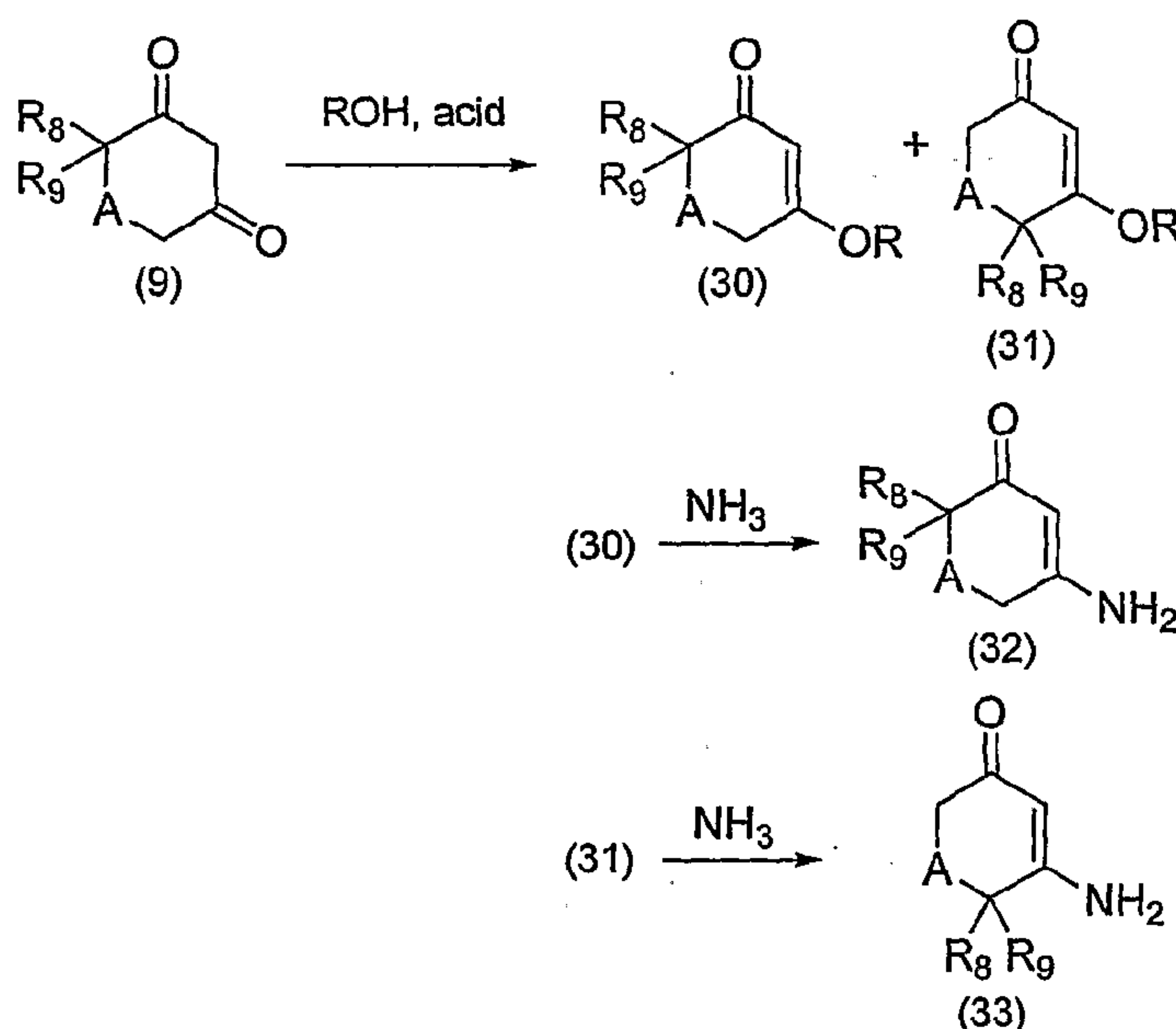
Scheme 10
