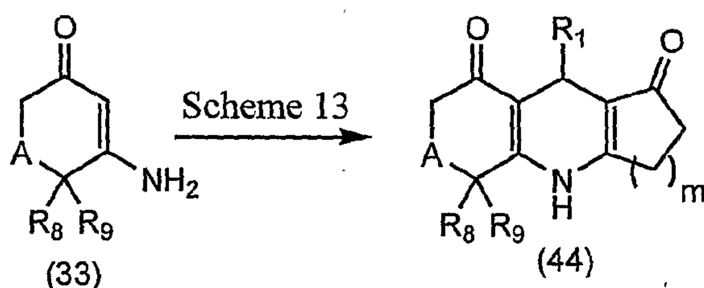
Scheme 14
