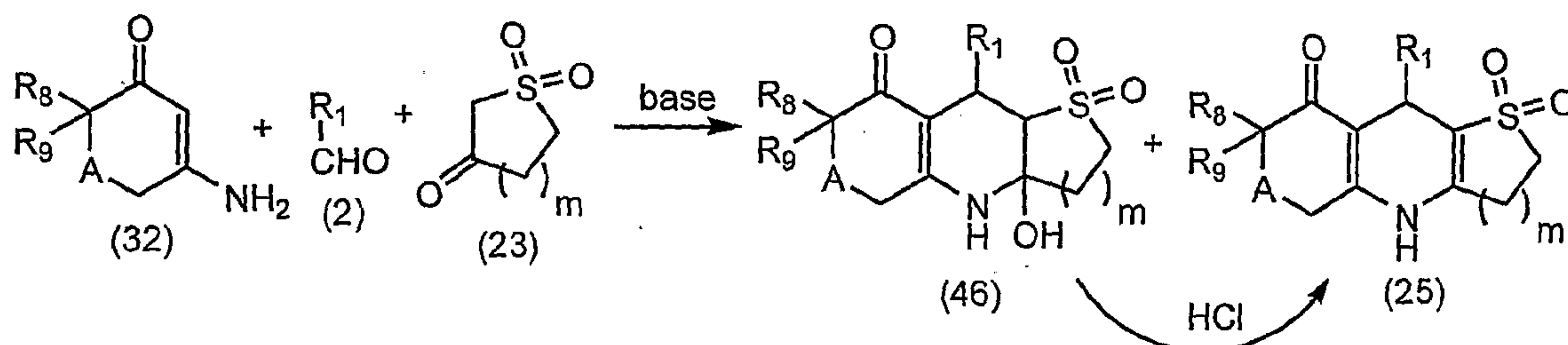
Scheme 15
