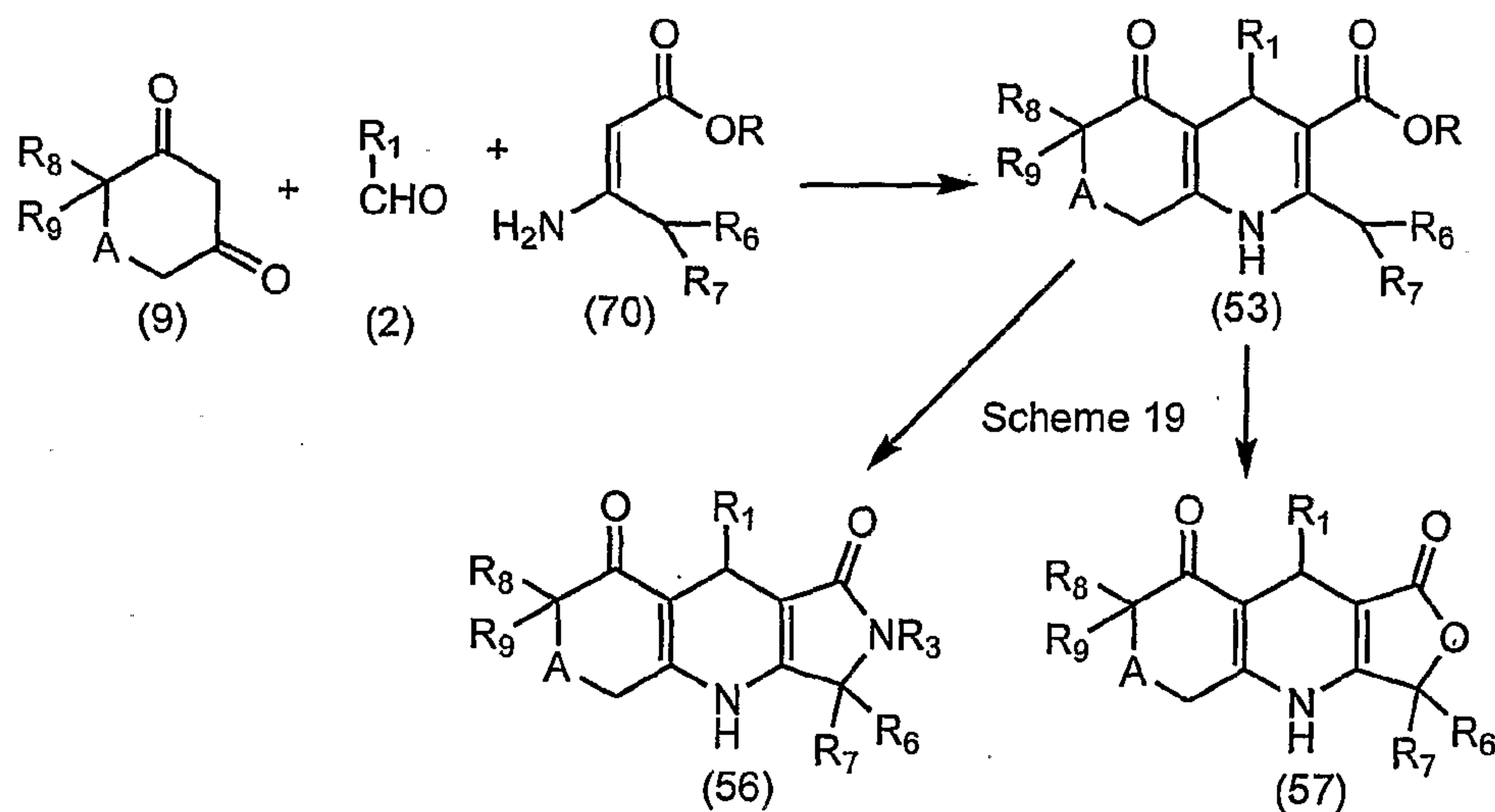
Scheme 25
