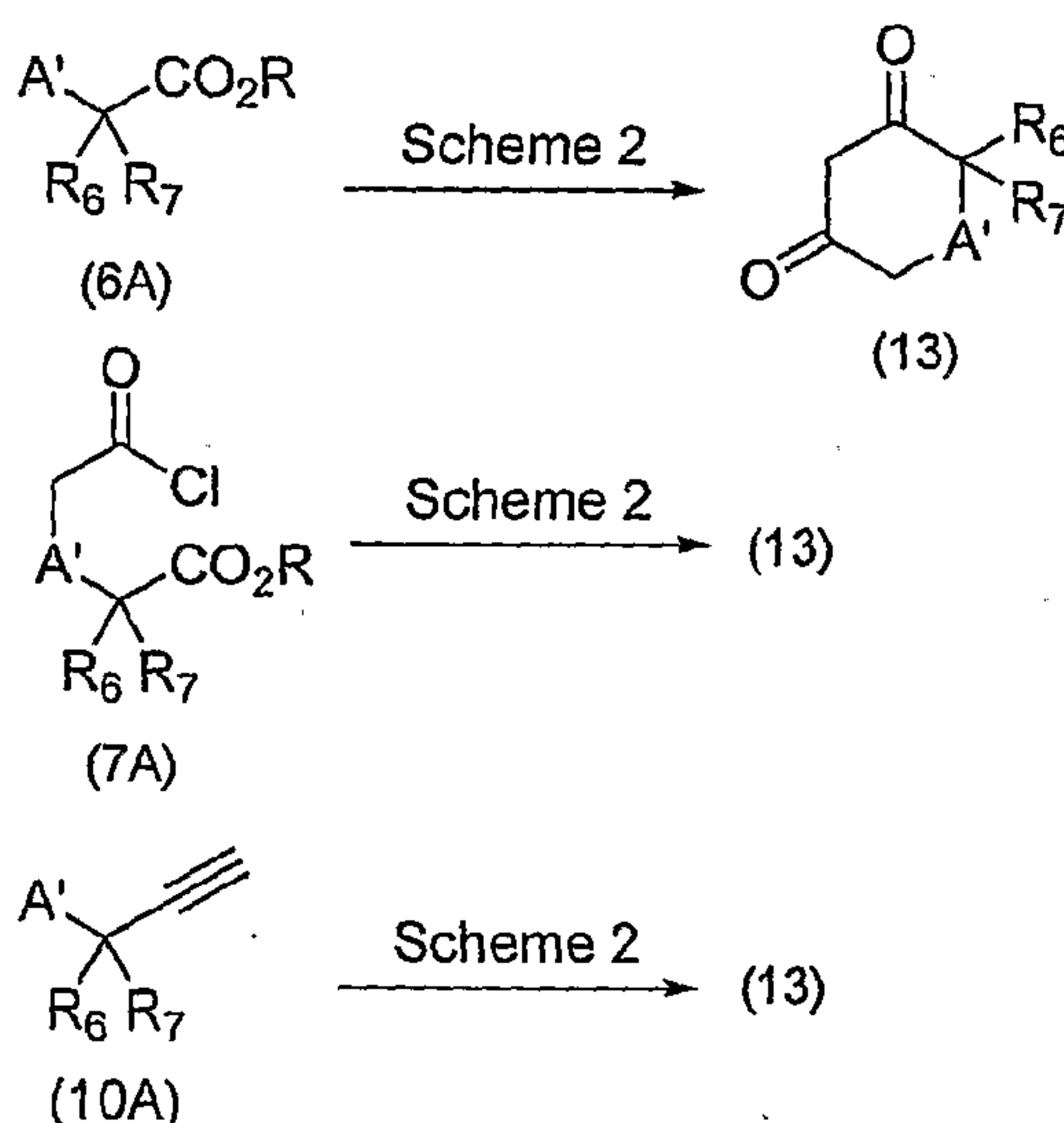
Scheme 3
