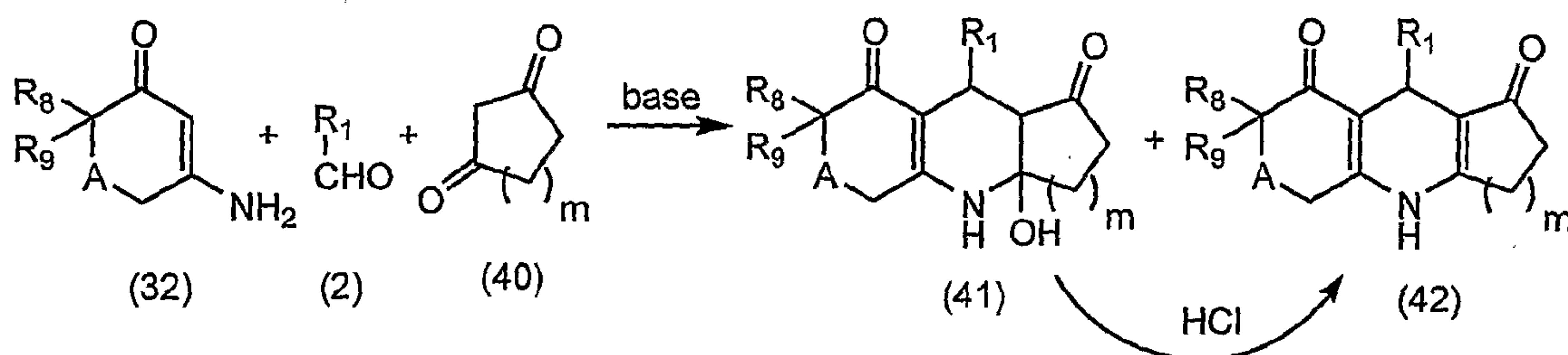
Scheme 13
