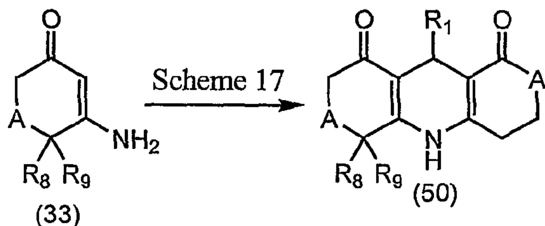
Scheme 18
