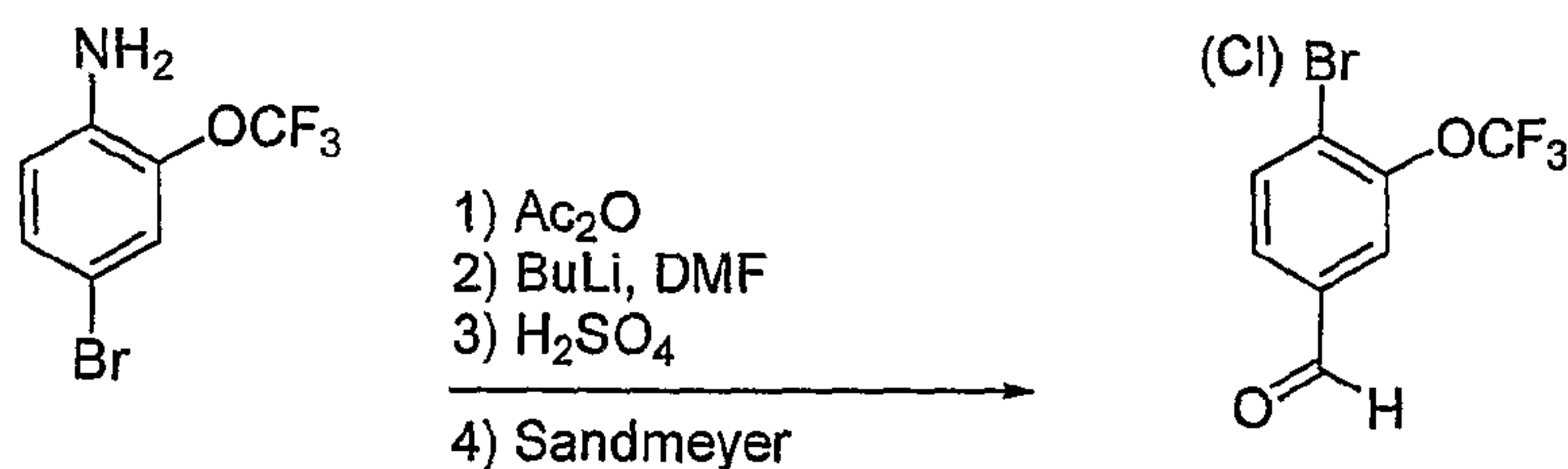
Scheme 49
