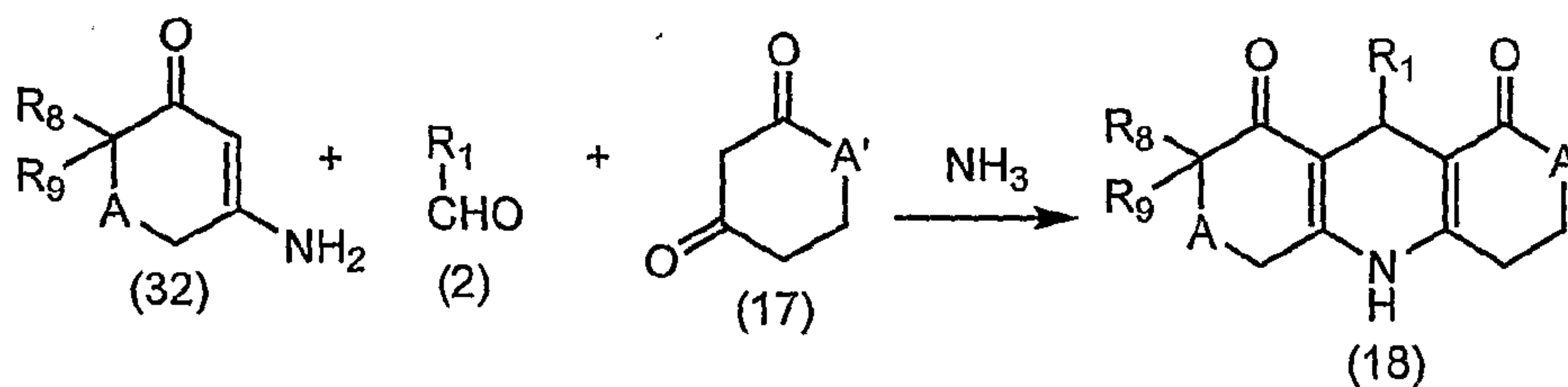
Scheme 17
