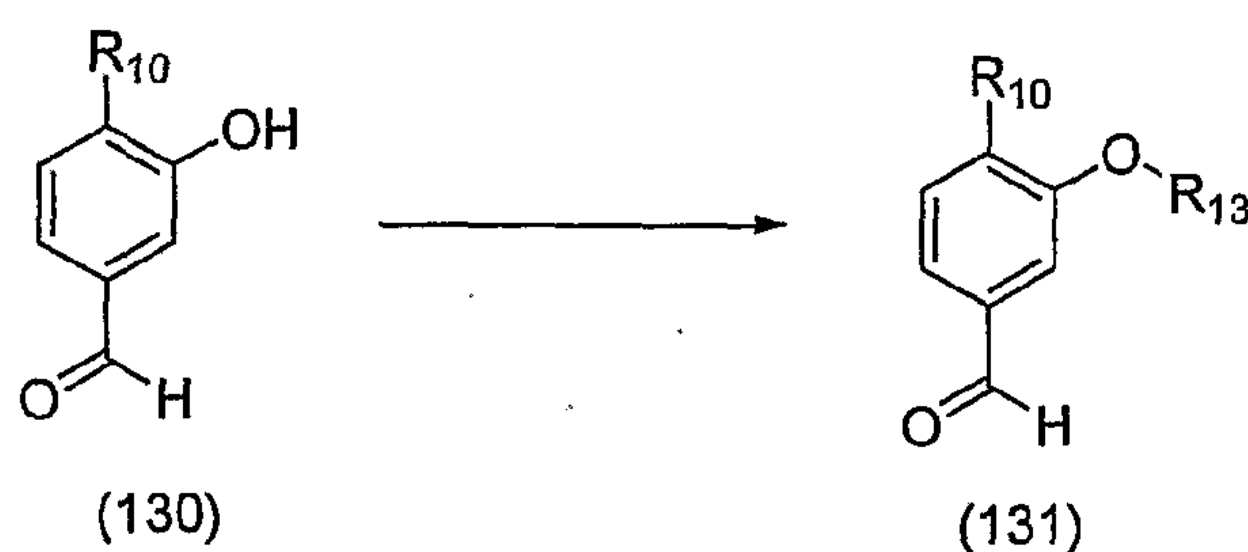
Scheme 45
