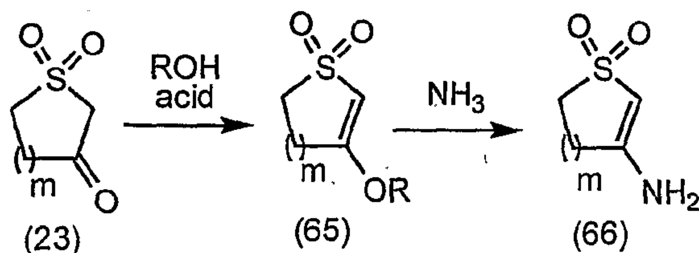
Scheme 23
