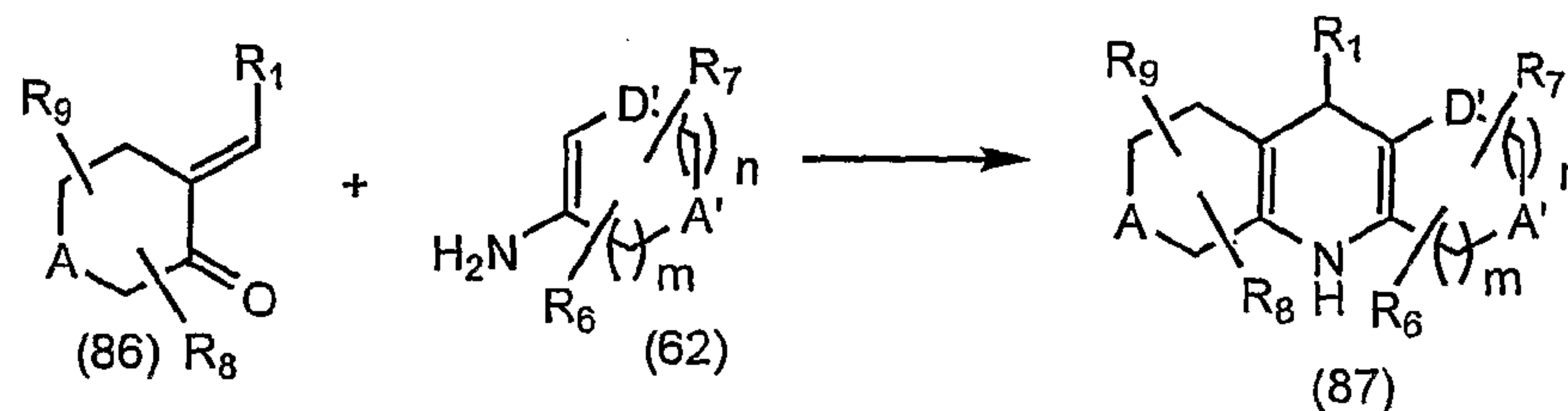
Scheme 33
