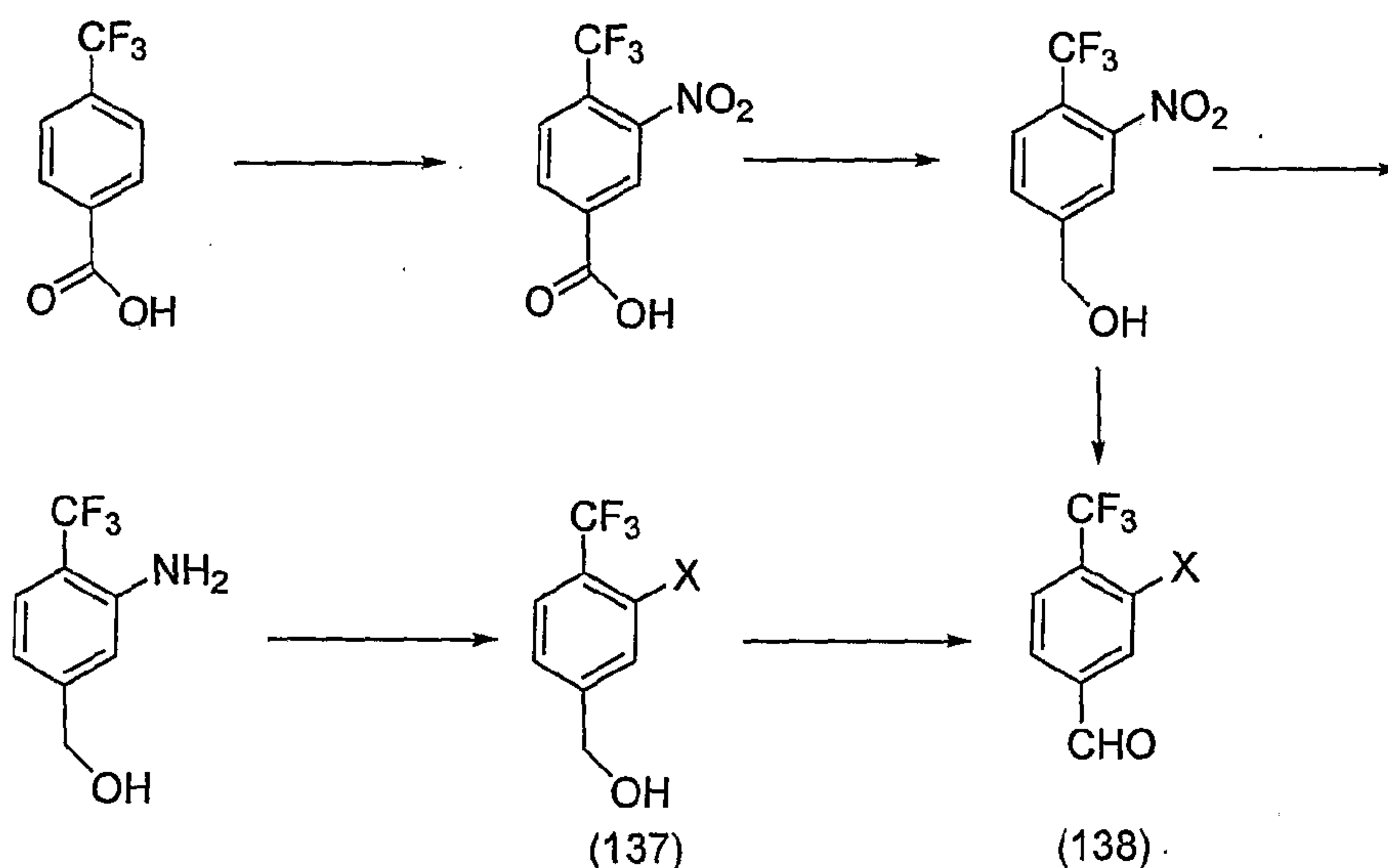
Scheme 50
