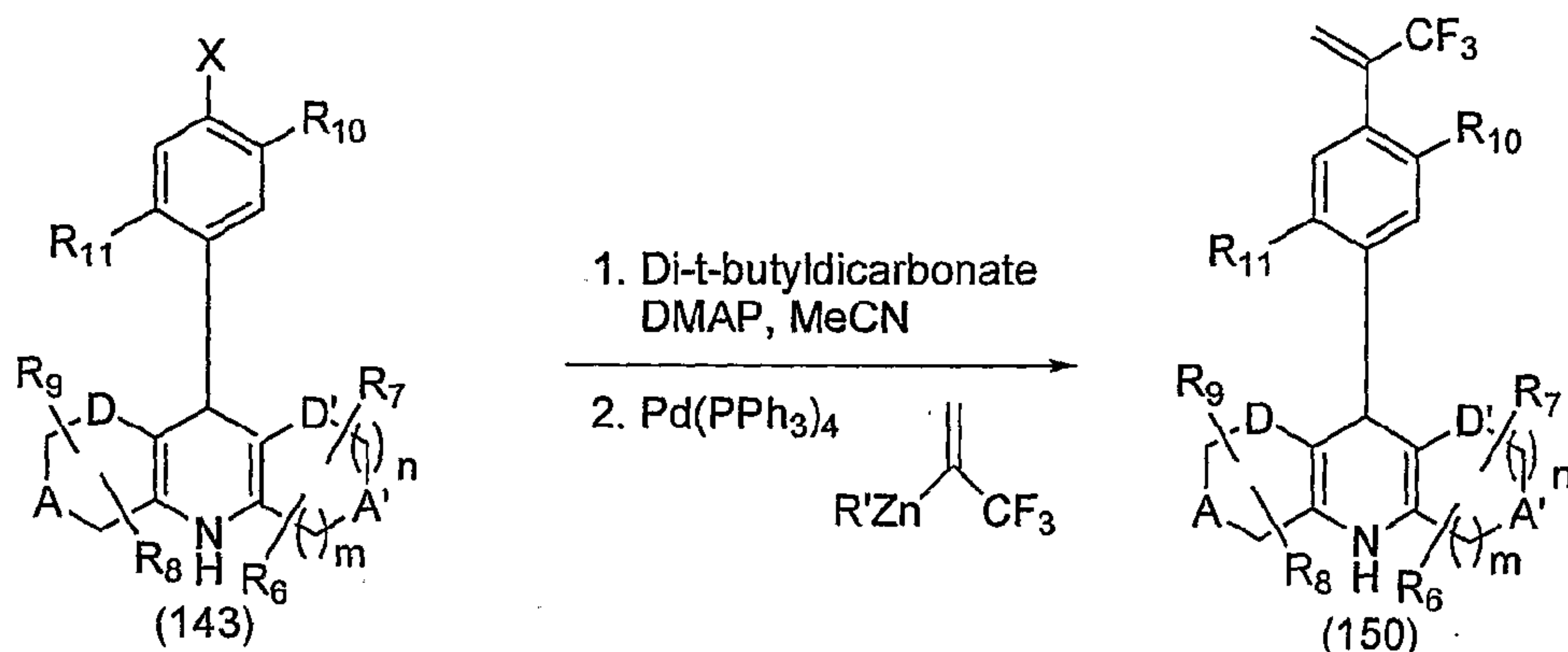
Scheme 54
