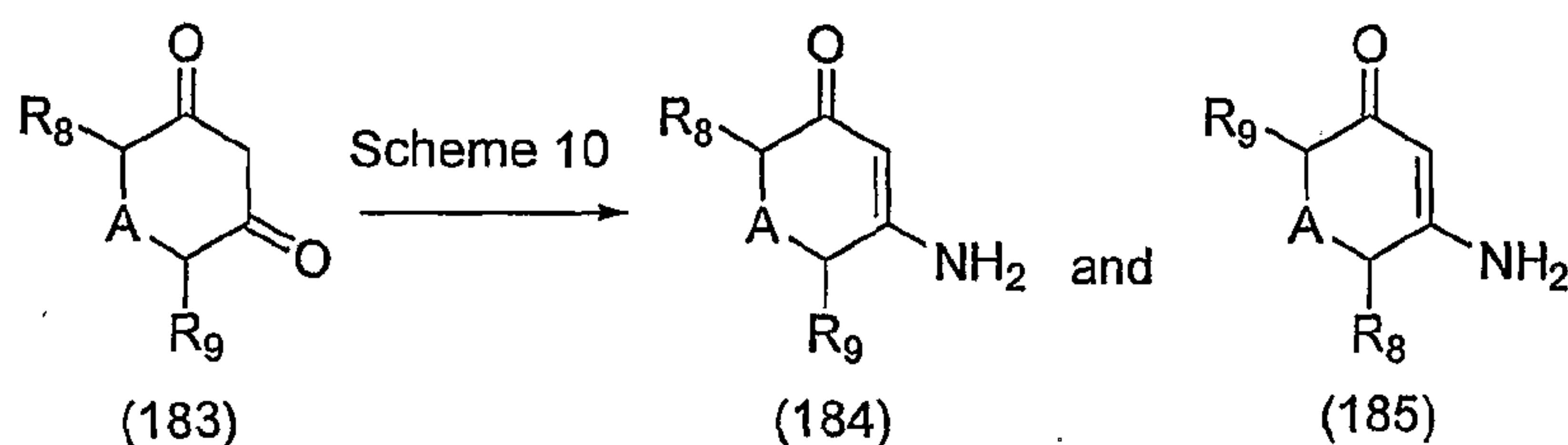
Scheme 58
