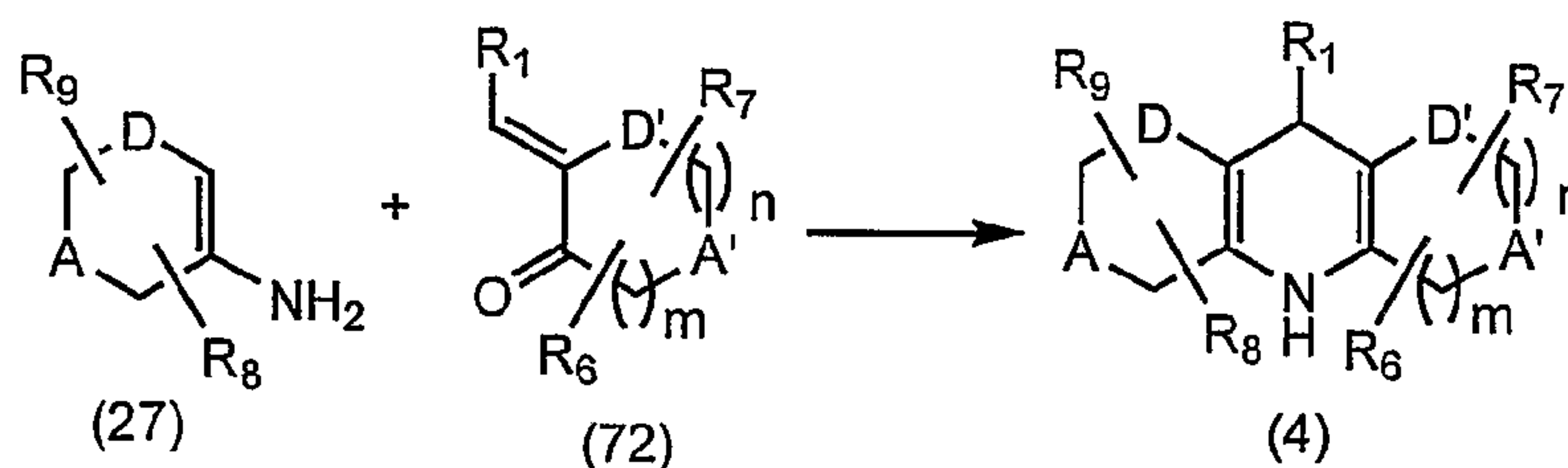
Scheme 29
