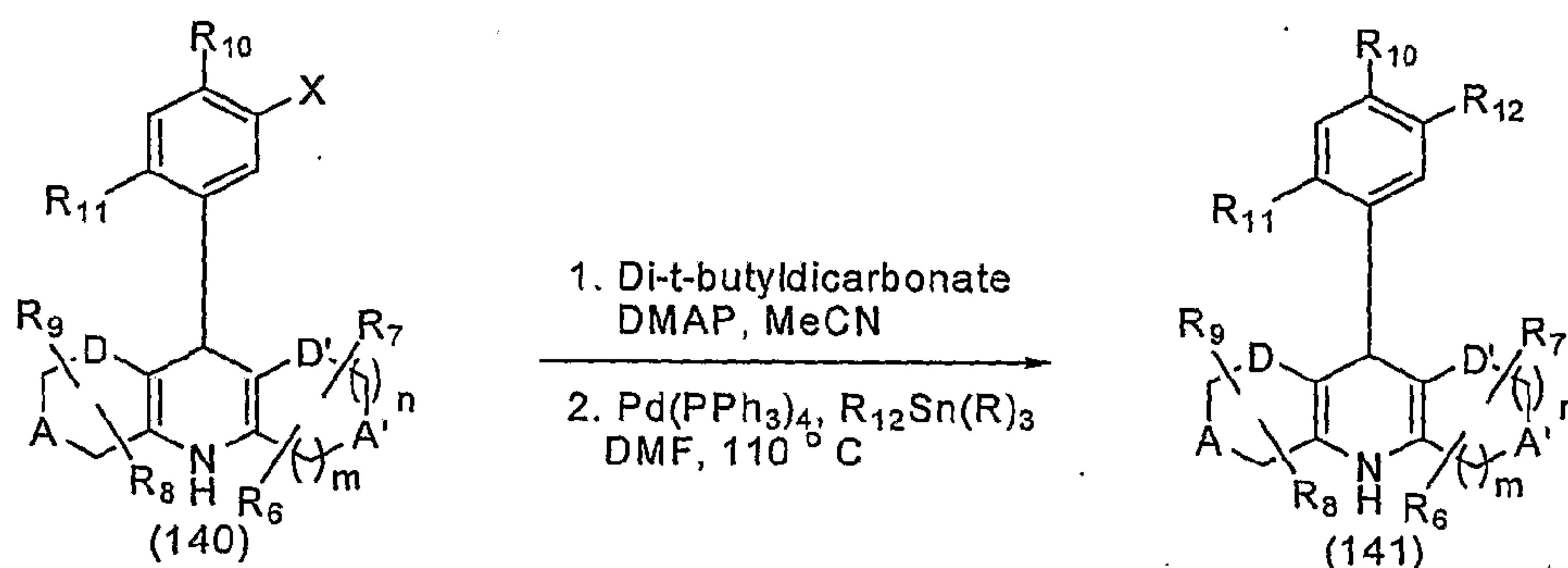
Scheme 51
