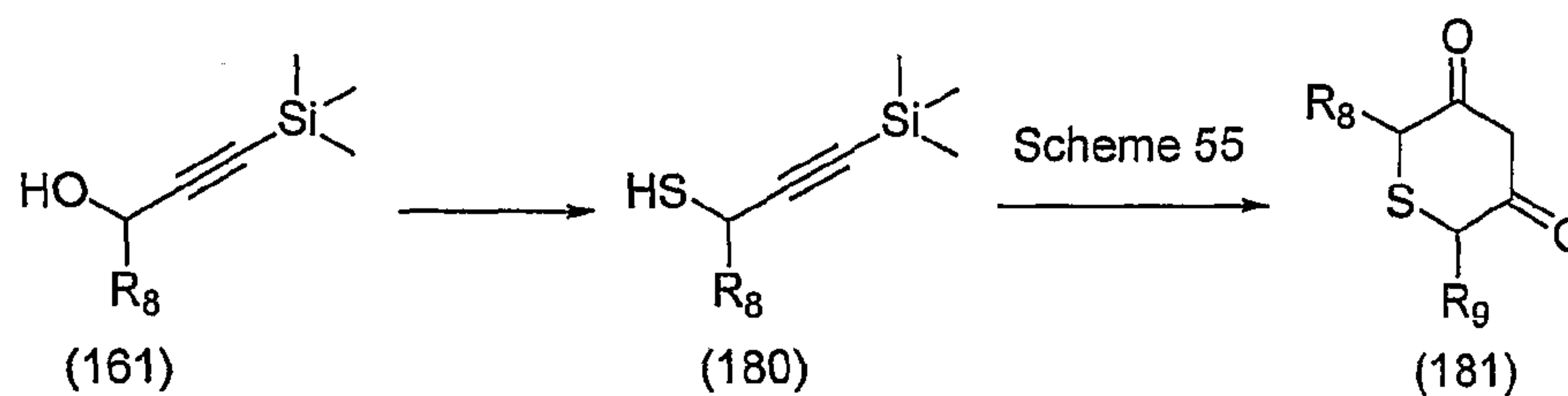
Scheme 57
