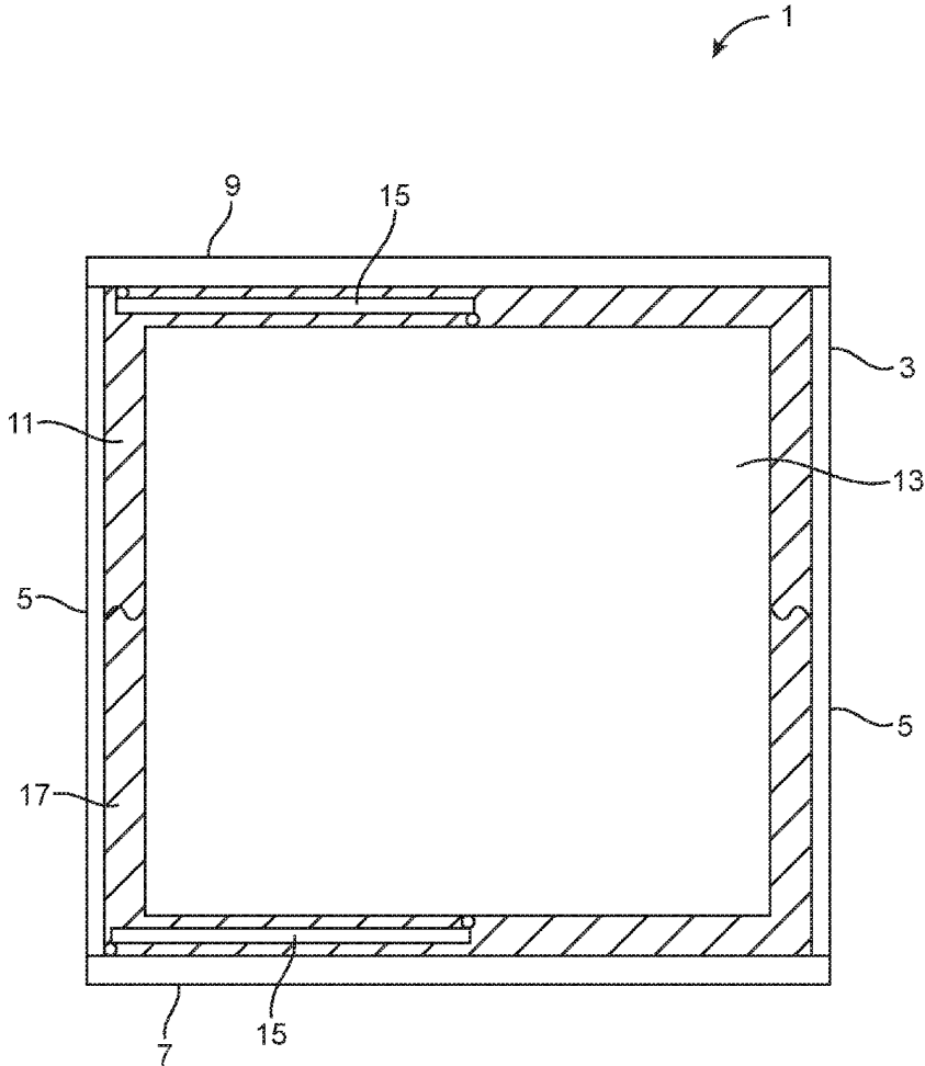
FIG. 1 (PRIOR ART)
