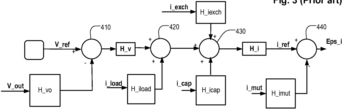
Fig. 4 (Prior art)
