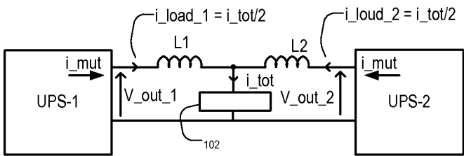
Fig. 2 (Prior art)
