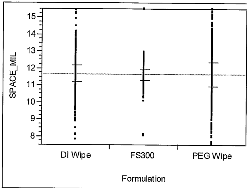
Frequency [kHz]=30 Oneway Analysis of SPACE_MIL By Formulation
