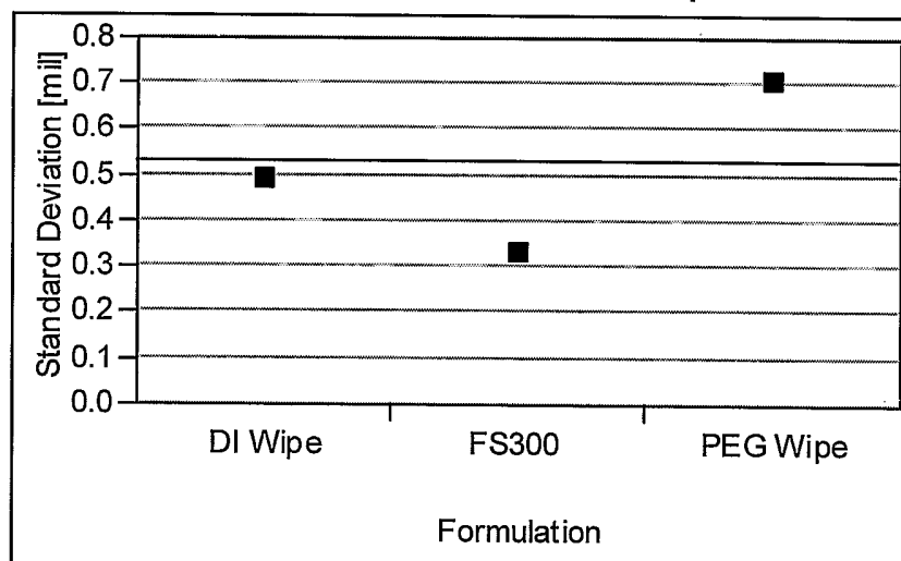
Tests that the Variances are Equal
