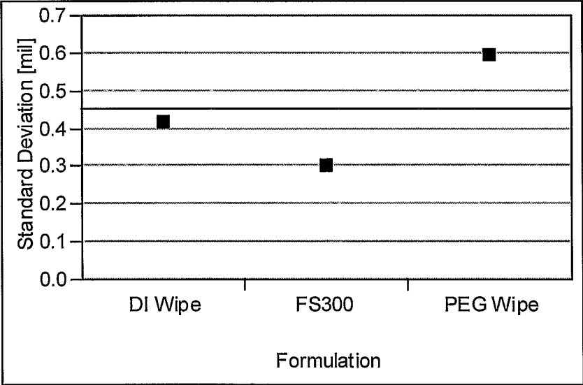
Tests that the Variances are Equal
