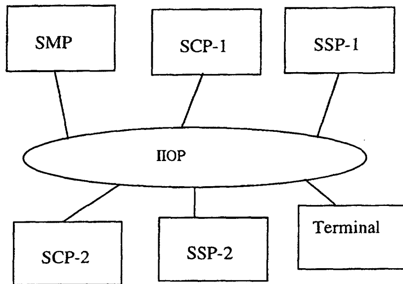
Figure 4: Architecture 3
