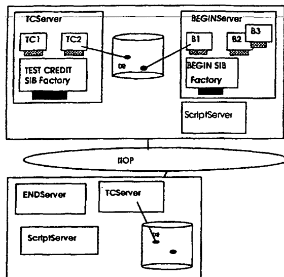
Figure 3: Architecture 2
