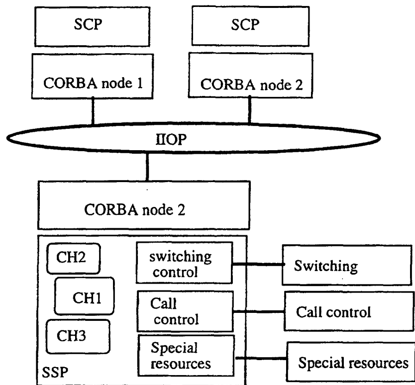
Figure 5: SSP Server
