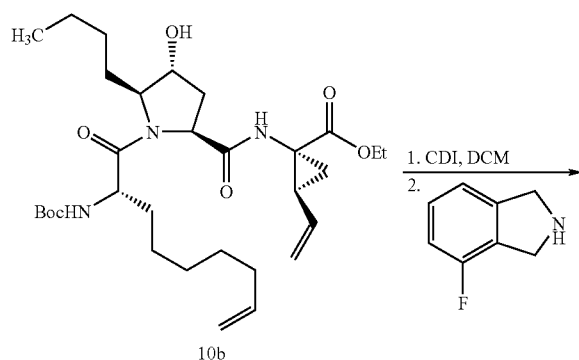
Scheme 11
