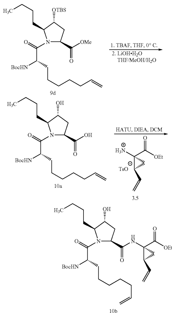
Scheme 10
