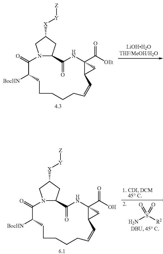
Scheme 6
