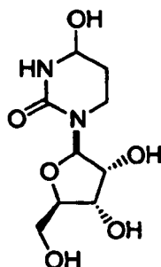
Tetrahydrouridine (THU)
