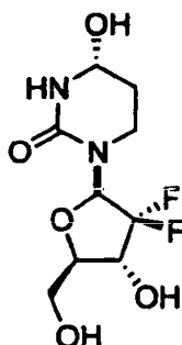
Compound 1a.
