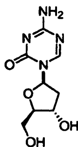
5-aza-2'-deoxycytidine (decitabine)
