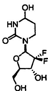
Compound 1
