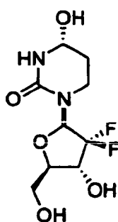
Compound 1a.
