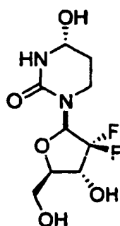
Compound 1a.
