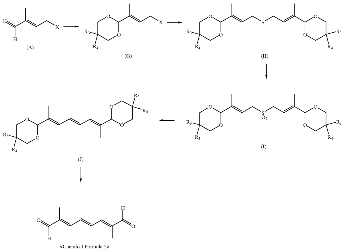
Scheme 5
