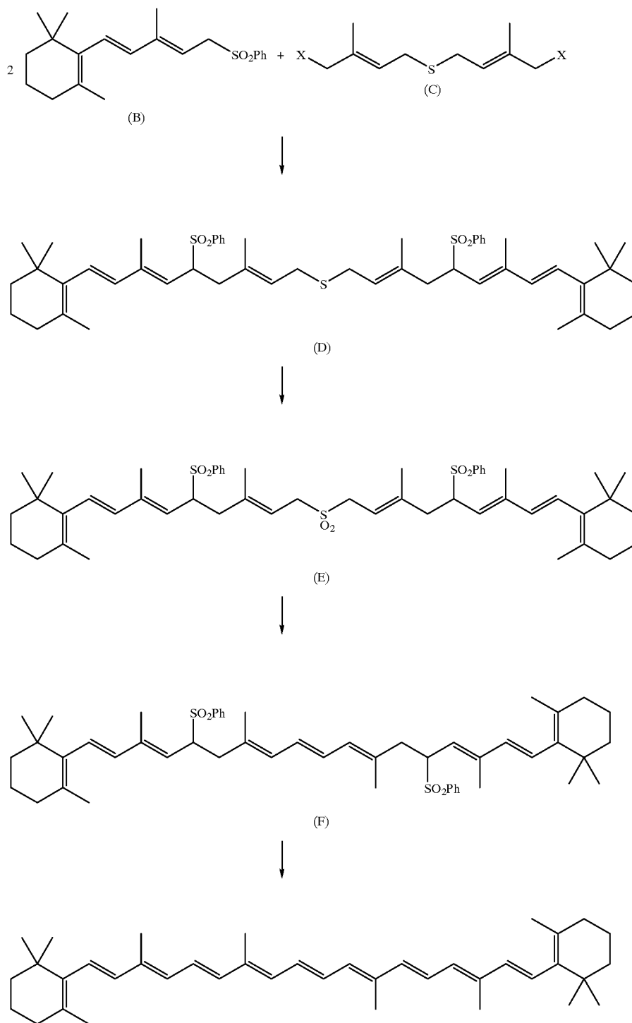
Scheme 6
