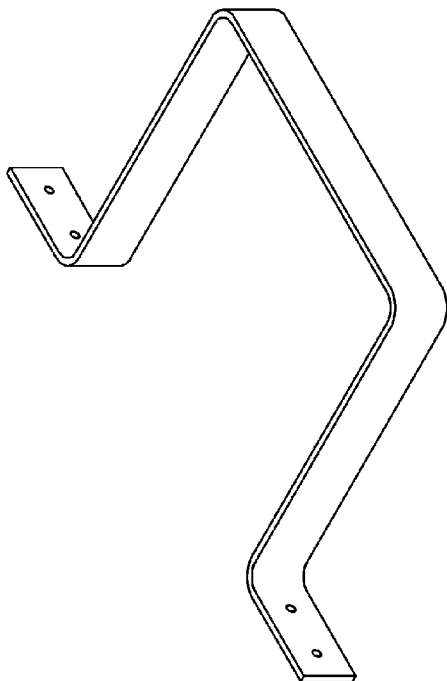
FIG. 3A. ISOMETRIC NOT TO SCALE
