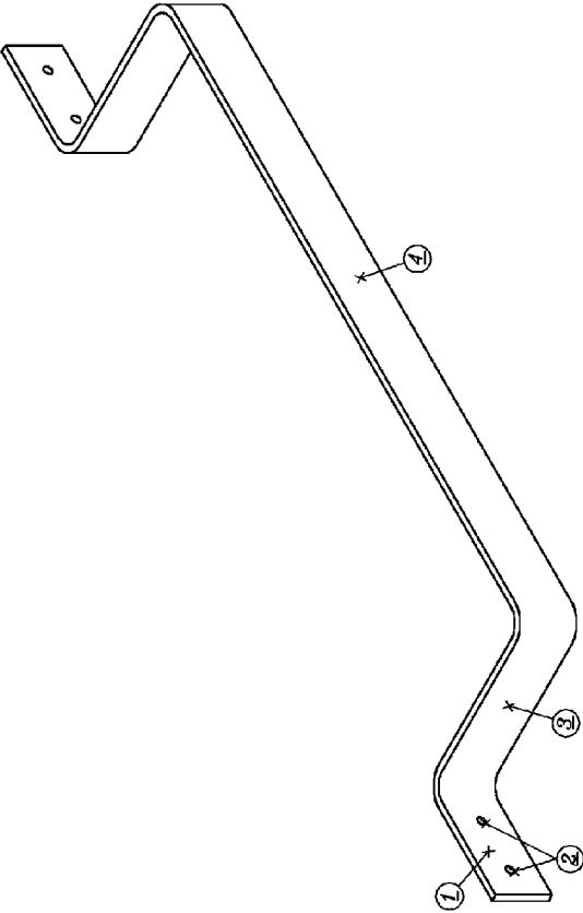
FIG. 1 WORK SAFE SINGLE FULL WRAP LADDER BRACKET
