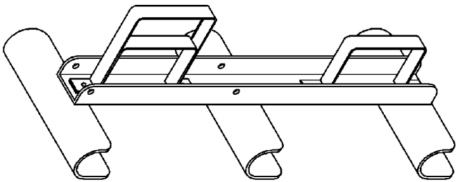
FIG. 20A ISOMETRIC NOT TO SCALE
