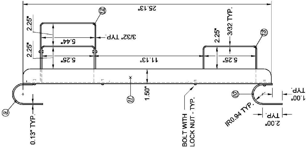
FIG. 10C. SIDE
