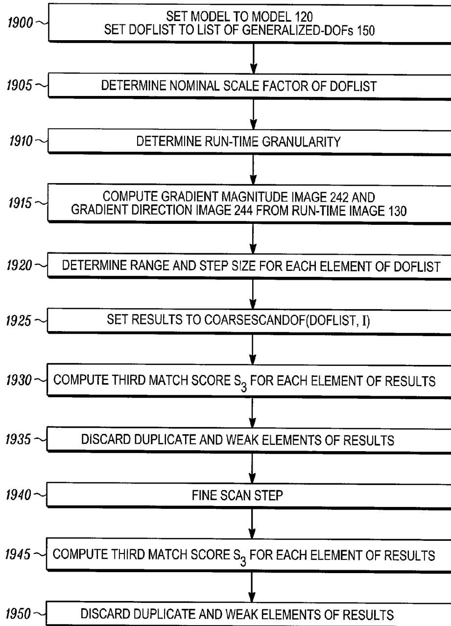
FLOW CHART OF RUN-TIME STEP 140
