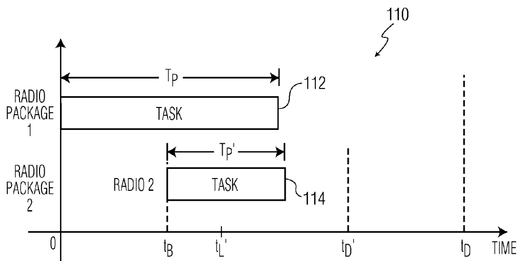
FIG. 3 PRIOR ART
