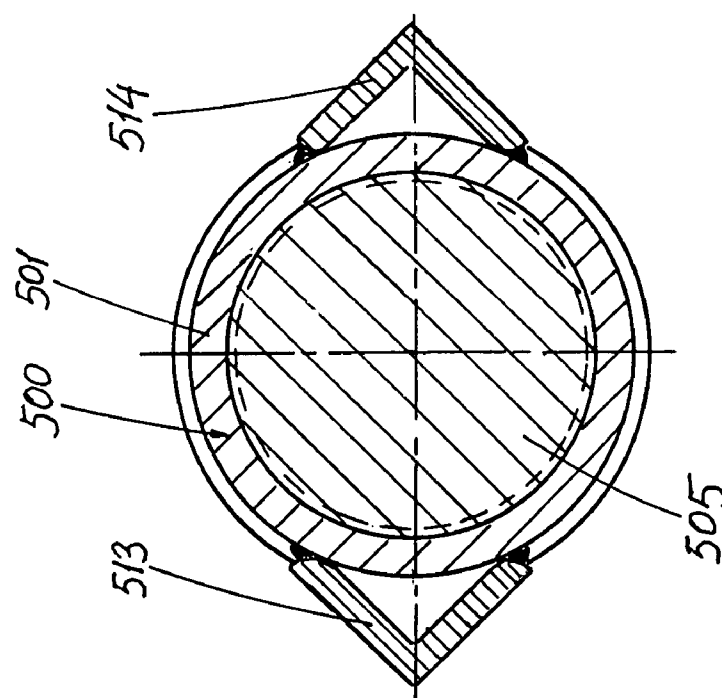
SECTION 5-5
