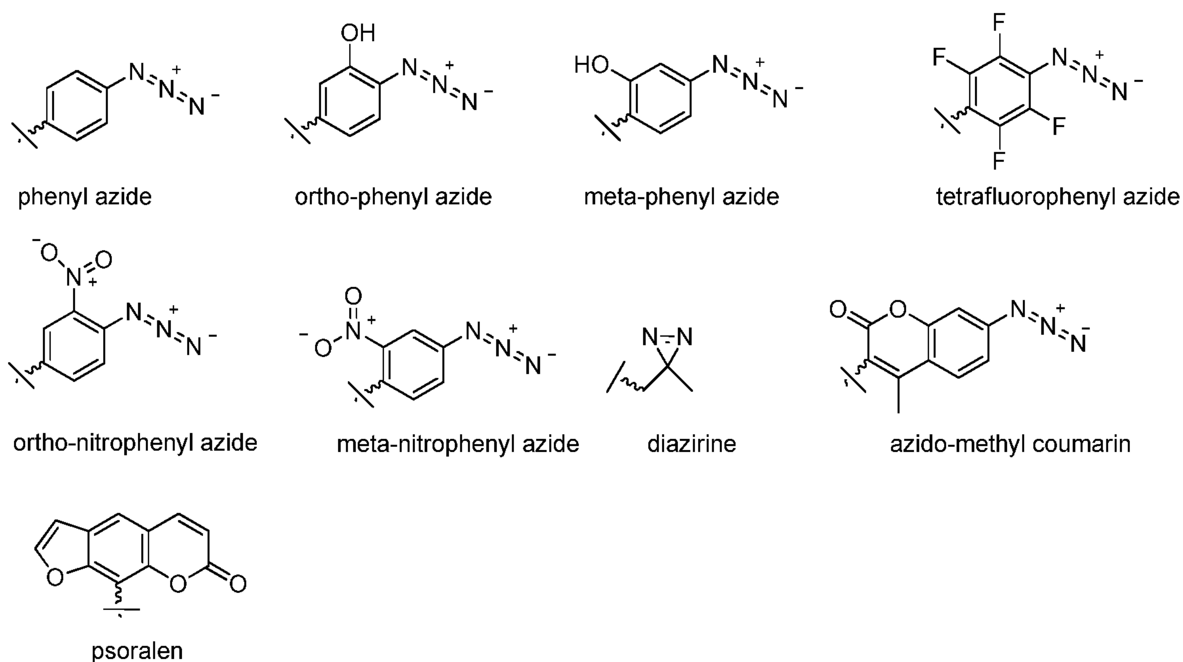
Scheme 2
