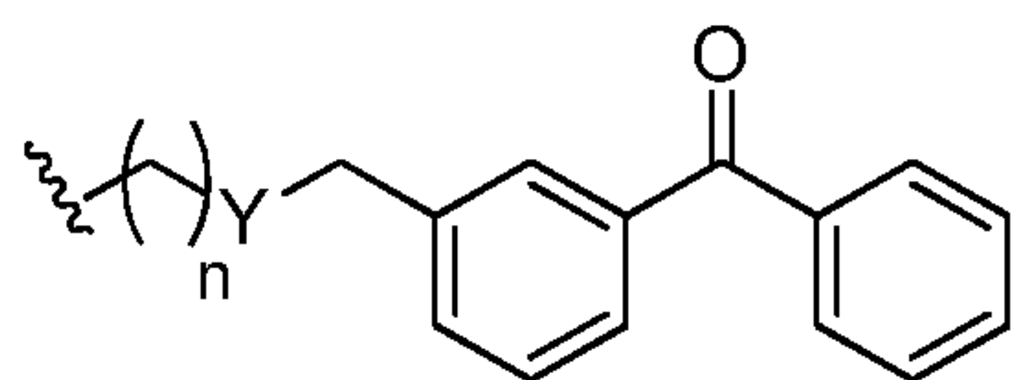
Formula (IX)
