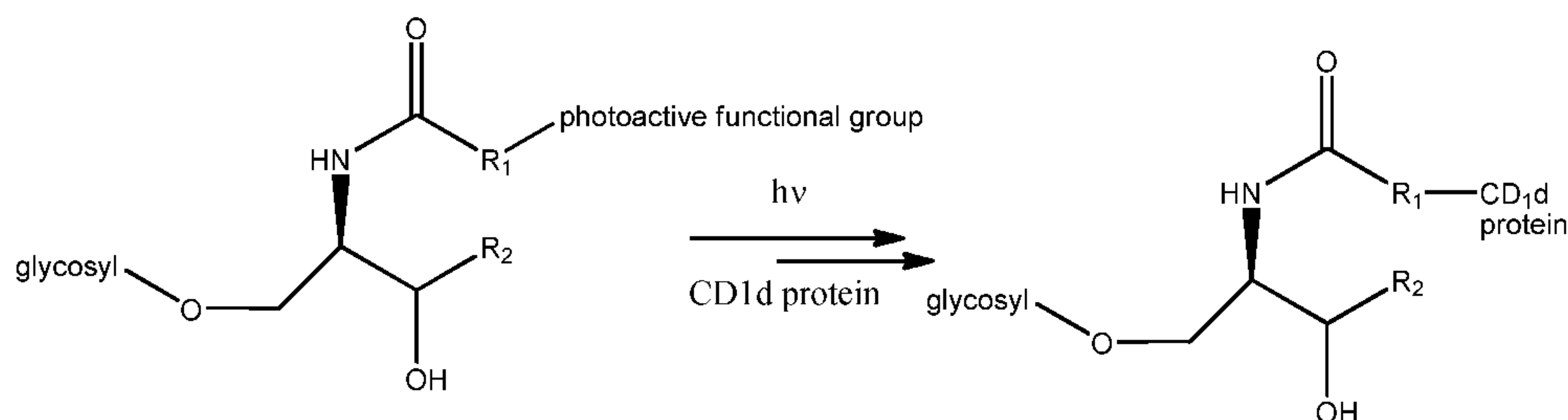
Scheme 1
