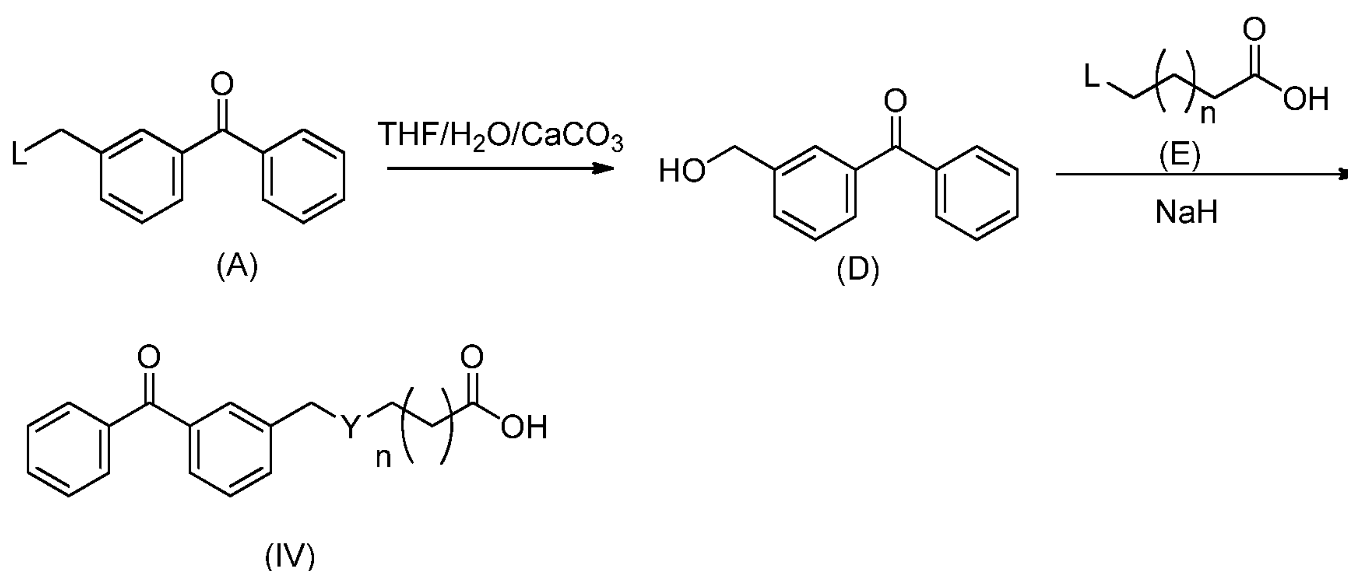
Scheme 5
