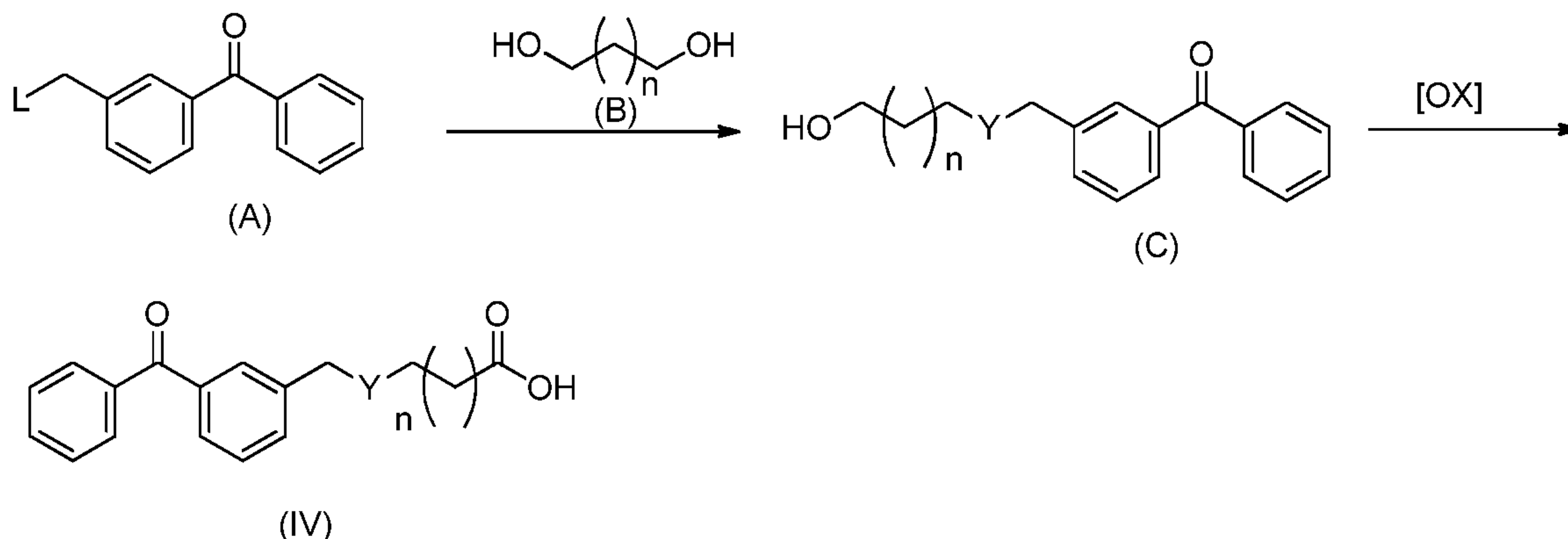
Scheme 4
