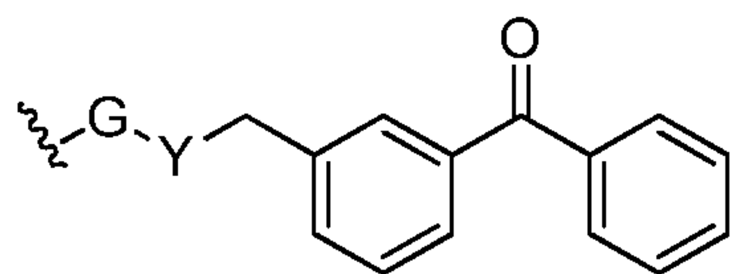
Formula (VIII)
