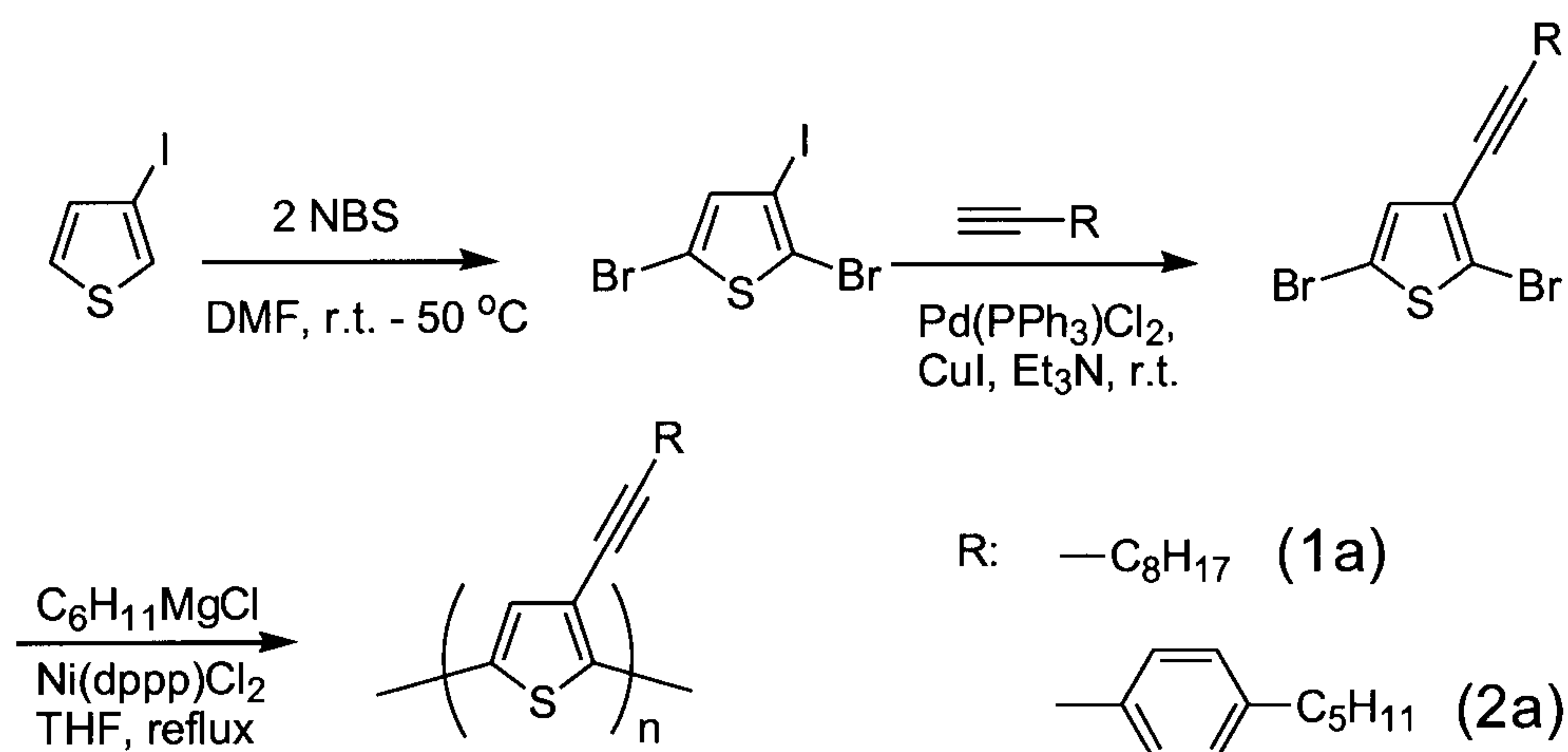
Scheme 1 - Synthesis of Poly(3-alkynyl thiophene)
