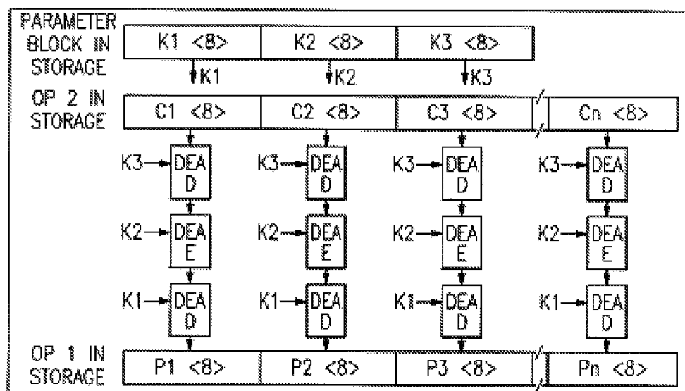
FIG.17 Prior Art
