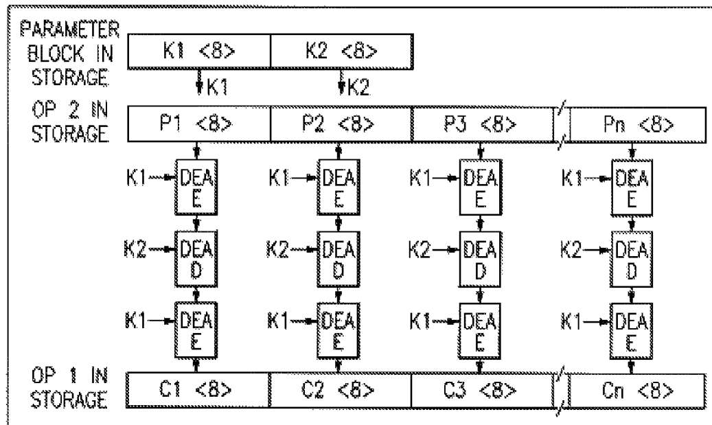
FIG.13 Prior Art
