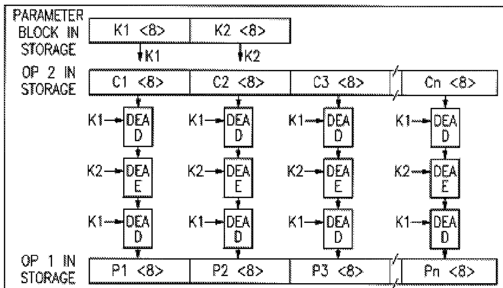
FIG.14 Prior Art
