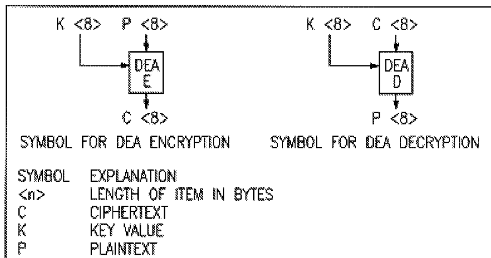
FIG. 7 Prior Art
