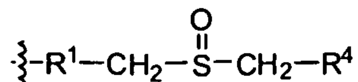
Structure III
