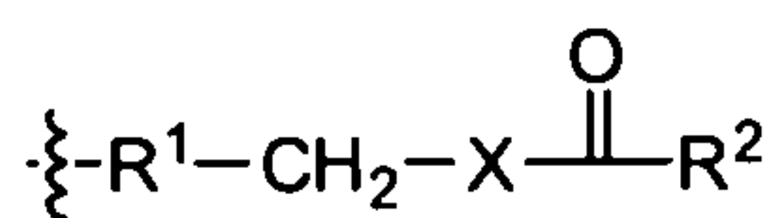
Structure I
