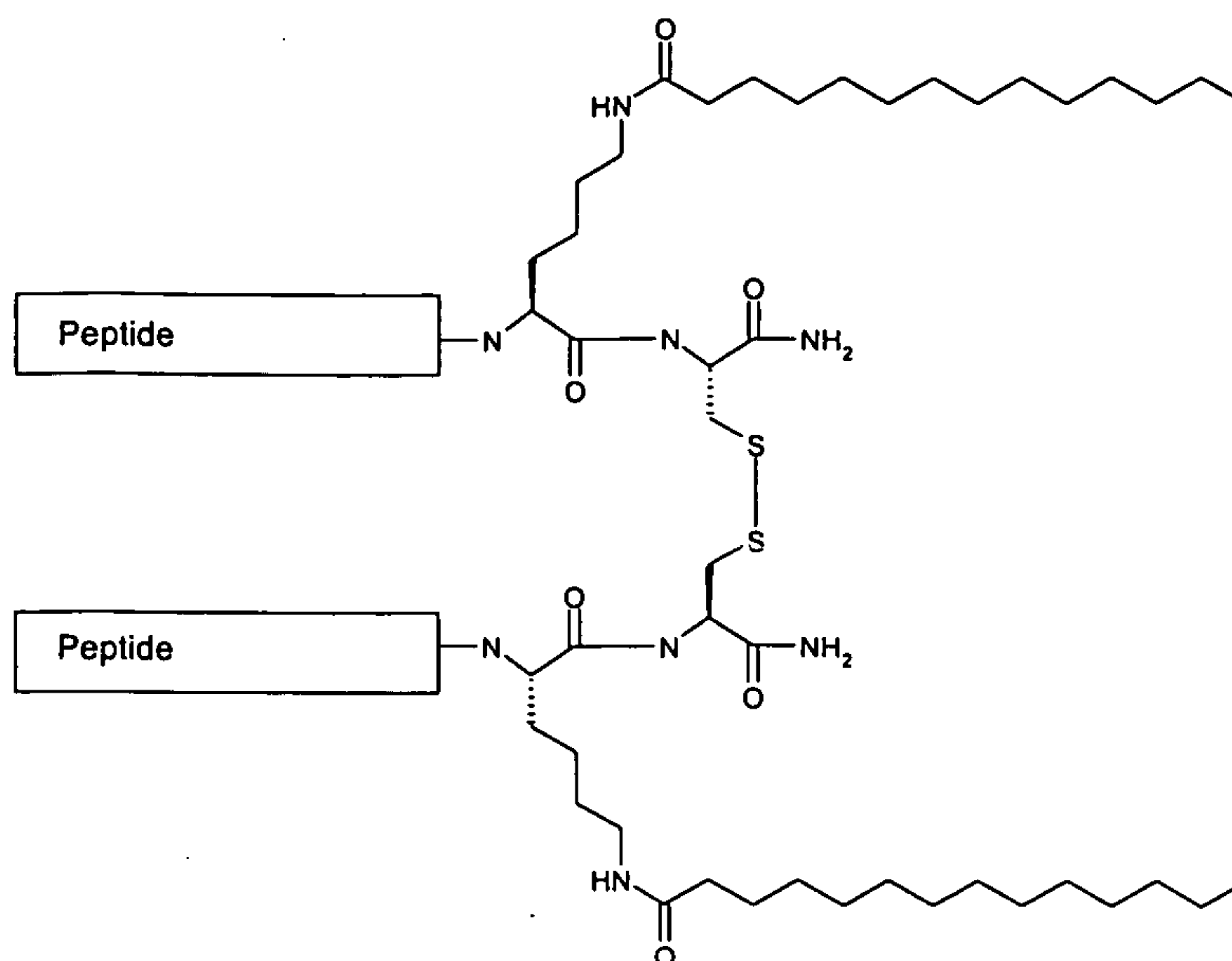
Disulfide dimer
