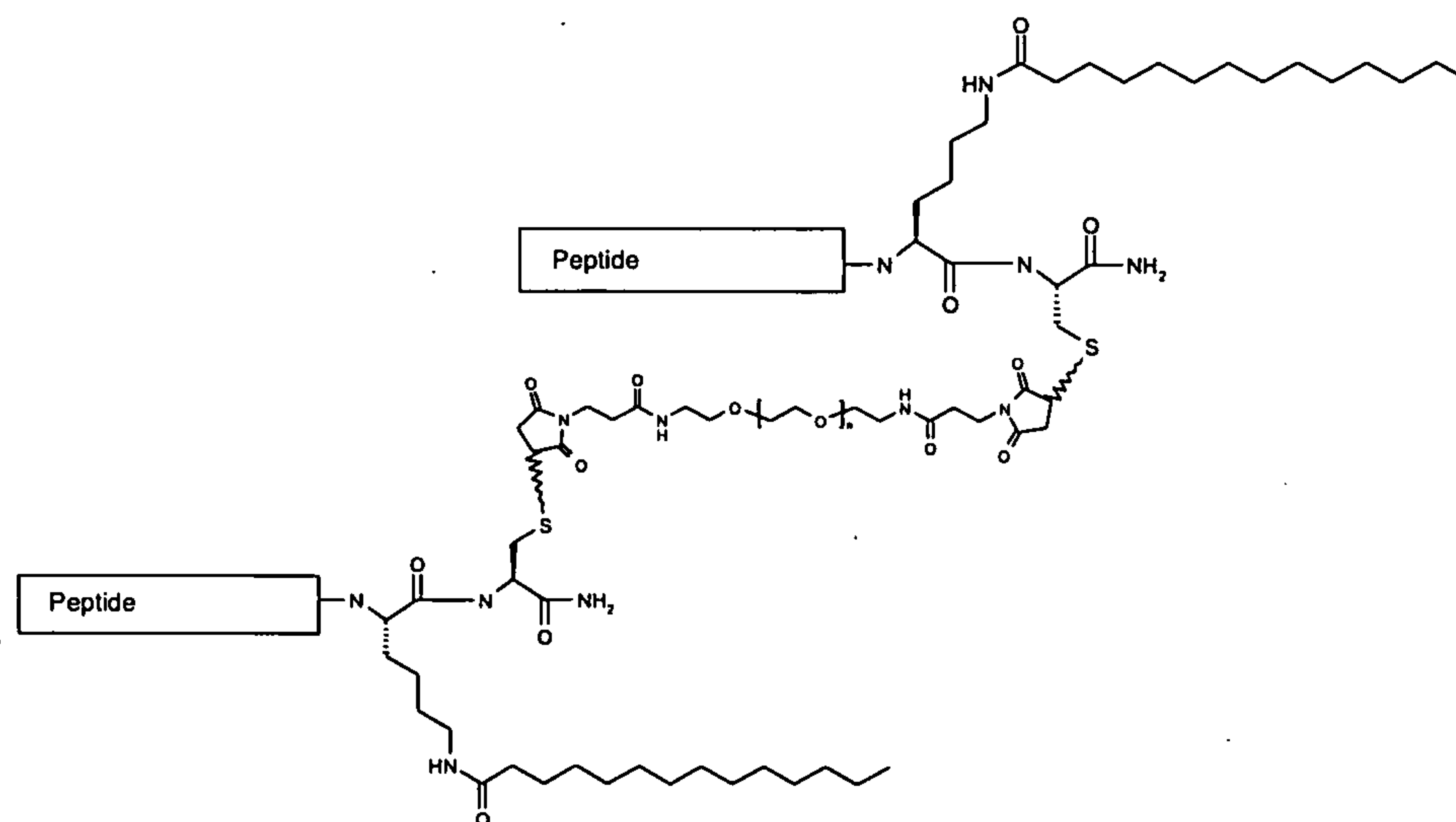
Structure B
