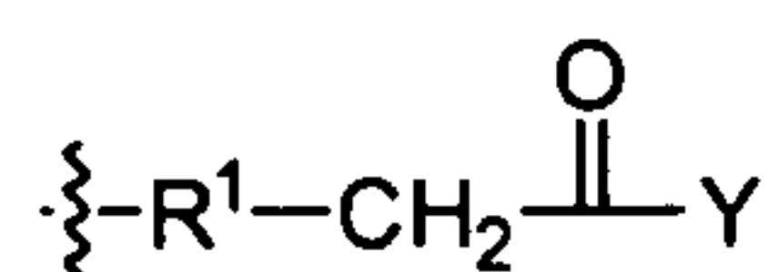
Structure II
