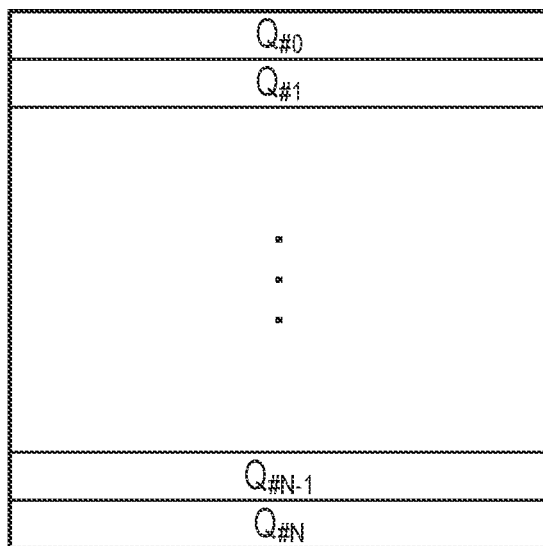
SECOND QUANTIZATION METHOD
