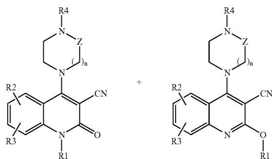
Reaction Scheme 6
